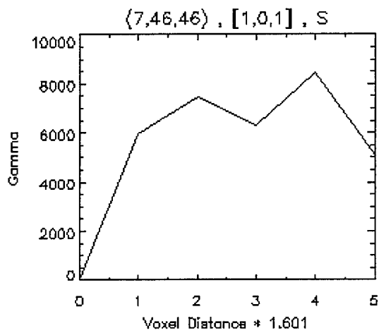
Figure 4-10. Discrete Directional Variograms
