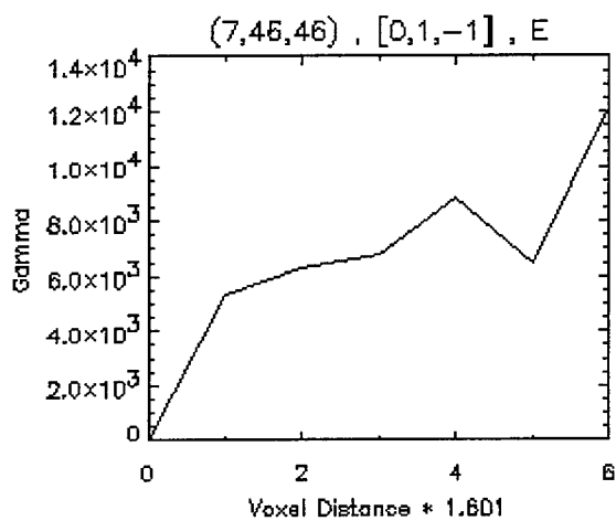
Figure 4-10. Discrete Directional Variograms
