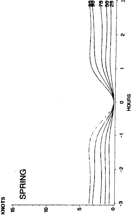
F-5 Temporal correlation of wind speed, arctic climate, sunrise.
