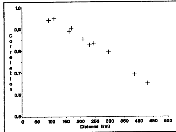
Figure 10. Correlation of temperature between Patrick AFB and neighboring synoptic stations.
