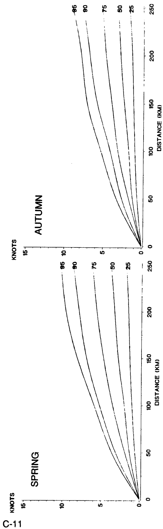
C-10 Spatial correlation of wind speed, maritime climate, midnight.
