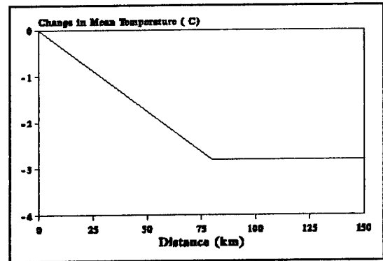
Figure 18. Modeled change in mean temperature as a function of distance inland during winter at sunrise.
