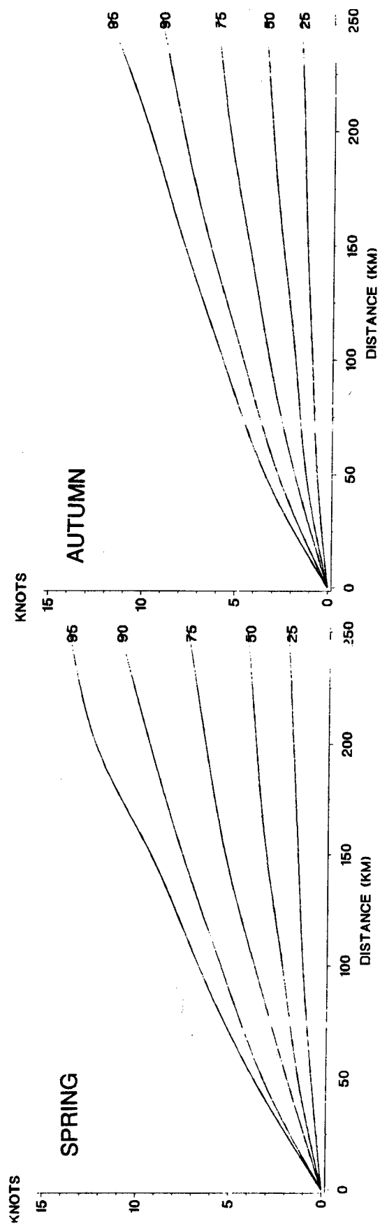
C-3 Spatial correlation of wind speed, continental climate, noon.
