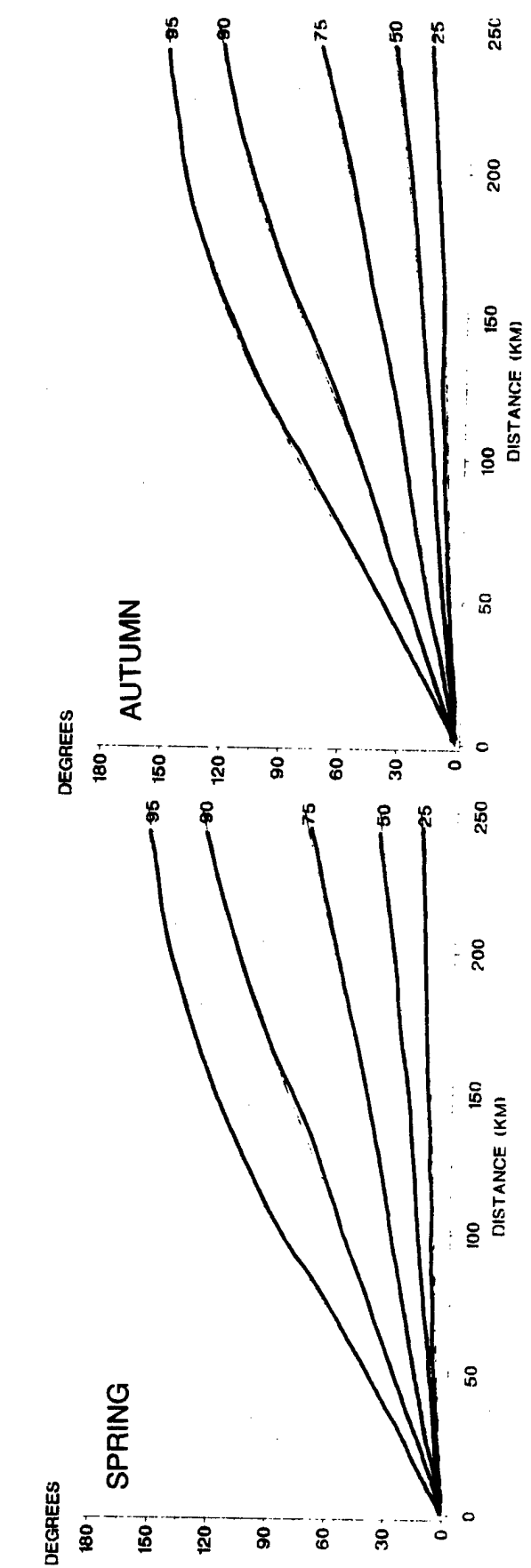
B-6 Spatial correlation of wind direction, arctic climate, noon.
