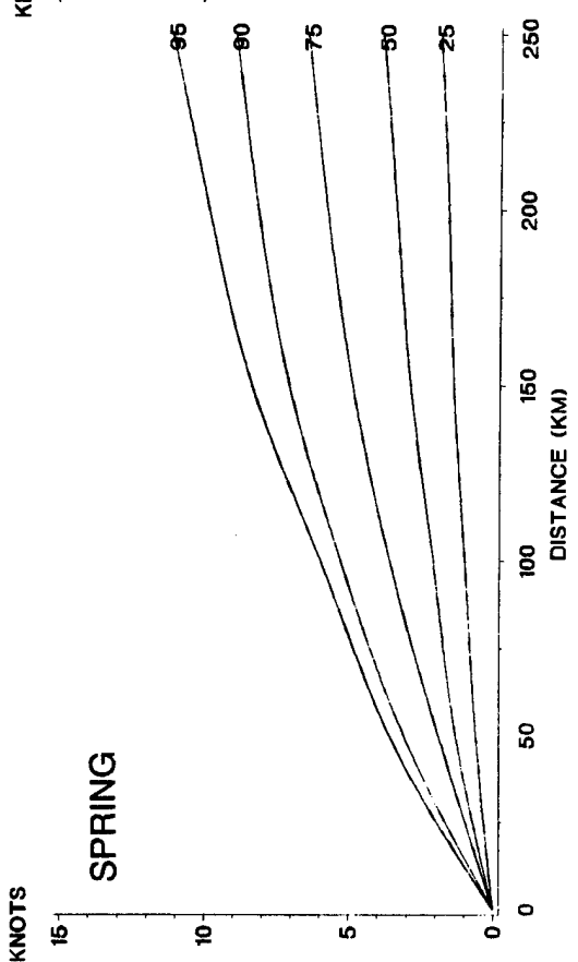
C-12 Spatial correlation of wind speed, maritime climate, noon.
