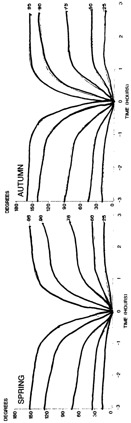
E-7 Temporal correlation of wind direction, desert climate, midnight.
