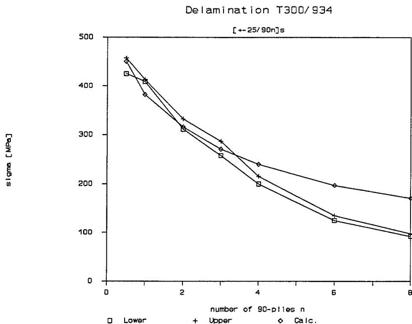
Figure 4 Delamination stress of [±25/90 n ] s T300/934. Lower-Upper: Experimental range.
