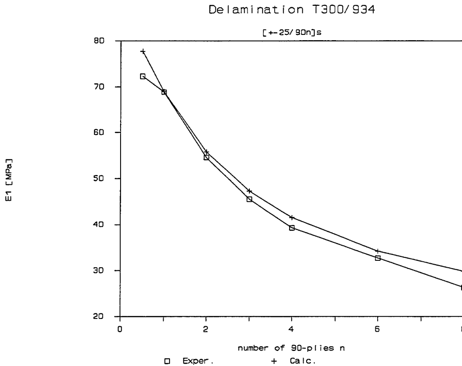
Figure 3 Tangent modulus for [±25/90 n ] s T300/934.
