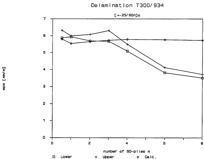
Figure 5 Delamination strain of [±25/90 n ] s T300/934. Lower-Upper: Experimental range.
