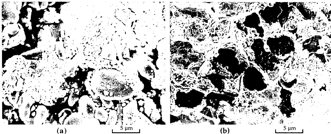
Fig. 4 - Fracture surfaces of Pb-40% Al 2 O 3 green compacts formed by static pressure of 414MPa (left) or 10 5 cycles of 0-414MPa (right) [from paper 3].
