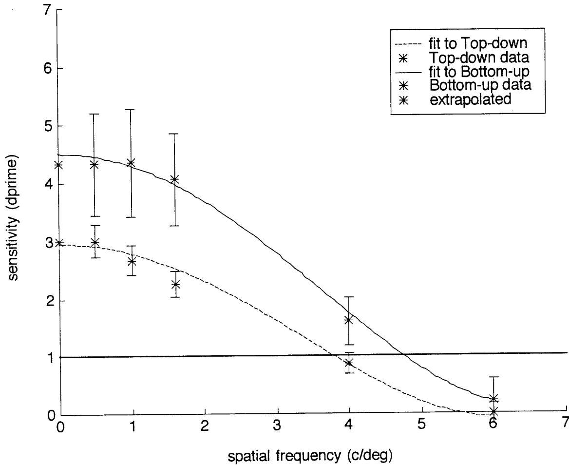
Attention MTF, Top-down and Bottom-up, subject EB
