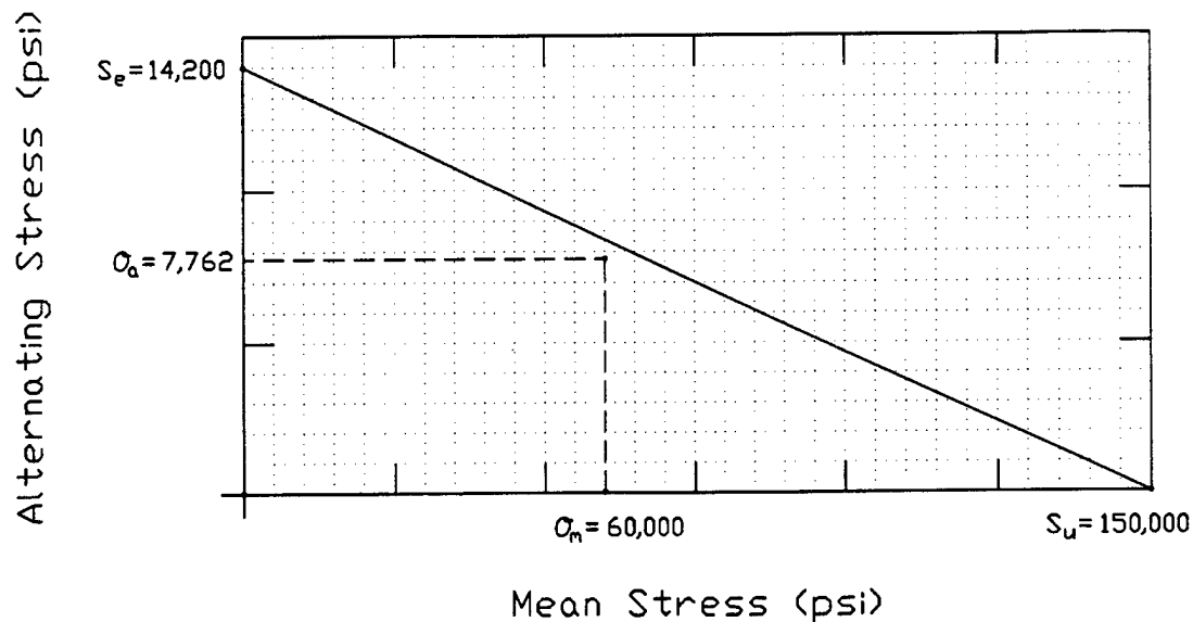
Figure 5. Fatigue diagram for the stop bolt.
