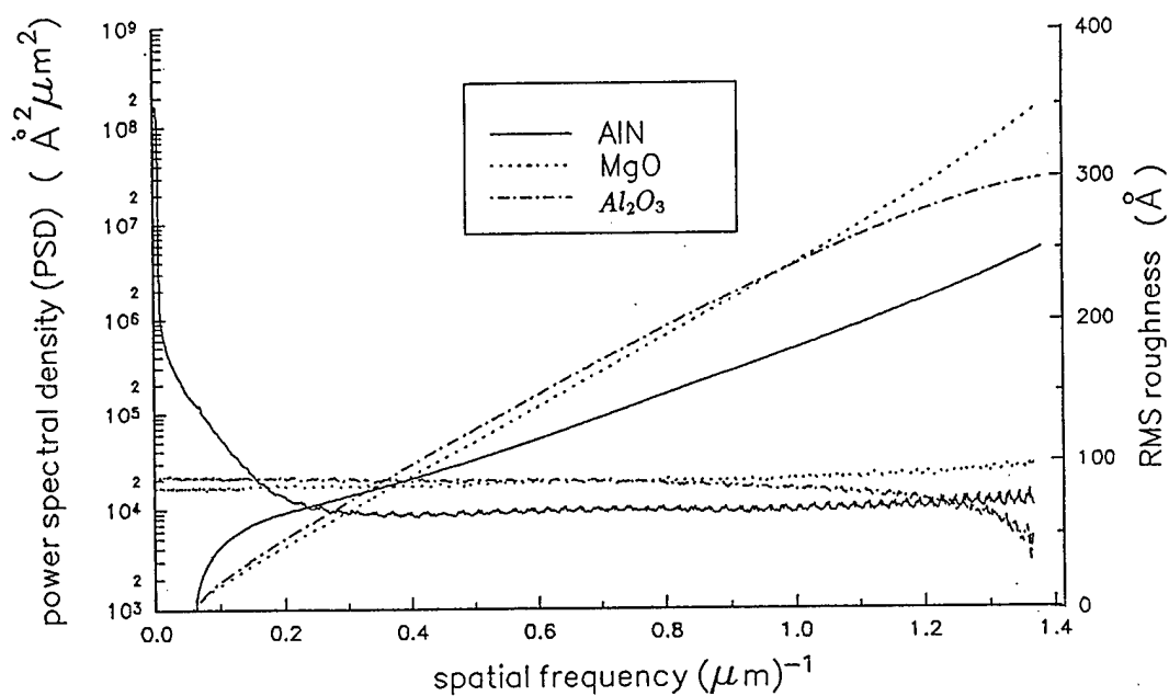
Figure 8: Scatterometry spectra comparing various polycrystalline ceramic substrate materials, \lambda = 632.8nm .
