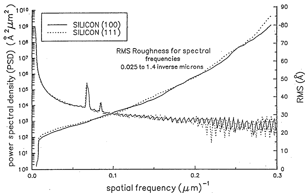
Figure 7: Scatterometry spectra of highly polished electronic grade silicon wafers (substrates), \lambda = 632.8nm .
