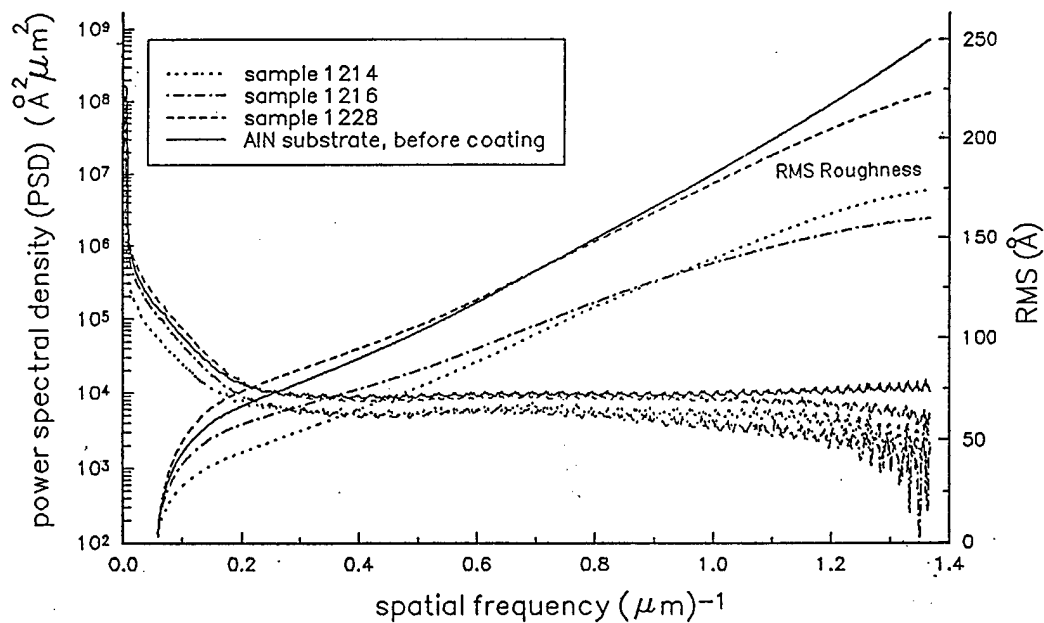
Figure 6: Scatterometry spectra of as-deposited polycrystalline \text{AlN} thin films, \lambda = 632.8\text{nm} .
