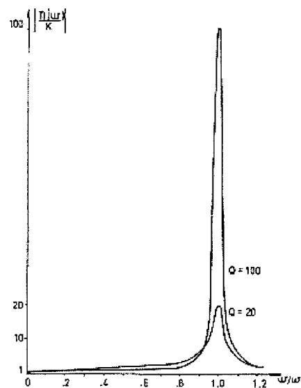
Figure 3-2 - Comparison of Different Q 's. Measured from the half-power points (0.707 x peak), the Q of a circuit is a measure of bandwidth. Here, the amplitude of response is much greater for the higher Q circuit compared with the lower Q circuit [10].
