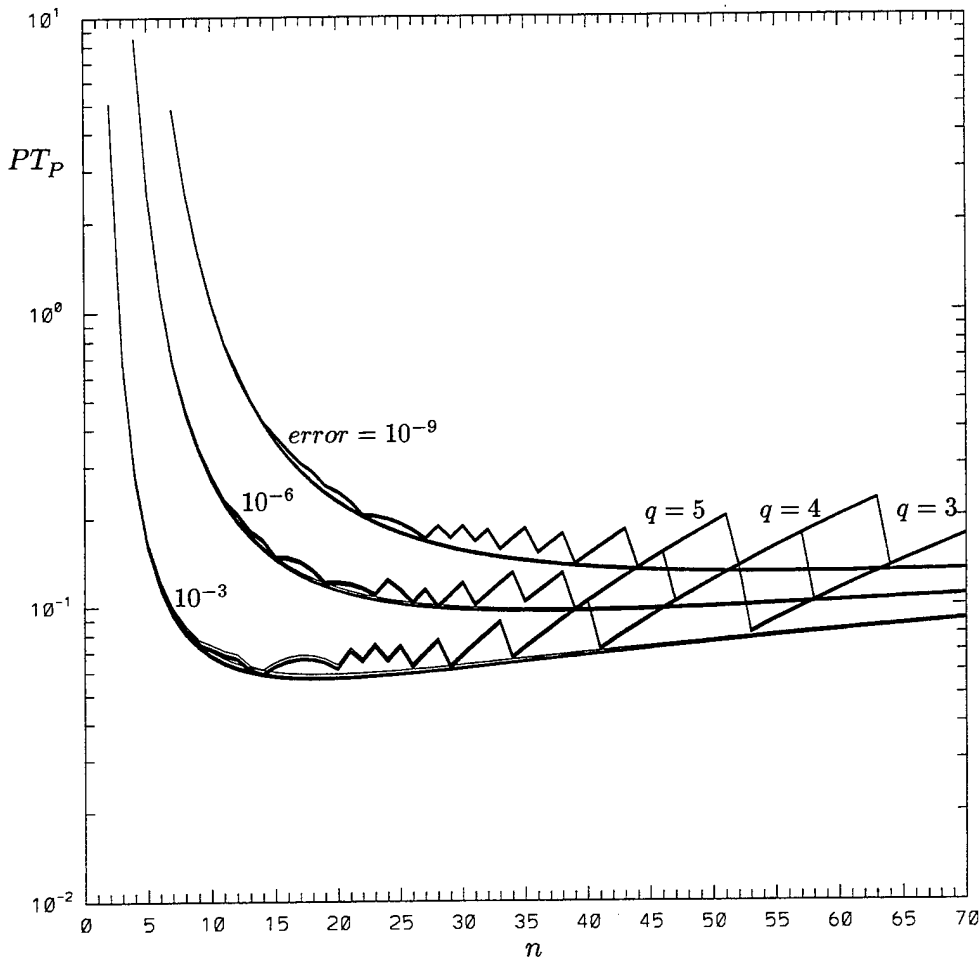
Figure 1: Normalized time per step for two-dimensional problem with \alpha = 0 .
