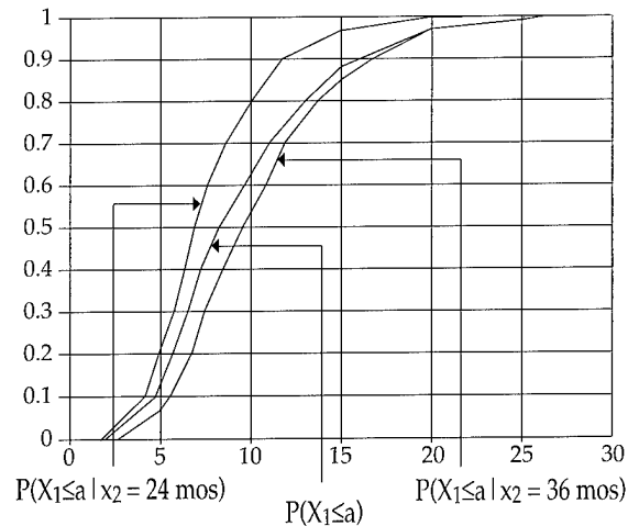
Figure 5. A Family of Conditional LogNormal Cost Distributions Ada Cost-Schedule Model Example
