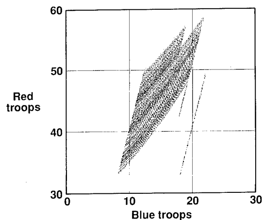
FIGURE 8 Phase Space Attractor
