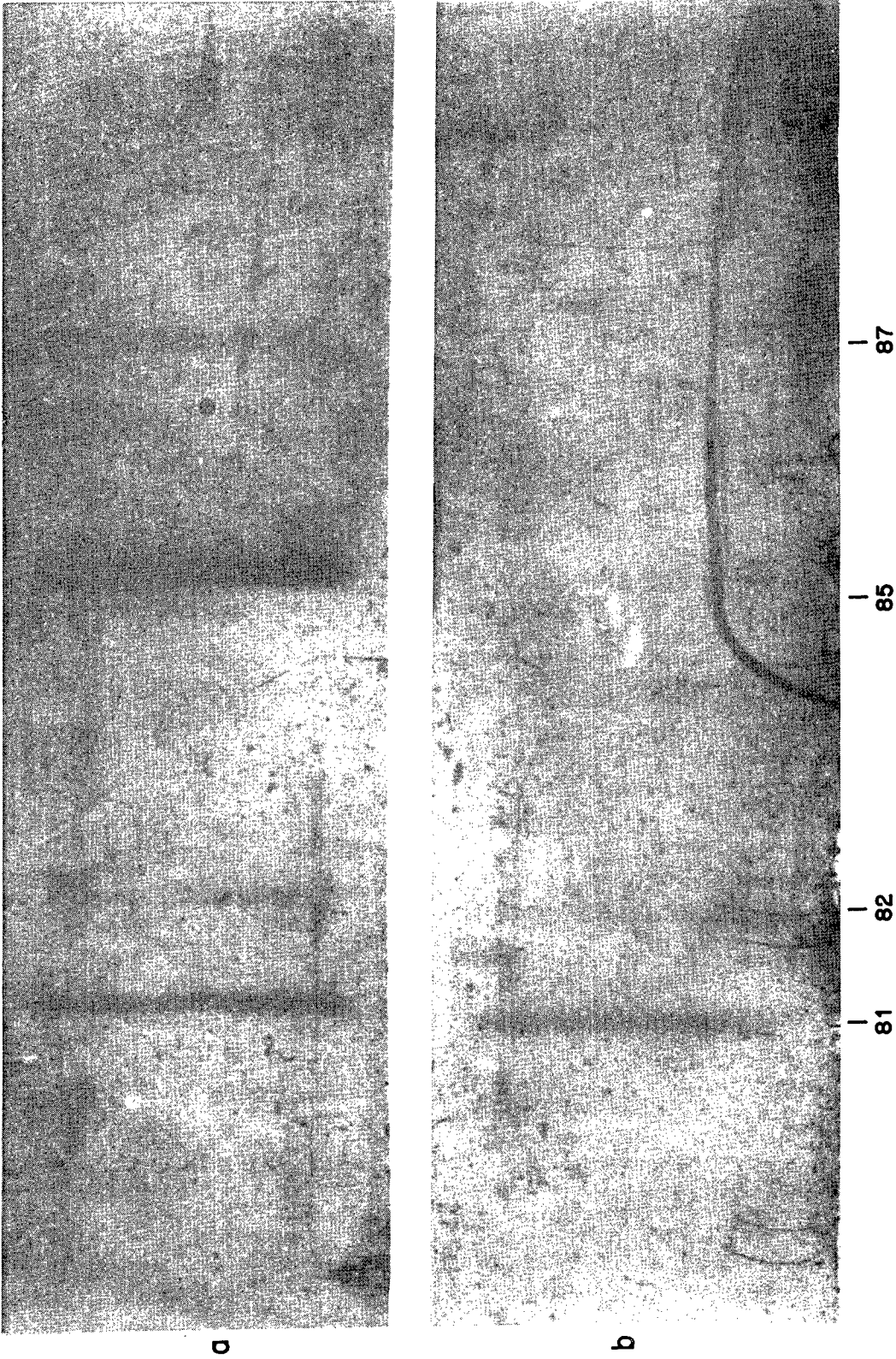
Figure 1. The original plate shows stable Rb 85 and radioactive Rb 87 and radioactive Rb 81 and Rb 82 . The "transfer" plate is placed emulsion-to-emulsion with the original for several hours before either is developed, to locate radioactive material.
