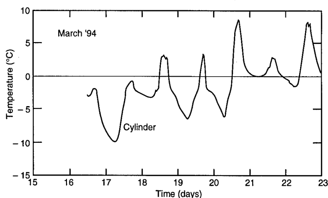
Figure 15. Temperature history of the center of mass of a 75- x 150-mm (3 x 6 in.) cylinder of EY11L concrete stored on grade in the unheated shelter at Sault Ste. Marie, Michigan.
