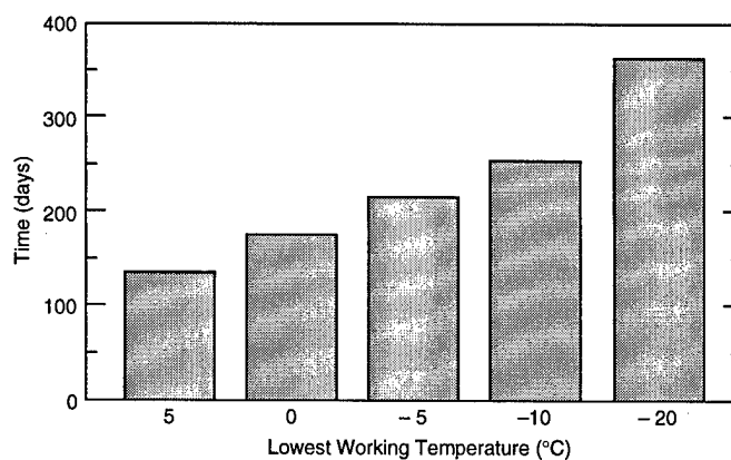
Figure 16. Possible extension of construction season with various low-temperature limits (Horrigan 1995, unpublished).
