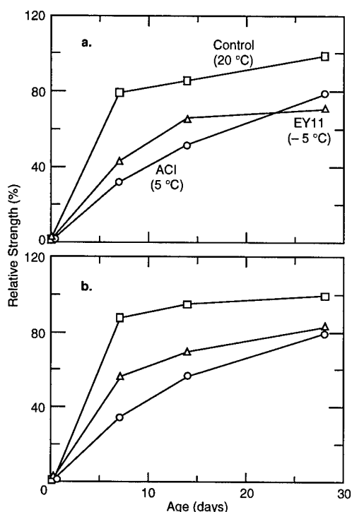
Figure 6. Strength gain of concrete made with EY-11 cured at -5^{\circ}\text{C} ( 23^{\circ}\text{F} ) compared to control concrete cured at two above-freezing temperatures. The line denoted as ACI ( 5^{\circ}\text{C} ) is based on guidance provided by ACI (1988). That line represents the minimum curing condition used by the construction industry today. Figure 6a is for concrete containing a 365\text{-kg/m}^3 ( 611\text{ lb/yd}^3 ) cement factor and a 100\text{-mL/kg} ( 150\text{ fl oz/cwt} ) EY-11 dosage. Figure 6b contains a 420\text{-kg/m}^3 ( 705\text{ lb/yd}^3 ) cement factor and a 100\text{-mL/kg} ( 150\text{ fl oz/cwt} ) EY-11 dosage.
