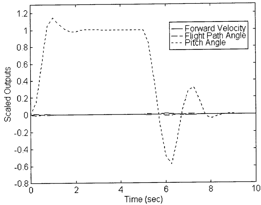
Figure 4.53 PP Output Resp. (Failures: SS at t=0.5 ; AS at t=1.0 )
