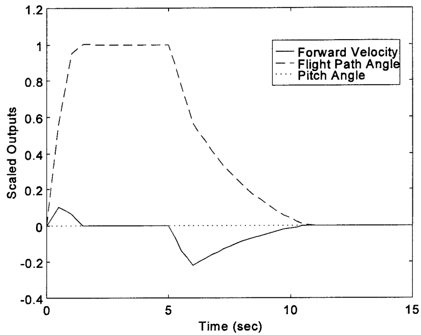
Figure 4.21 VT Output Resp. (Failures: SS at t=0 ; TES at t=0.5 )
