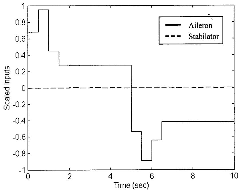
Figure 4.28 VT Control Defl. (Failures: SS and TVS at t=0 )
