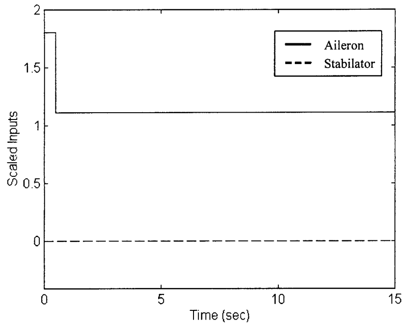
Figure 4.36 Controls (Failures: SS at t=0 ; LES at t=0.5 ; AS at t=1.0 )
