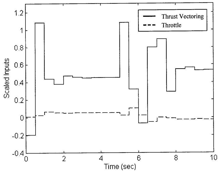
Figure 4.54 PP Control Defl. (Failures: SS at t=0.5 ; AS at t=1.0 )
