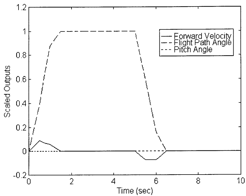
Figure 4.25 VT Output Resp. (Failures: SS and TVS at t=0 )
