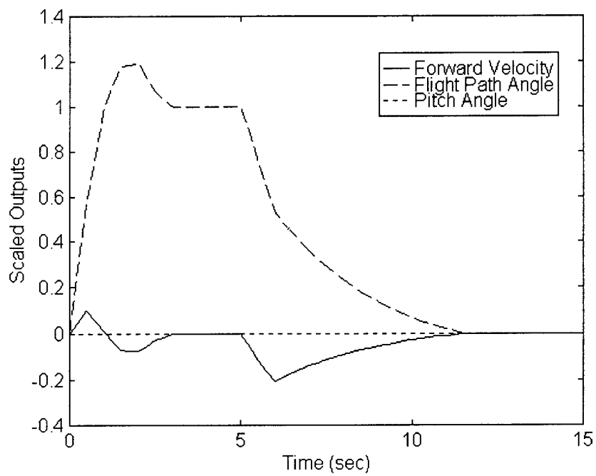
Figure 4.33 Outputs (Failures: SS at t=0 ; LES at t=0.5 ; AS at t=1.0 )
