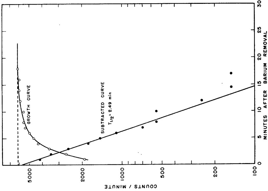
Figure 2. Growth of Ba^{137} \gamma activity in Cs^{137} .
