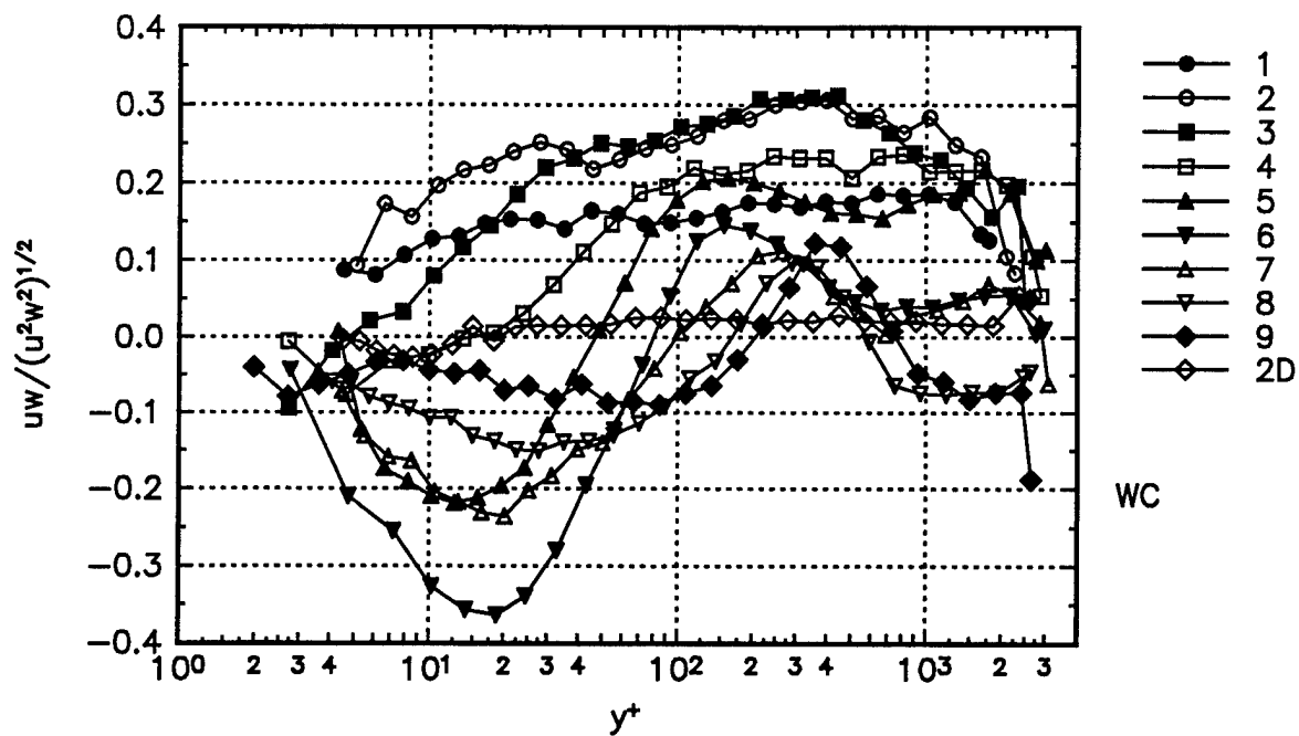
Figure 11. The \overline{uw}/(\overline{u^2 w^2})^{1/2} shear stress correlation coefficient in wall-stress coordinates. The uncertainties are on the order of the symbol size.
