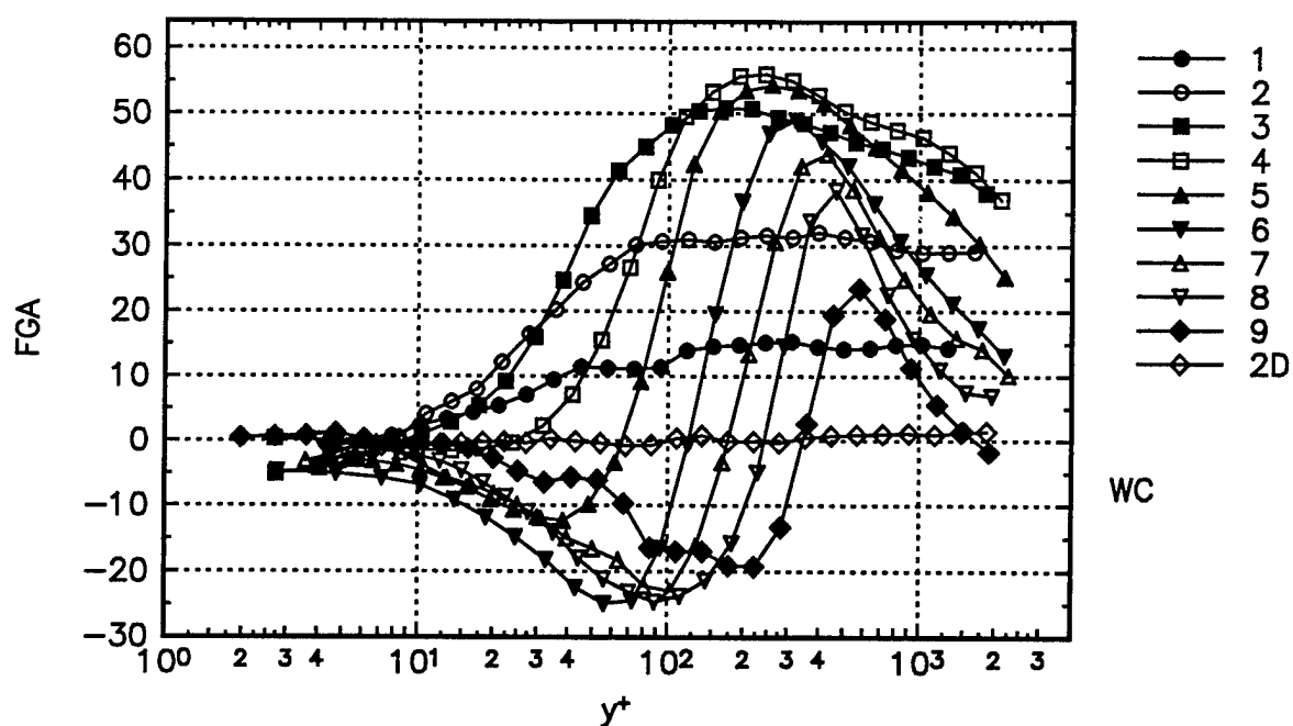
Figure 6b. Flow gradient angle calculated in wall-stress coordinates. The uncertainties are on the order of the symbol size.
