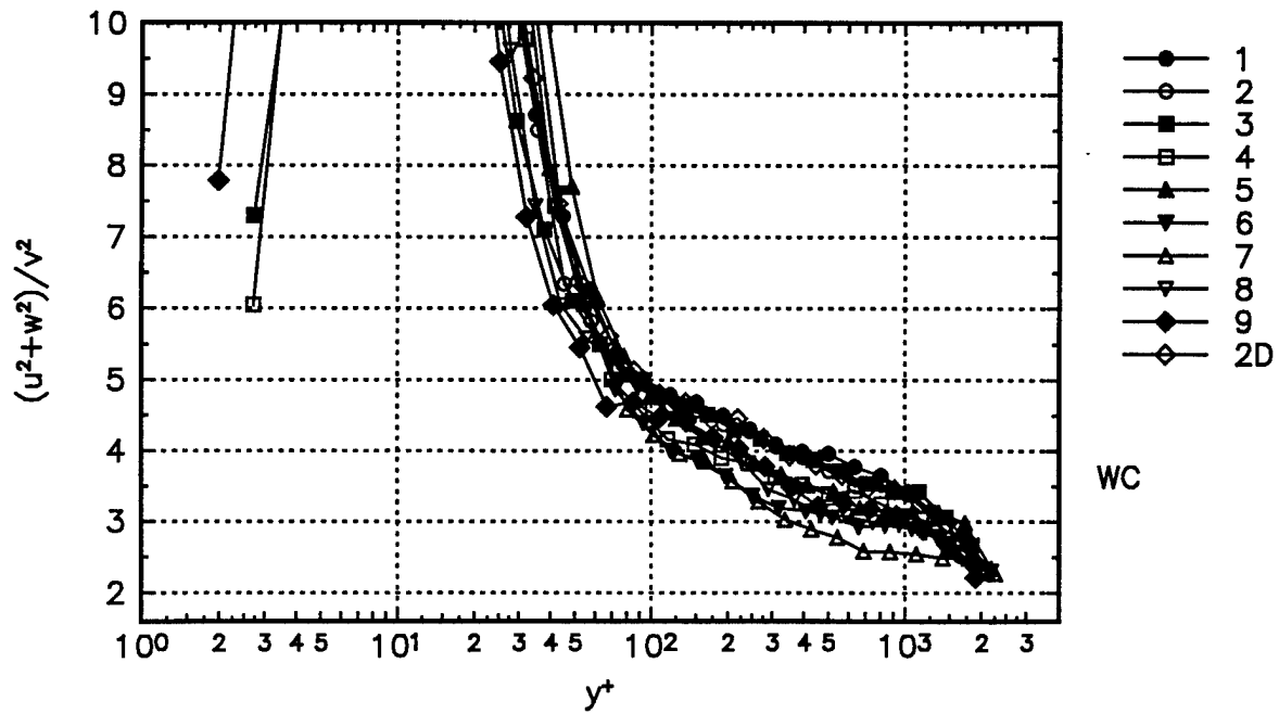
Figure 30. The (\overline{u^2}+\overline{w^2})/\overline{v^2} structural parameter calculated in wall-stress coordinates. The uncertainties are on the order of the symbol size.
