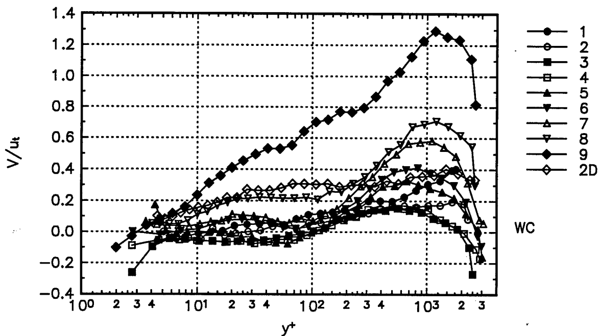
Figure 4. V/u_t , mean velocity component in wall-stress coordinates. The uncertainties are on the order of the symbol size.
