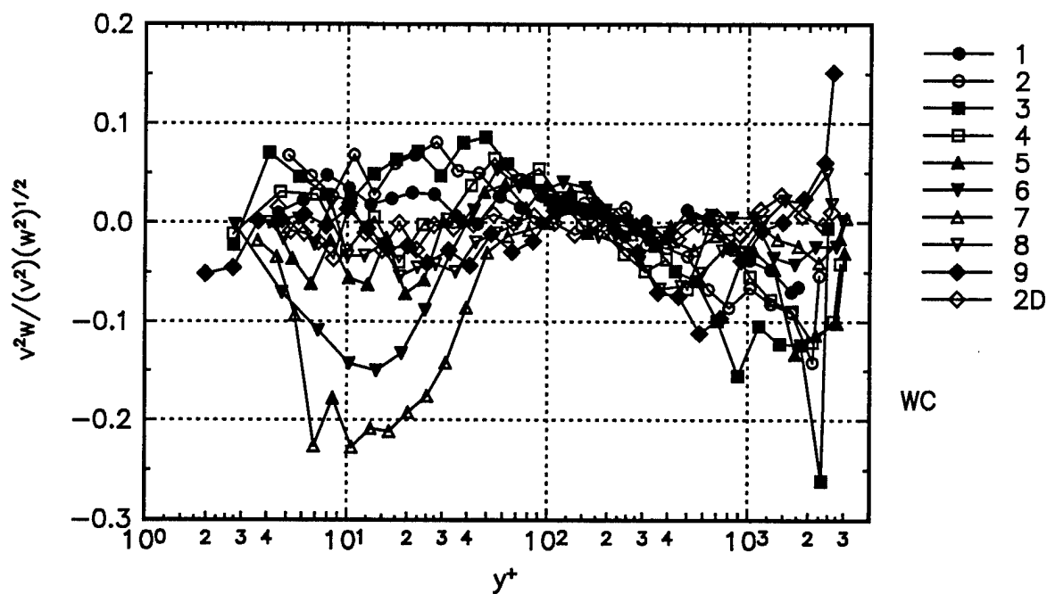
Figure 17. The \overline{v^2 w} / (\overline{v^2})^{1/2} (\overline{w^2})^{1/2} triple product correlation coefficient in wall-stress coordinates. Typical uncertainty is \pm 0.011 .
