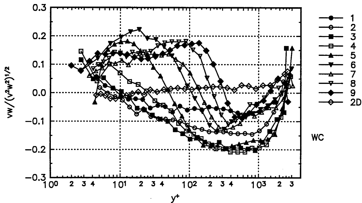
Figure 12. The \overline{vw}/(\overline{v^2 w^2})^{1/2} shear stress correlation coefficient in wall-stress coordinates. The uncertainties are on the order of the symbol size.
