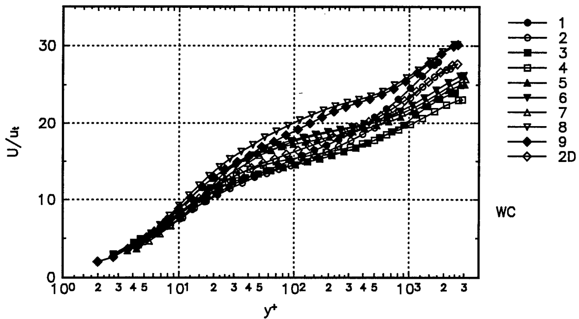
Figure 2. U/u_{\tau} , mean velocity component in wall-stress coordinates. The uncertainties are on the order of the symbol size.
