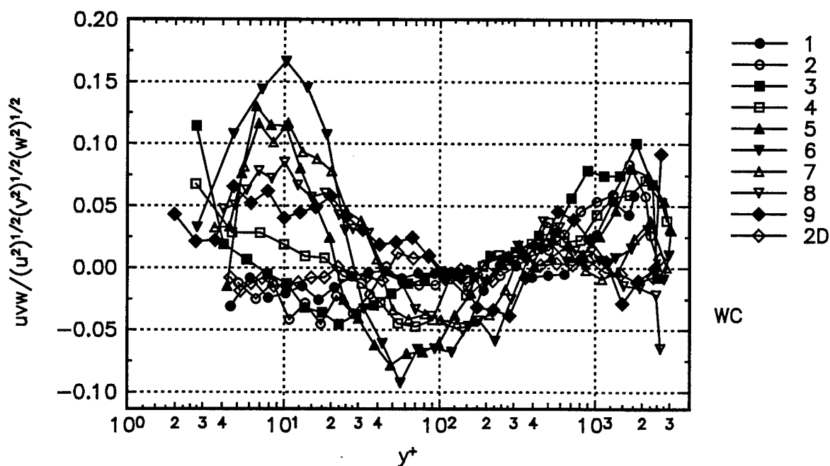
Figure 18. The \overline{uvw} / (\overline{u^2})^{1/2} (\overline{v^2})^{1/2} (\overline{w^2})^{1/2} triple product correlation coefficient in wall-stress coordinates. The uncertainties are on the order of the symbol size.
