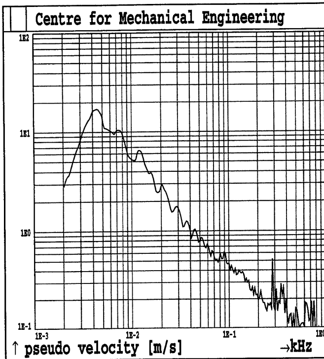
Fig.3B99. Shot 3 MAXIMAX Sensor A20
