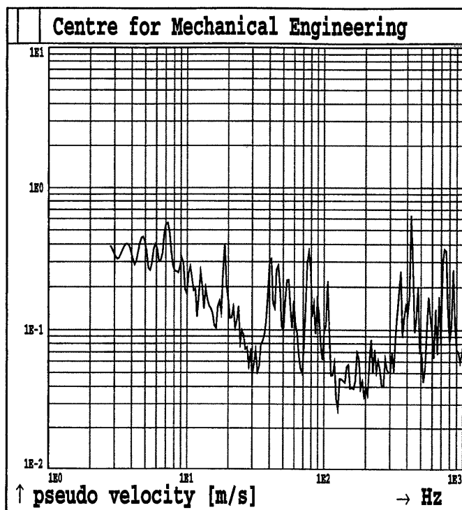
Fig.1B99. Shot 1 MAXIMAX Sensor A19
