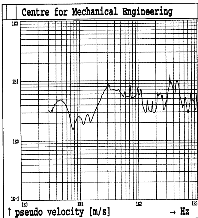
Fig.1B81. Shot 1 MAXIMAX Sensor A1
