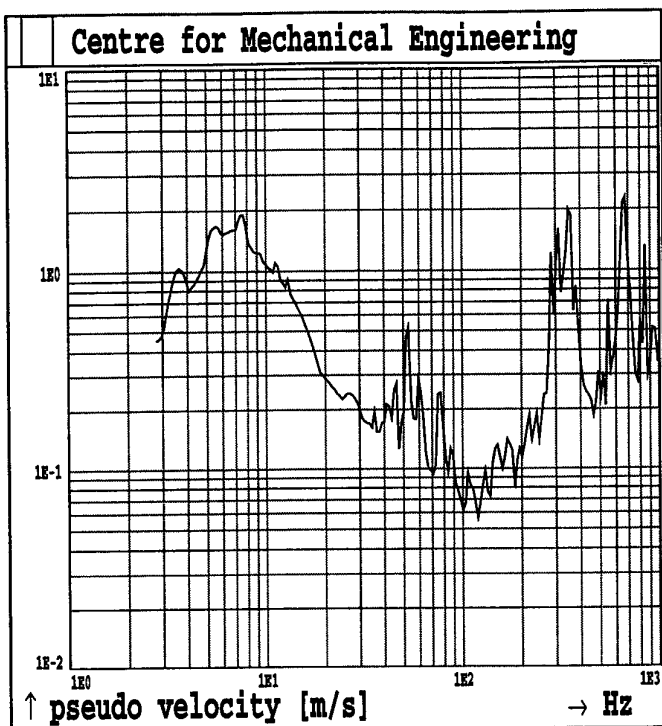
Fig.1B97. Shot 1 MAXIMAX Sensor A17
