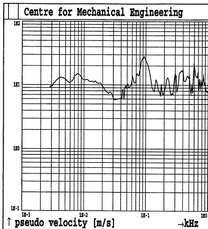
Fig.2B89. Shot 2 Sensor A9
