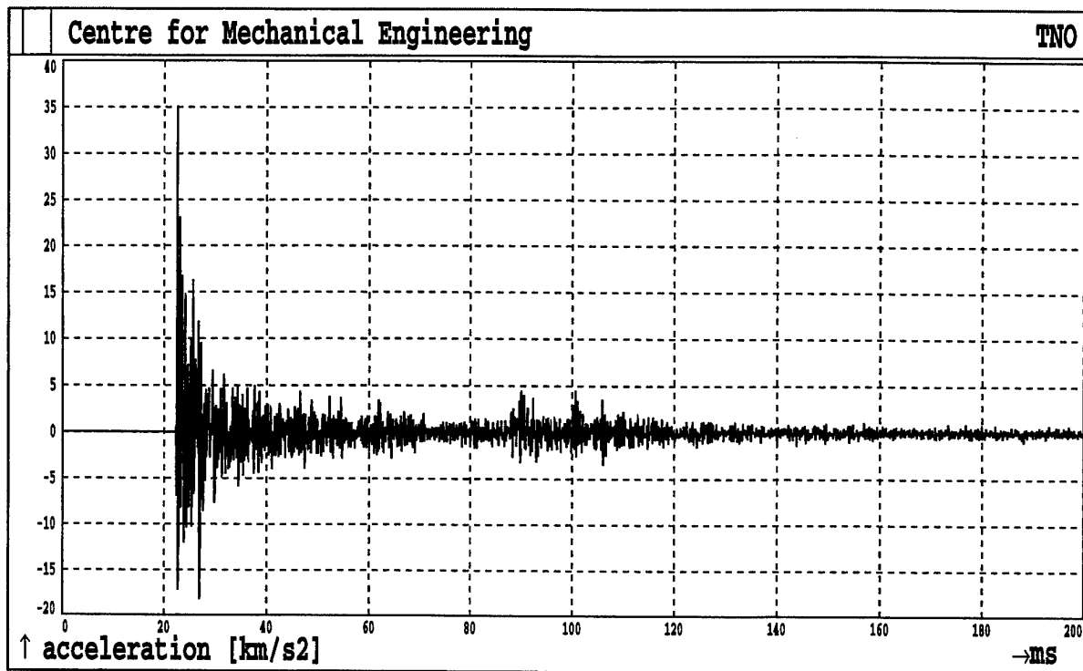
Fig.1B19. Shot 1 Sensor A11
