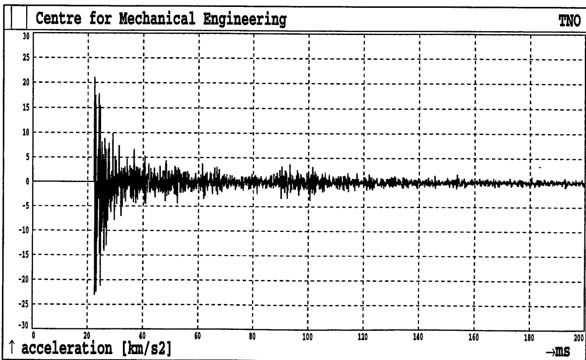
Fig.1B20. Shot 1 Sensor A12
