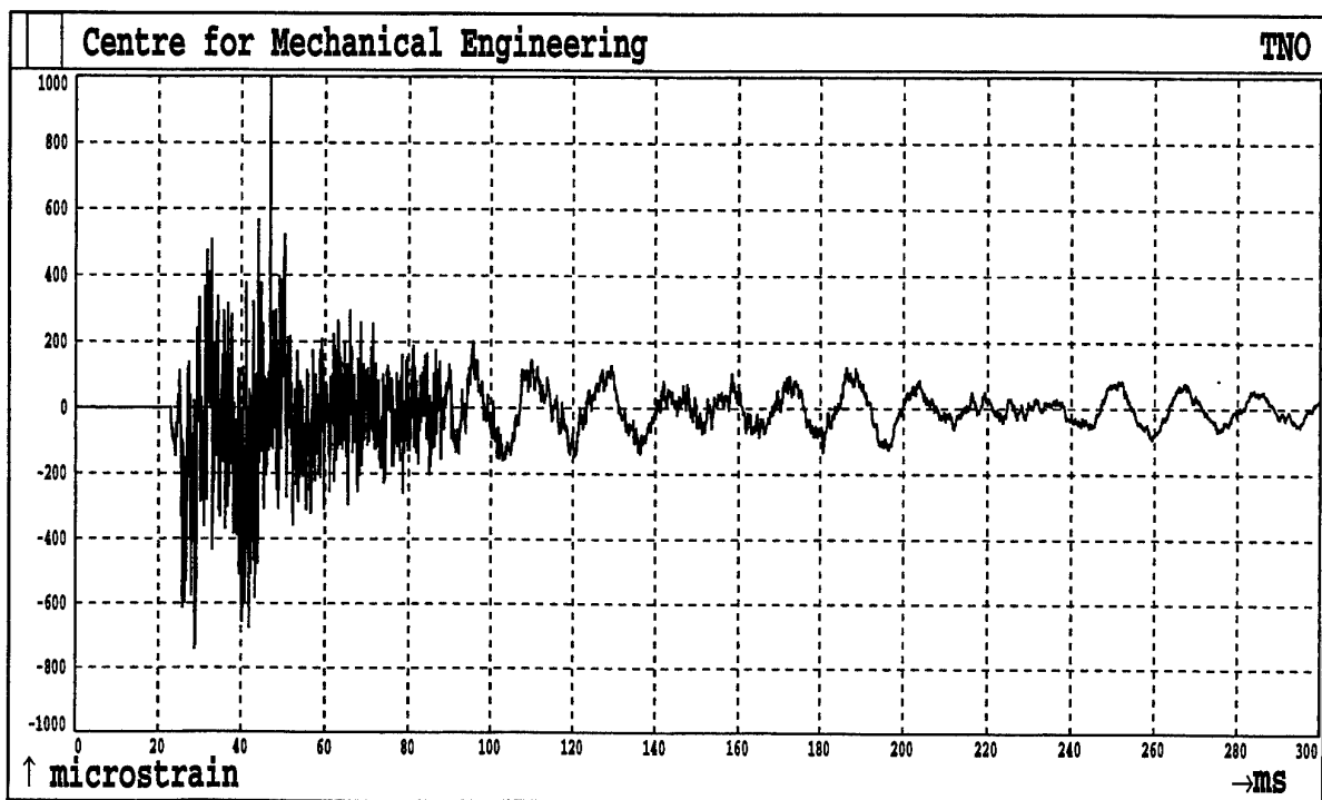
Fig.1A24. Shot 1 Sensor S25
