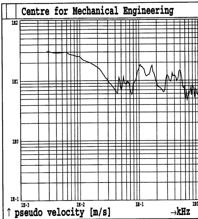
Fig.2B87. Shot 2 Sensor A7
