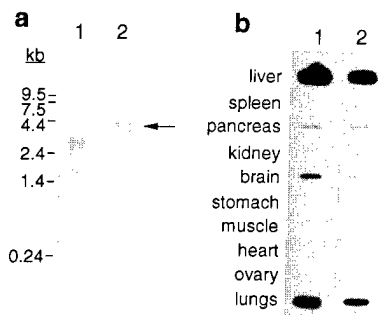
FIG. 5. Characterization and tissue distribution of saxiphilin mRNA. (a) Northern blot analysis of poly(A) + RNA from bullfrog liver. Five micrograms of poly(A) + RNA was fractionated on agarose, transferred to nylon, and consecutively hybridized with a 2.25-kb Sma I probe (lane 1) and a 0.43-kb insert-specific probe (lane 2). The arrow at the right points to the band identified as saxiphilin mRNA. (b) The same probes were hybridized to 5 \mu g of total RNA from various bullfrog tissues using a slot blot apparatus: 2.25-kb Sma I probe (lane 1); 0.43-kb insert-specific probe (lane 2).
