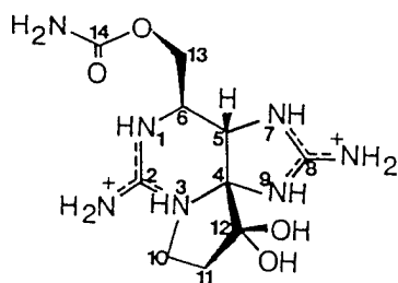
SAXITOXIN
