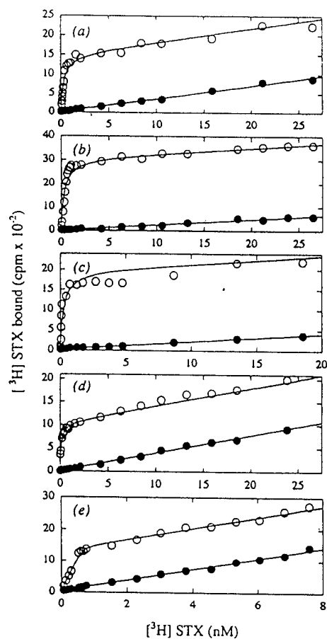
Figure 6. Saxiphilin-like activity in diverse animal species. The five panels above demonstrate the presence of saxiphilin-like activity in an amphibian, two reptiles, a fish and an arthropod. A constant amount of soluble protein extracted from various animal species was assayed for binding at the indicated concentrations of total [ ^3\text{H} ]STX, where filled circles indicate the non-specific component in the presence of excess unlabeled STX. (a) plasma from Bufo marinus , cane toad; (b) plasma from Naja naja kaouthia , Thailand cobra; (c) plasma from Thamnophis sirtalis , garter snake; (d) crude soluble extract from Gambusia affinis , mosquito fish; (e) hemolymph from Ethmostigmus rubripes , an Australian centipede. Figure taken from Llewellyn et al., 1996.
