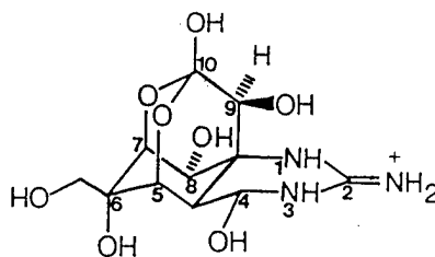
TETRODOTOXIN
