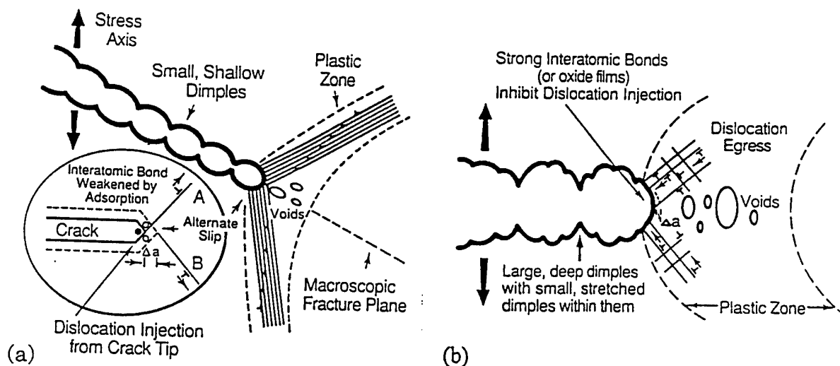
Fig.1 Schematic diagrams illustrating crack growth by (a) adsorption-induced localised-slip compared with (b) crack growth in inert environments.
