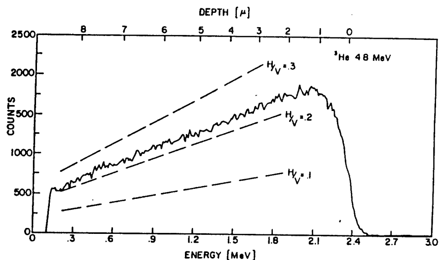
Figure 4: An ERD spectrum recorded from a sample of V electrolytically charged with hydrogen to \text{VH}_{0.23} . From reference [6].
