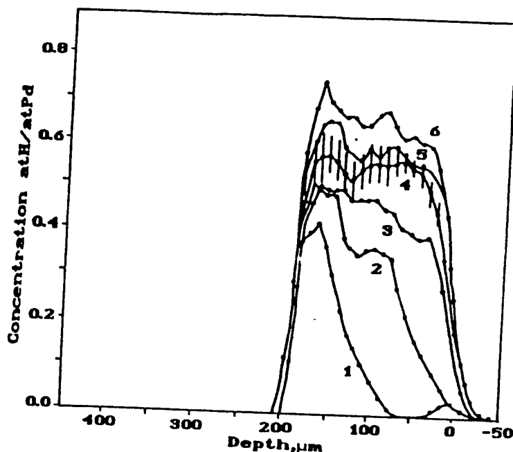
Figure 8: Hydrogen concentration profiles recorded by neutron ERD from 175 micron thick Pd samples electrolytically charged with hydrogen to various degrees. From reference [11].
