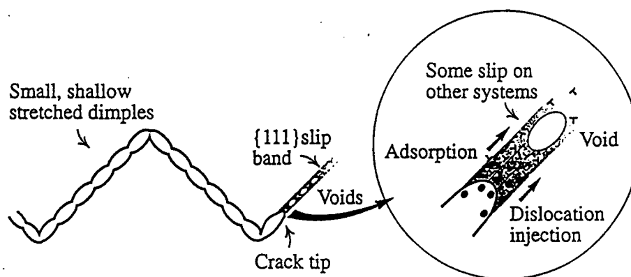
Fig. 4 Schematic diagram illustrating modified adsorption-induced localized slip process occurring along alternate shear planes.
