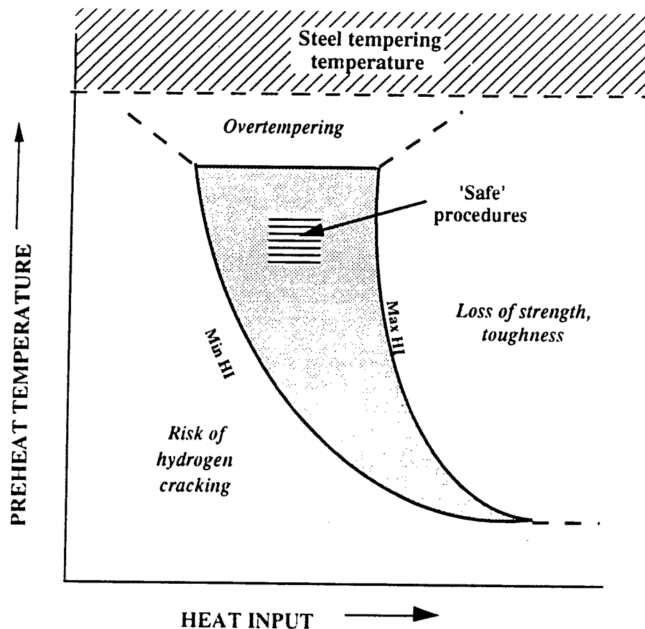
Figure 3 Unscaled graph (after Reference 10) showing the effect of preheat and heat input on weld zone properties. Acceptable properties are only obtained in the shaded region.
