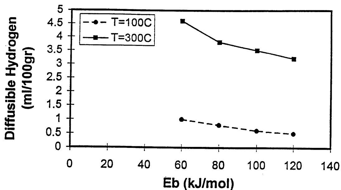
Figure 12. Effect of trap binding energy on the diffusible hydrogen content. Initial diffusible hydrogen content is 15 ml/100g. M_t = 400C , \Delta t_{8/5} is 5 seconds, trap density, N_t = 5 \times 10^{19} \text{ \#/cc} .
