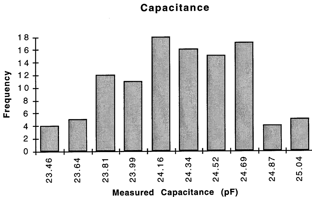
Figure 70. Censored Vendor B Wafer 2 measured capacitance.
