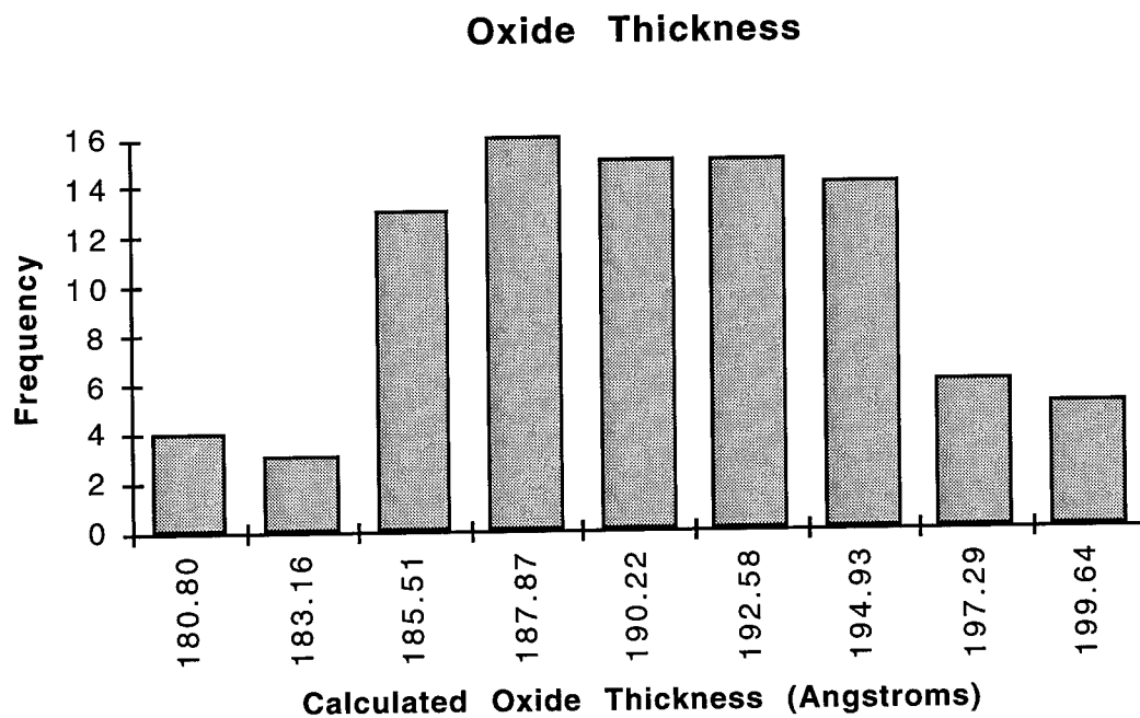
Figure 42. Censored Vendor A calculated oxide thickness.
