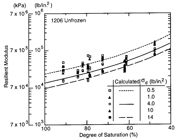
a. Low-density ( 1.66-1.7\text{-Mg/m}^3 or 104-106\text{-lb/ft}^3 ) 1206 subgrade. (These data are probably in error—see text.)
