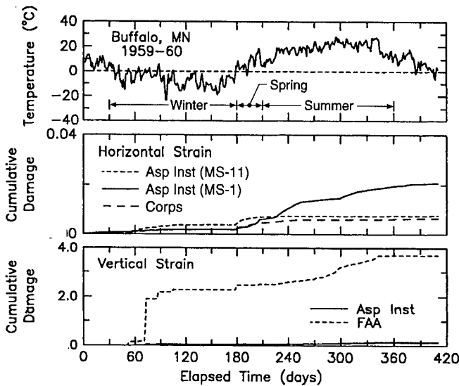
Figure 22. Cumulative damage for case f4w6 with "normal" subgrade.
