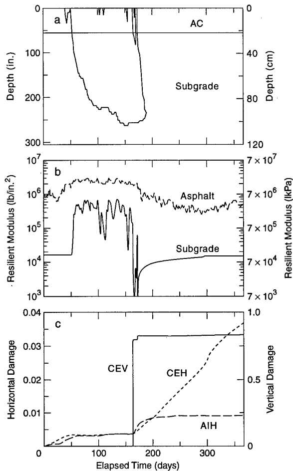
Figure 29. Predicted results from simulation of full-depth section during freeze season 1985–1986, starting on 1 October; a) frost/thaw depth, b) seed resilient modulus passed to NELAPAV, and c) cumulative damage (see Table 19).
