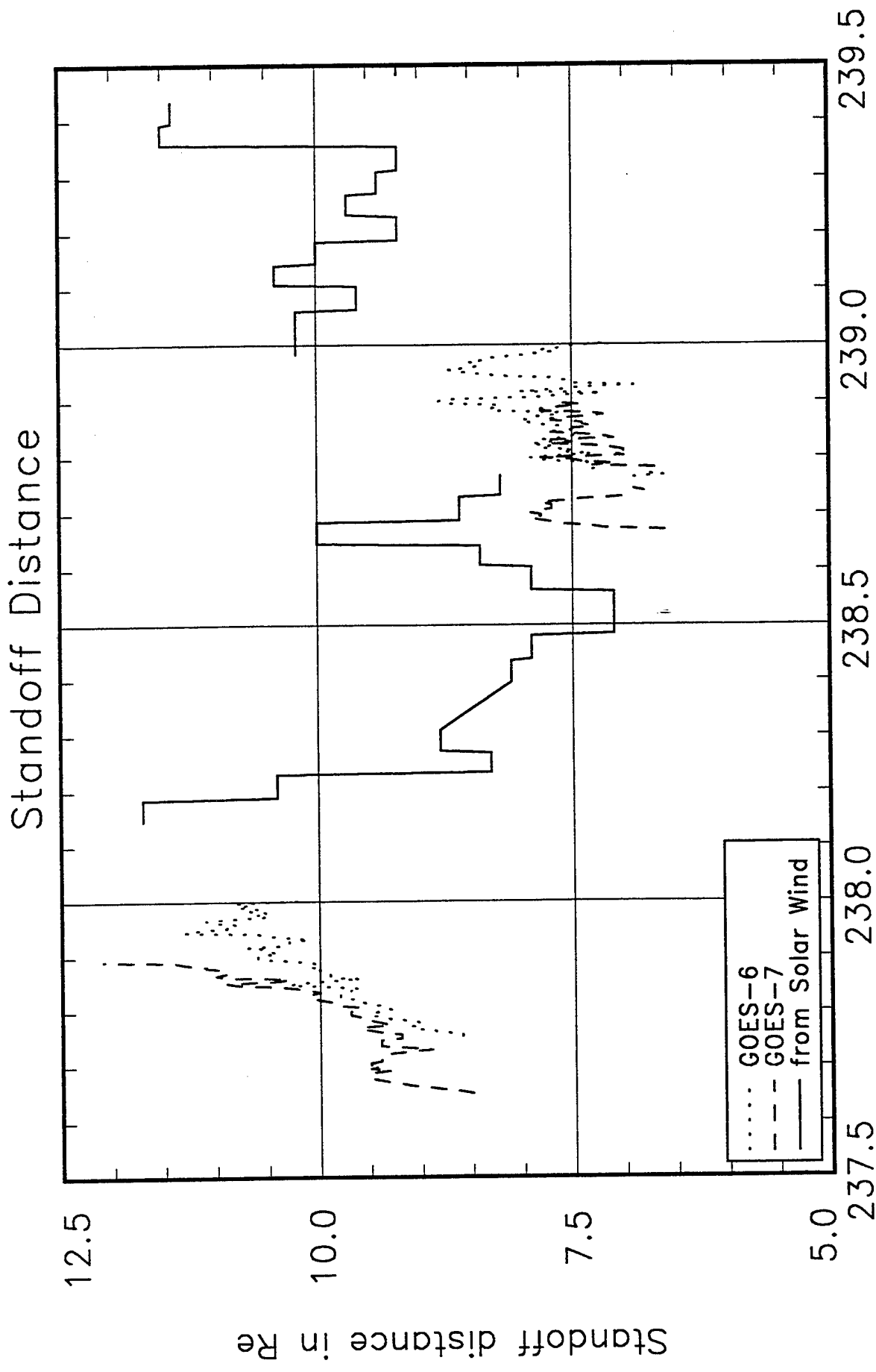
Figure 10. Best guess standoff distance from our standoff distance data base.
