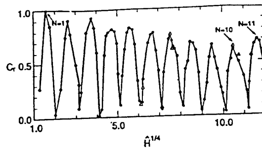
Plot of the coherence factor C_r versus H^{1/4} . b_n = 0.05 . The number of orbits for each energy is 355 (solid circle) or 598 (triangle). Straight lines are drawn between points. Peaks for N = 1, 10 and 11 are shown.
