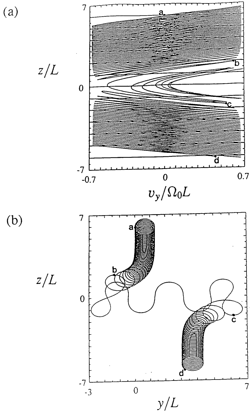
Figure 7: a) v_y / \Omega_0 L as a function of z/L for the particle in Fig. 5a. The particle is non midplane crossing on the segments a-b and c-d, and we use guiding center coordinates. The particle is midplane crossing on the segment b-c and we use true particle coordinates. Notes that if actual particle coordinates are used on the segments a-b and c-d, there is an excess of positive y-velocity in the regions 5.3 \leq z/L \leq 6.7 and -6.3 \leq z/L \leq -5 and an excess of negative y-current in the regions 0.5 \leq z/L \leq 1.9 and -2 \leq z/L \leq -0.3 . b) y/L as a function of z/L for the same particle. Note the \nabla B drift in the regions around |z/L| = 2 and the large y-velocity at |z/L| = 1 .
