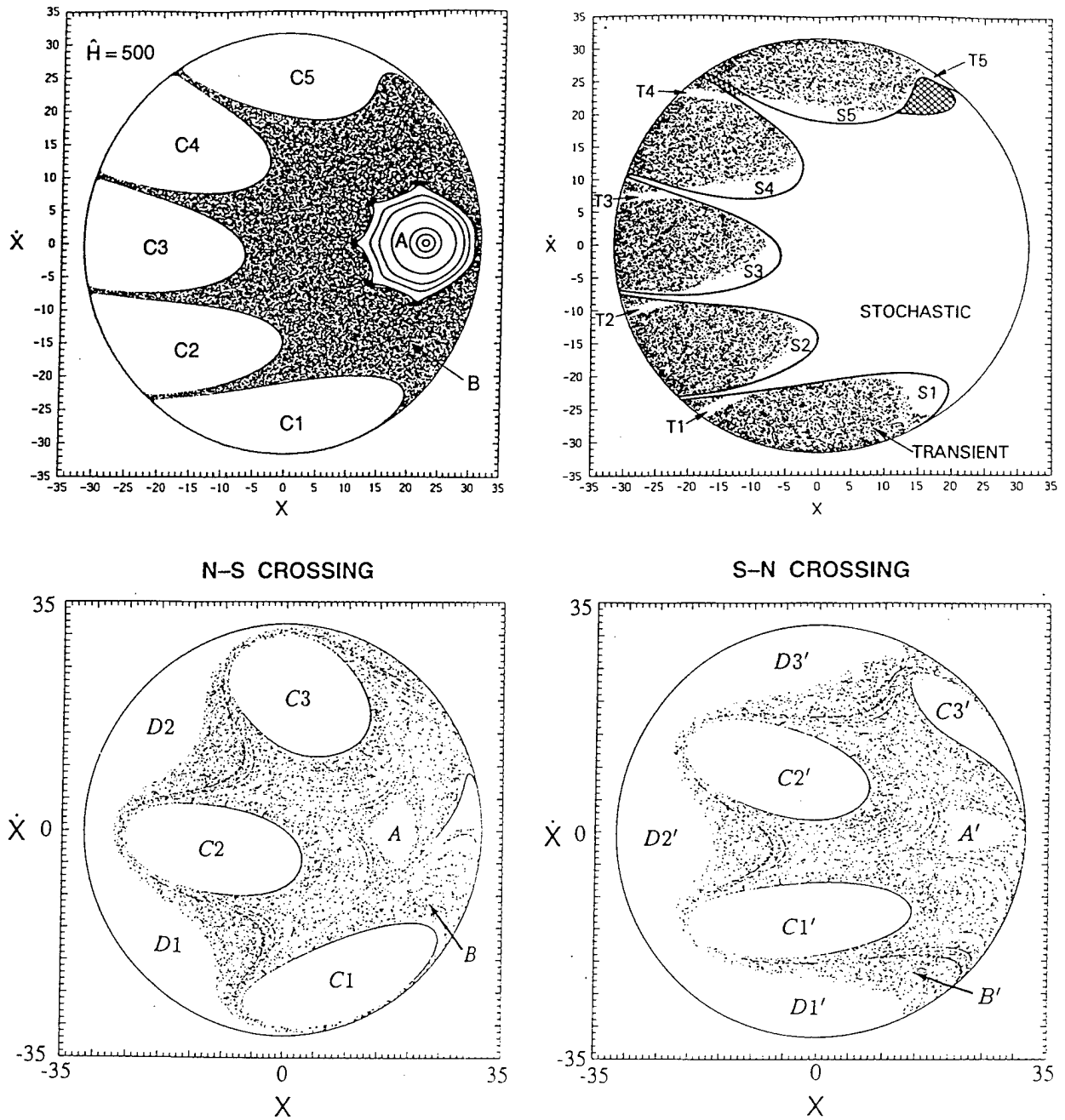
Fig. 4. A Poincaré surface of section map. b_n = 0.1 . Adapted from Chen and Palmadesso [1986]. (a) B_y = 0 . Region A is integrable and region B is stochastic. Regions C1 – C5 are transient regions. The boundaries \partial(C_j) are shown. (b) Internal structure of the transient regions. S1 and T1 are the entry regions for stochastic orbits. The orbits shown are transient orbits. (c) B_y = 0.1 B_0 . Surface of section return map for north-to-south crossings. (d) B_y = 0.1 B_0 . South-to-north crossings.
