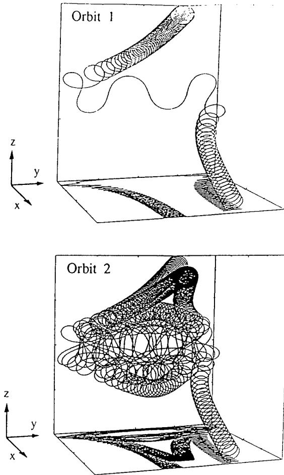
Fig. 3. Trajectories of two orbits with initial conditions \dot{H} = 500 , \beta = 100^\circ , and z = 3.5\delta . Orbit 1 has \theta = 20^\circ and orbit 2 has \theta = 50^\circ . From Holland and Chen [1991]
