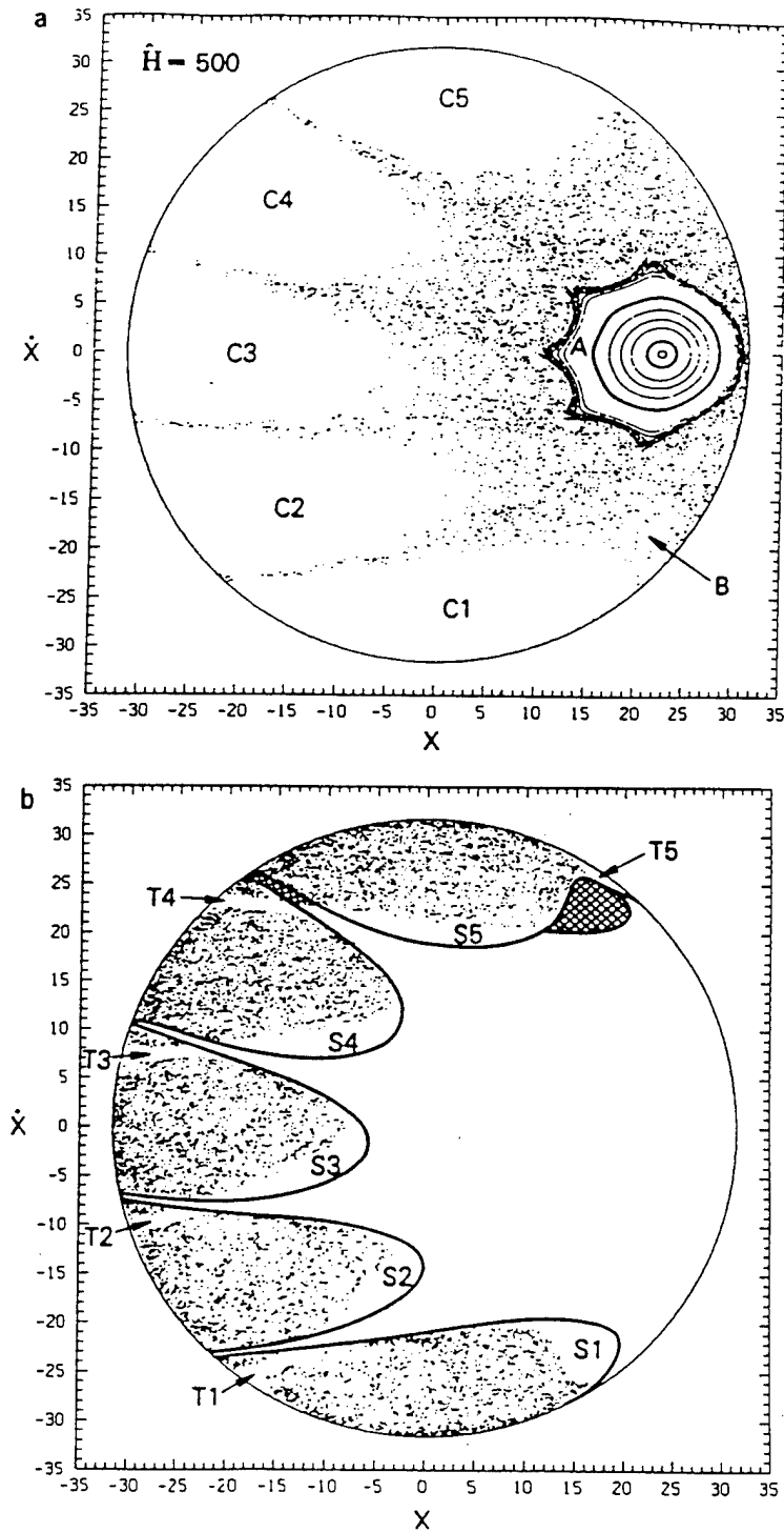
Surface of section plots for the Harris-type field with b_z = 0.1 and \tilde{H} = 500 . (a) Representative integrable orbits in region A and stochastic orbits in region B; 60,000 points. (b) Transient orbits, showing the substructures in regions C1-C5; 42,000 points.
