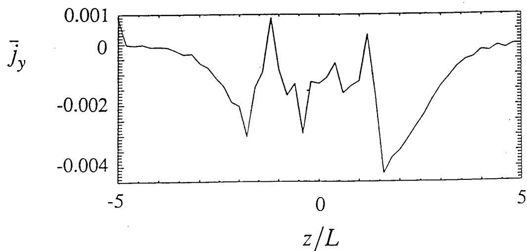
Figure 5: a) Trajectory of an ion with energy H = 0.24 L^2 \Omega_0^2 , initial pitch angle \beta = 100^\circ , initial phase angle \phi = 0^\circ and initial starting position z/L = 6 . b) Current profile of the particle in Fig. 3.a as calculated from the standard ridding algorithm with the top grid cell located at z/L = 5 .
