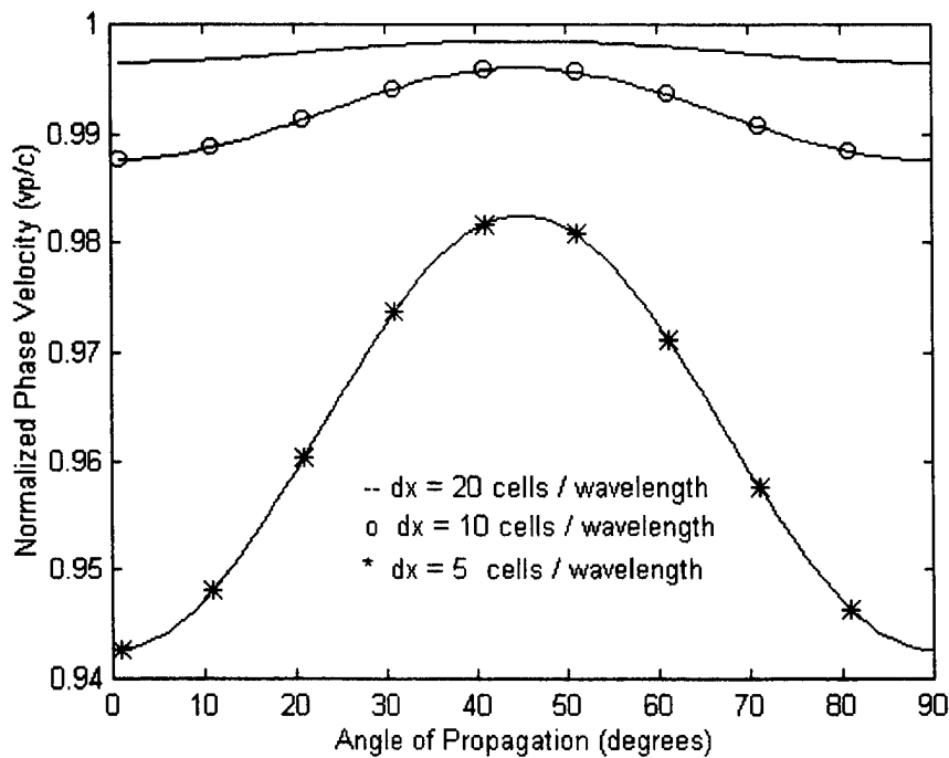
Figure 2: Variation of the numerical phase velocity with wave propagation angle in two-dimensional FDTD grid for three dimensions [Taflove]
