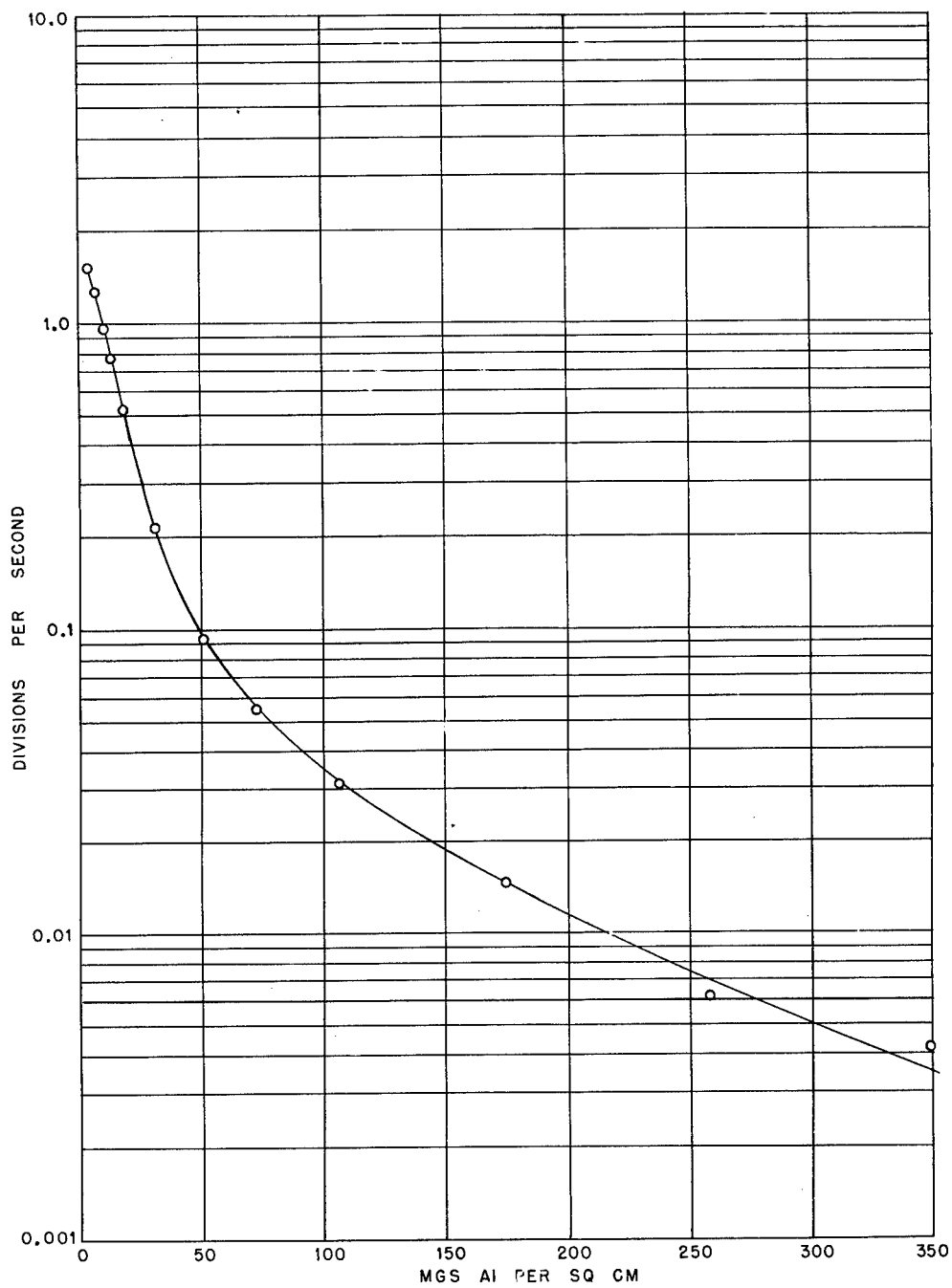
Figure 11. Al-absorption curve for Neptunium ( \text{Np}^{238} , \text{Np}^{239} ).
