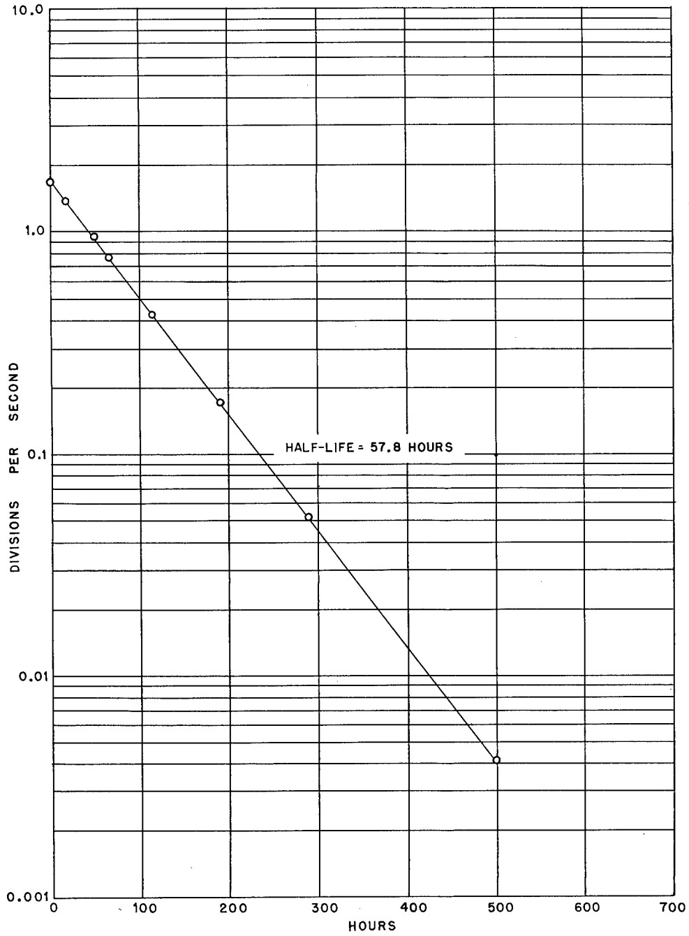
Figure 10. Decay curve for Neptunium ( Np^{238} , Np^{239} ).
