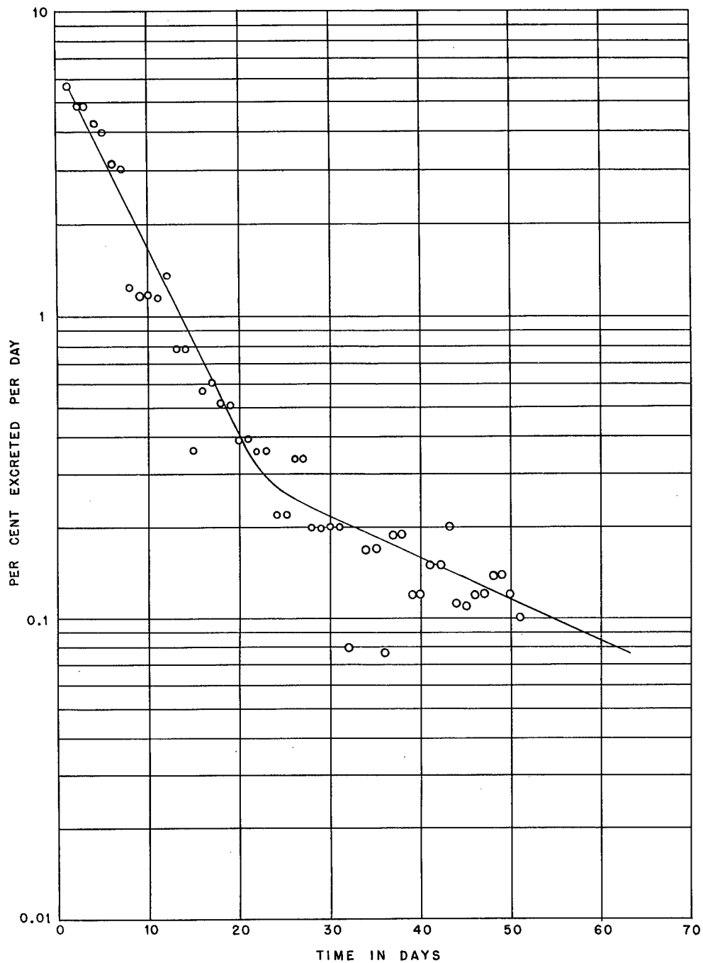
Figure 7. Fecal excretion of Ru -105 without carrier following intraperitoneal administration.
