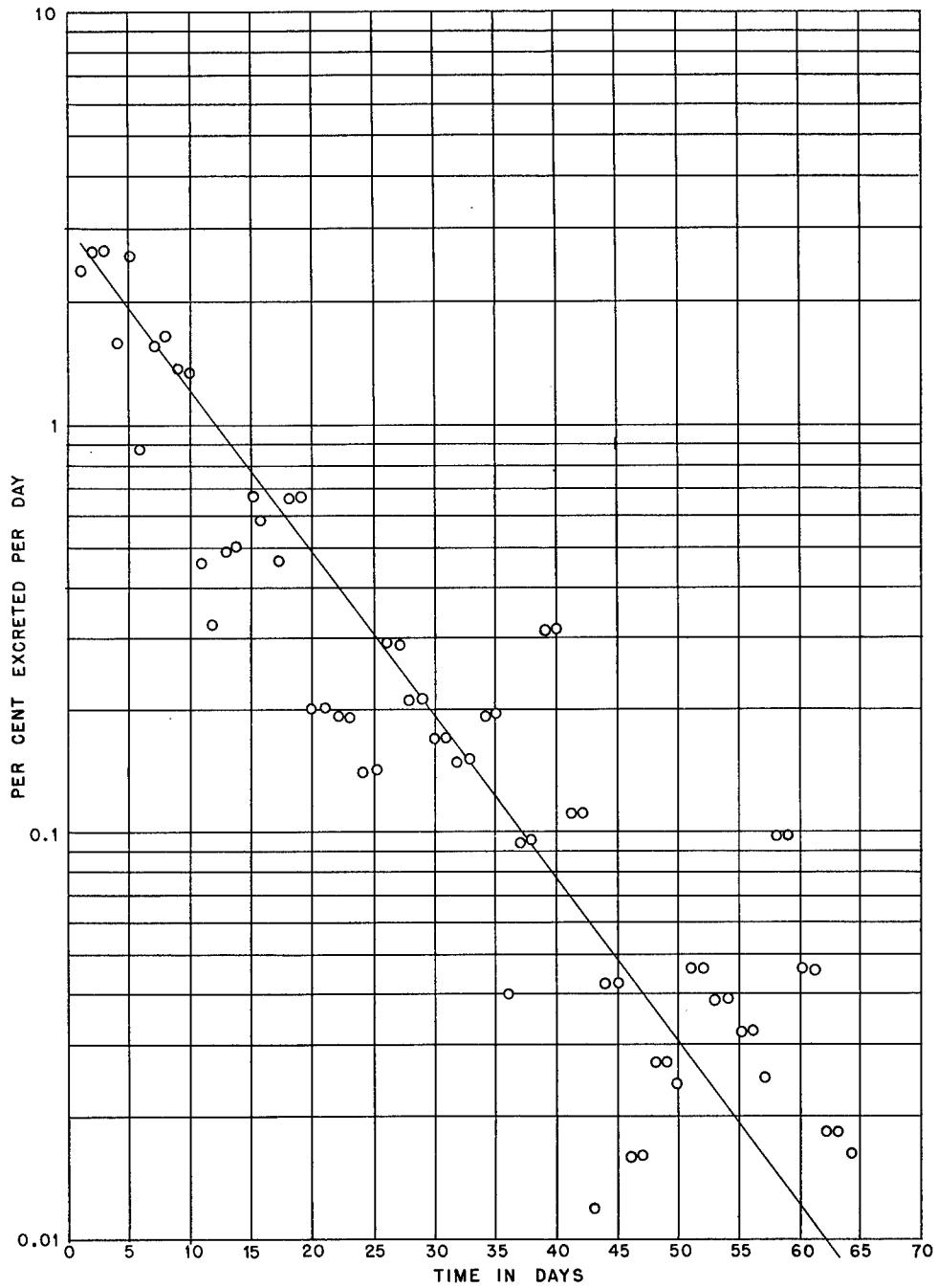
Figure 9. Fecal excretion of Ru^{105} without carrier following intramuscular administration.
