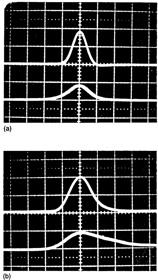
FIG. 3. Near-field mode profiles for 9.4 \mu\text{m} wide waveguide. (a) Horizontal scan with horiz. scale = 13.9 \mu\text{m}/\text{div} . and (b) vertical scan with horiz. scale = 7.7 \mu\text{m}/\text{div} . In both frames, upper traces are for TM with 200 mV/div. vertical scale, and lower traces are for TE with 50 mV/div. vertical scale.
