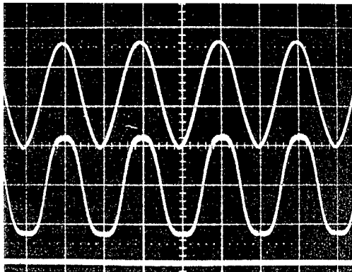
FIG. 3. Modulation response of 7.5 \mu\text{m} wide BSTN strain waveguide. Upper trace is the applied electrical signal at frequency = 100 kHz and 10 V/div. Lower trace is the optical response with zero level shown at the bottom.
