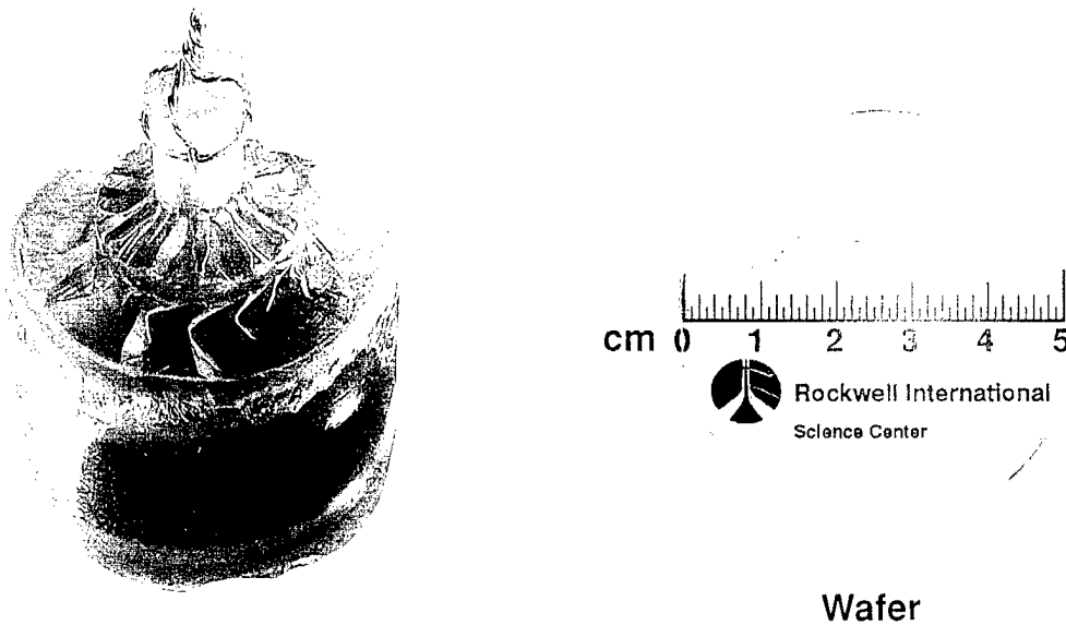
FIGURE 5 Large size tungsten bronze SBN single crystal boule grown along \langle 001 \rangle by the Czochralski method.
