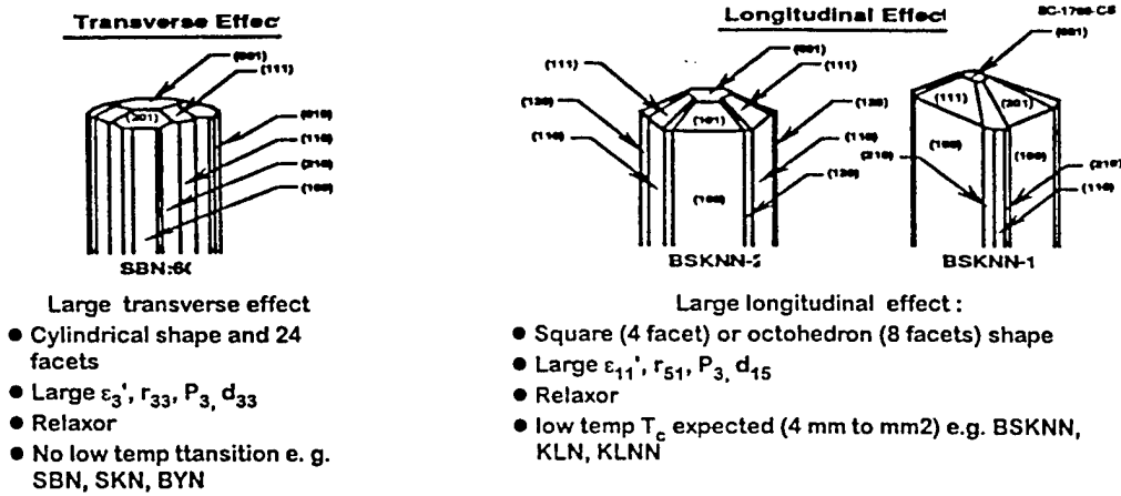
Figure 5 - Growth habits for tetragonal tungsten bronze crystals.
