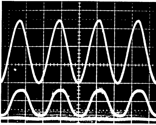
FIG. 4. Modulation response of 9.4 \mu\text{m} wide SBN:60 strain waveguide. Upper trace is the applied electrical signal at frequency=200 kHz and 10 V/div. Lower trace is the optical response with zero level shown at the bottom.
