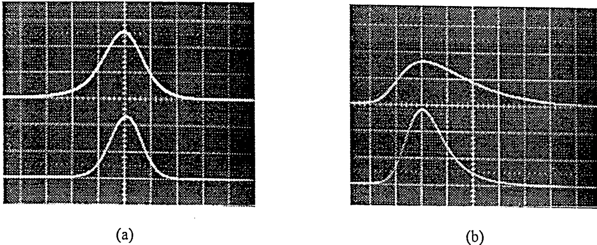
Figure 3.10: Near field mode profile of 11- \mu\text{m} wide BSTN strain waveguide at 1.3 \mu\text{m} wavelength. (a) Transverse scan. (b) vertical scan. In each photo, the upper trace is for TE and lower trace is for TM
