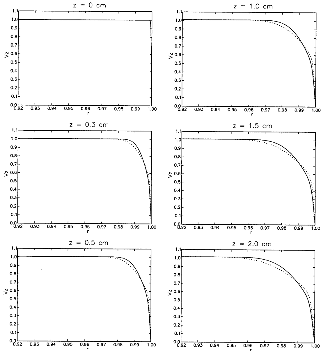
Figure 5.9: Steady state streamwise velocity profiles at different streamwise locations for high-speed injection of LP 1846 with U = 300\text{m/s} , and two different inlet temperature T_0 = 278^\circ\text{K} (dashed line), and T_0 = 298^\circ\text{K} (solid line). The uniform Peclet number model is adopted, and the computations are performed using the steady parabolized approximation on a stretched grid with a stretching parameter a = 6.5 , N_r = 401 points in the radial direction and N_z = 8001 points in the streamwise direction.
