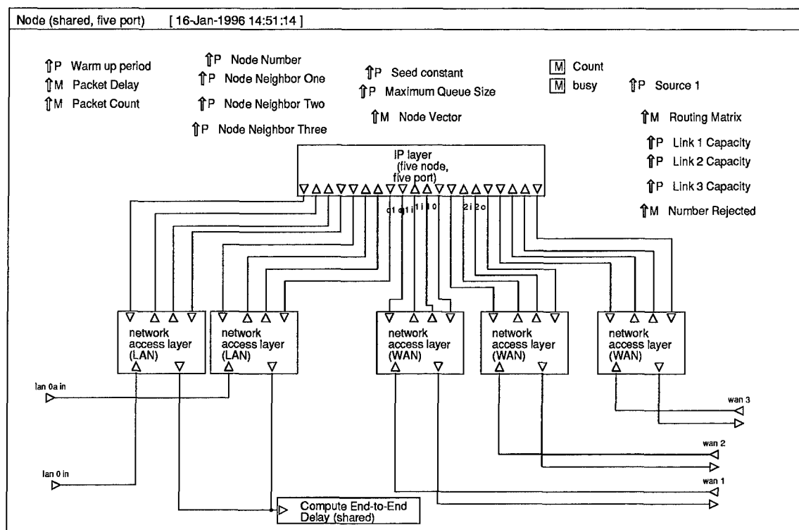
Figure 3.25 Node Module.
