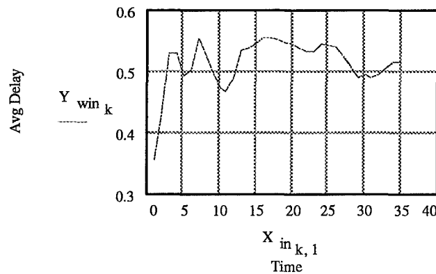
Figure 3.37 Results of Welch's Algorithm
