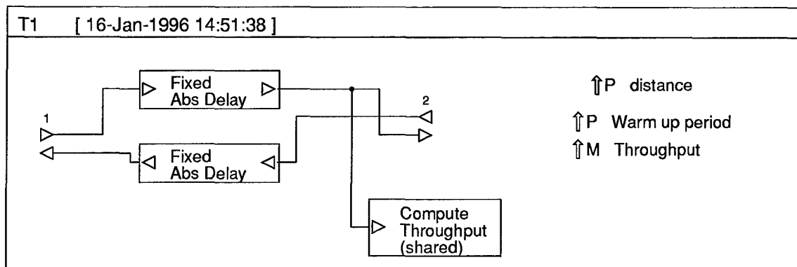
Figure 3.24 T1 Module
