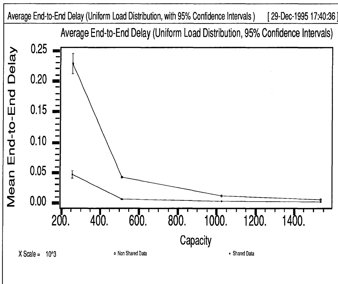
Figure 4.17 Mean End-to-End Delay Versus Capacity (Delay scaled in seconds)
