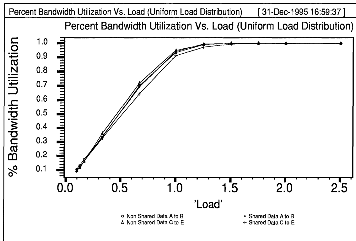
Figure 4.13 % Bandwidth Utilization ( \times 100 ) Versus Load
