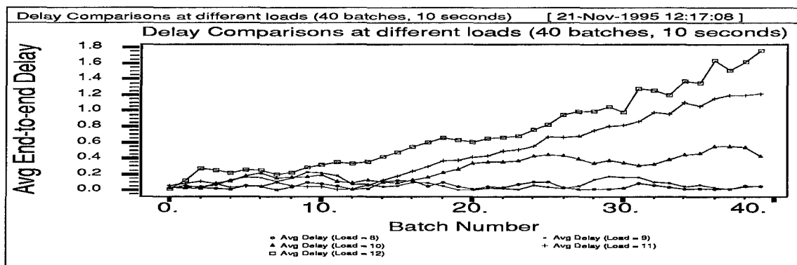
Figure 3.9 Delay Comparisons at Different Loads
