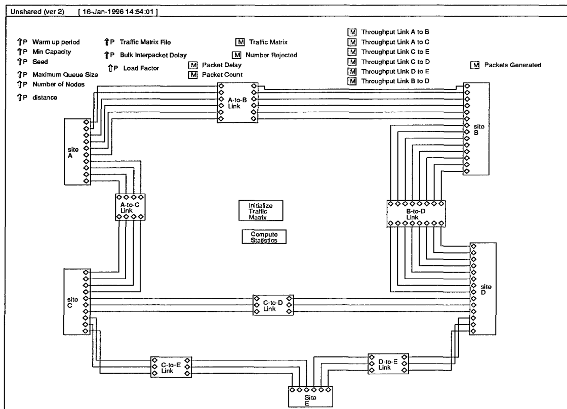
Figure 3.29 Nonshared System
