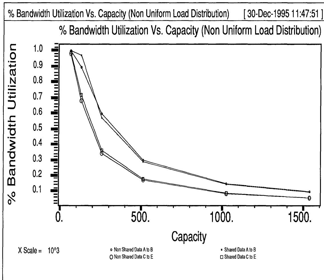
Figure 4.19 Percent Bandwidth Utilization ( \times 100 ) Versus Capacity (Non Uniform Load)
