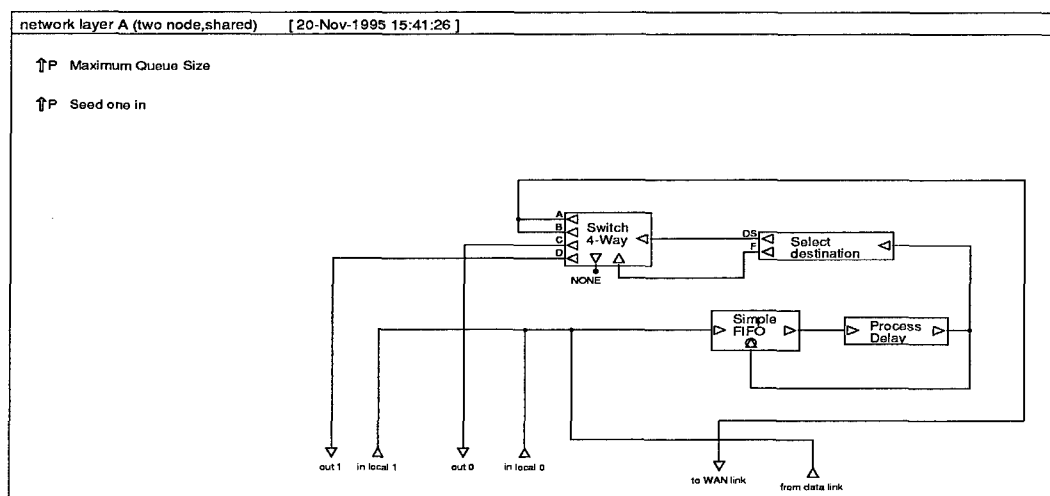
Figure 3.4 Network Layer
