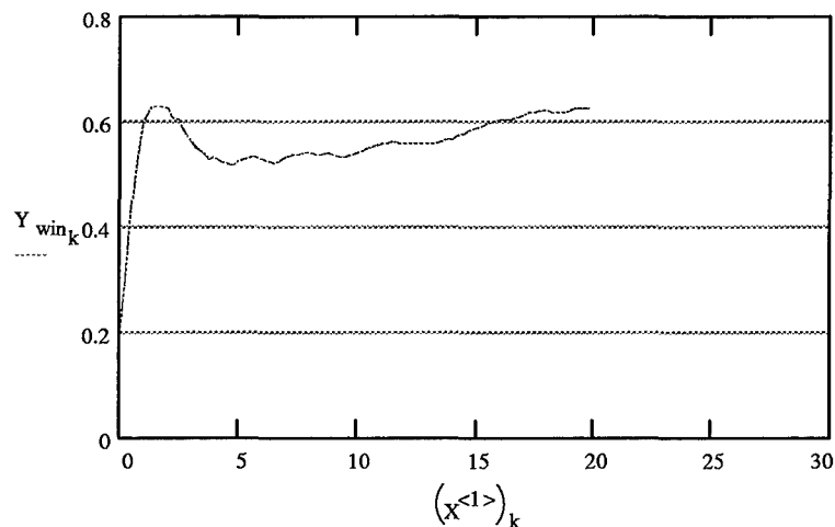
Figure 3.12 Warm Up Time Determination (Welch's Algorithm)
