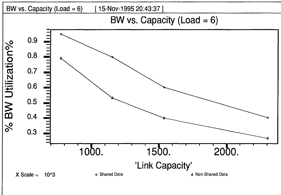
Figure 4.9 Percent BW ( \times 100 ) Versus Capacity (Load = 6)
