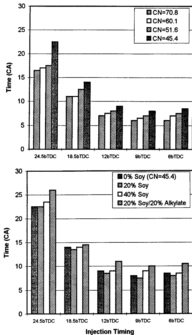
Fig. 10. Variation of Time from Injection: (A) to Rapid Pressure Rise and (B) to Maximum dP/dt.
