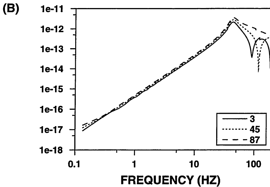
Figure 6: Log-log plot of the spectra of the wavefields generated by the (A) instantaneous pressurization and (B) volume injection point source models in the cavity of aspect ratio 5 (isotropic formation). The volume injection source was centered in the cavity. The hard rock formation velocities are given in Figure 2. Each plot shows the spectrum observed at 3, 45 and 87 degrees from the cavity axis.
