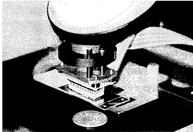
Fig. 9 - Kensal Corporation's laboratory demonstration of a lensless microscope.
