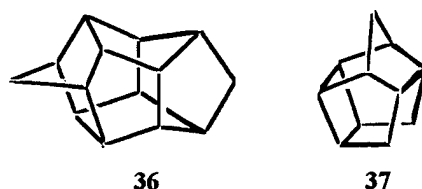
Scheme 9
