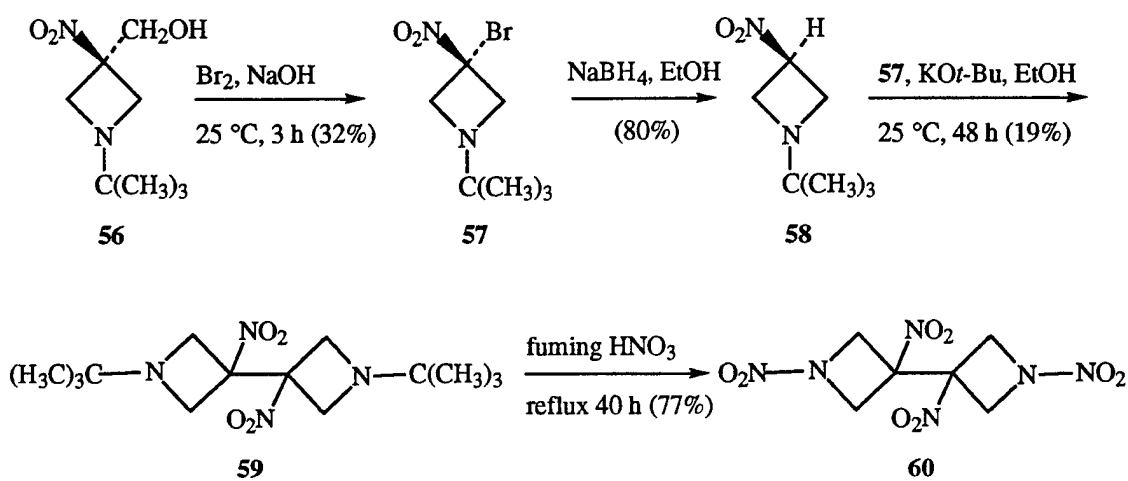
Scheme 15
