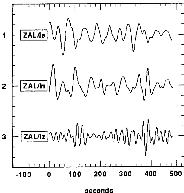
Figure 4. Seismograms showing high horizontal noise levels at station ZAL, 12.7 degrees from the Chinese nuclear test of July 28, 1996. This event had an M_s of 2.8 based on arrivals at ZAL and NRI.
