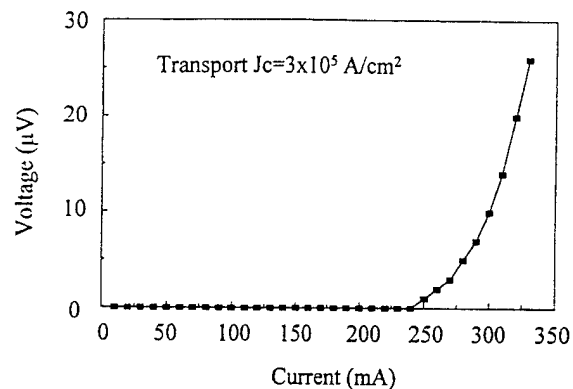
FIG. 5. I - V curve for measuring the transport J_c of the \text{Tl}_2\text{Ba}_2\text{CaCu}_2\text{O}_8 film on SAT/MgO.
