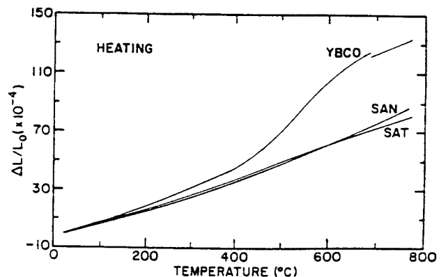
FIG. 7. Thermal strain measured by using a vertical push rod linear voltage differential transformer dilatometer.
