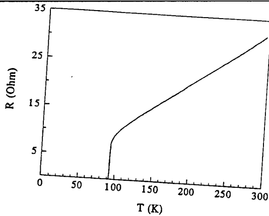
FIG. 4. Resistance vs temperature for a 3000 Å YBCO film on SAT/MgO.
