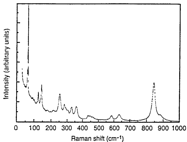
Figure 4 Micro-probe Raman spectrum of SAT sintered at 1400 °C for 7 h.
