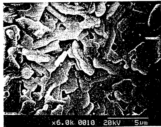
FIG. 1. SEM photograph of a \text{Tl}_2\text{Ba}_2\text{CaCu}_2\text{O}_8 superconducting film on SAT/MgO.
