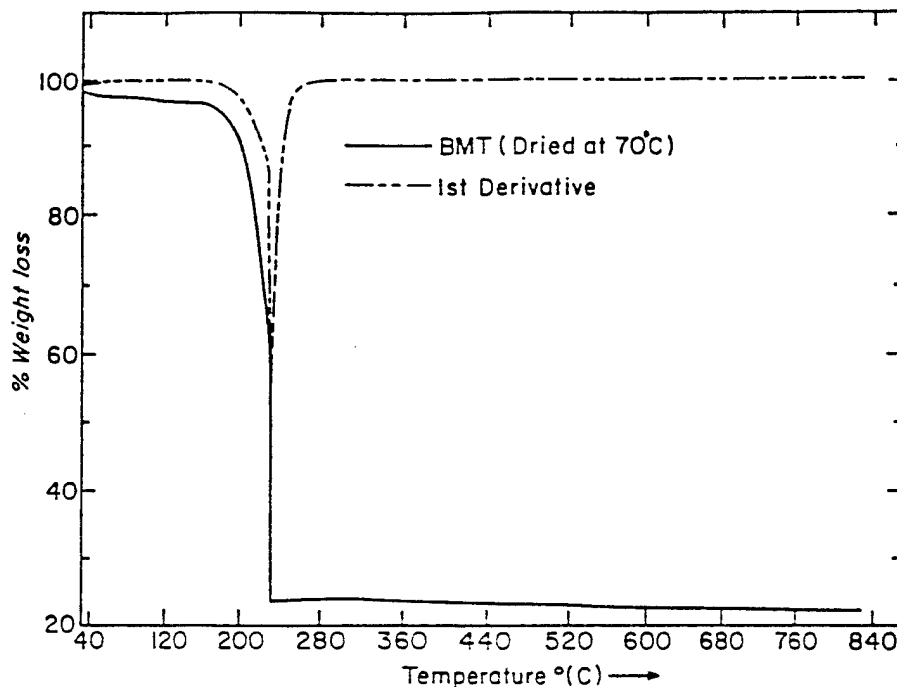
FIG. 2 TGA trace of BMT gel dried at 70°C in an air atmosphere.
