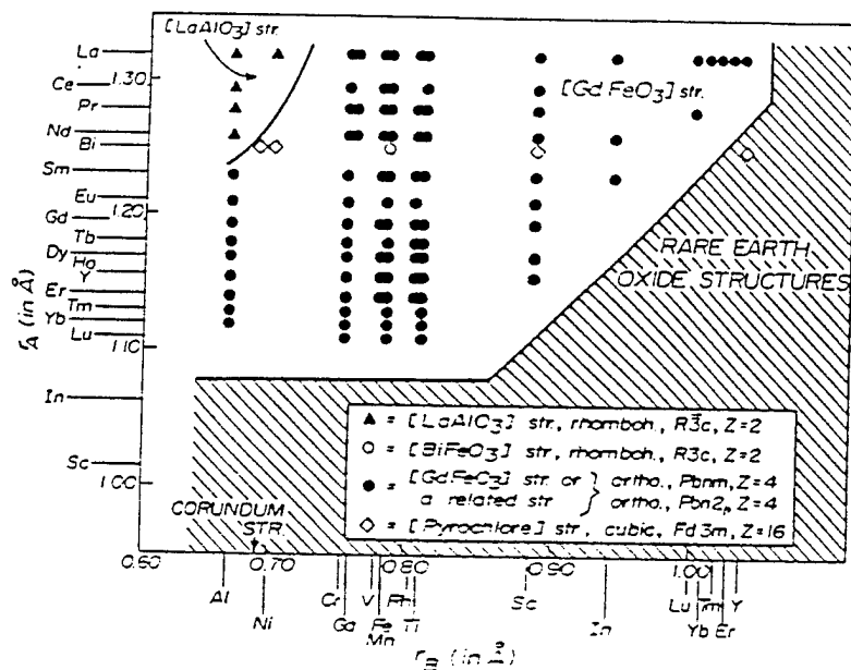
Fig. 4. Structure field map for [\text{A}]^{\text{B}3-}[\text{B}]^{\text{3}+}\text{O}_3 type compounds (ref. 15).
