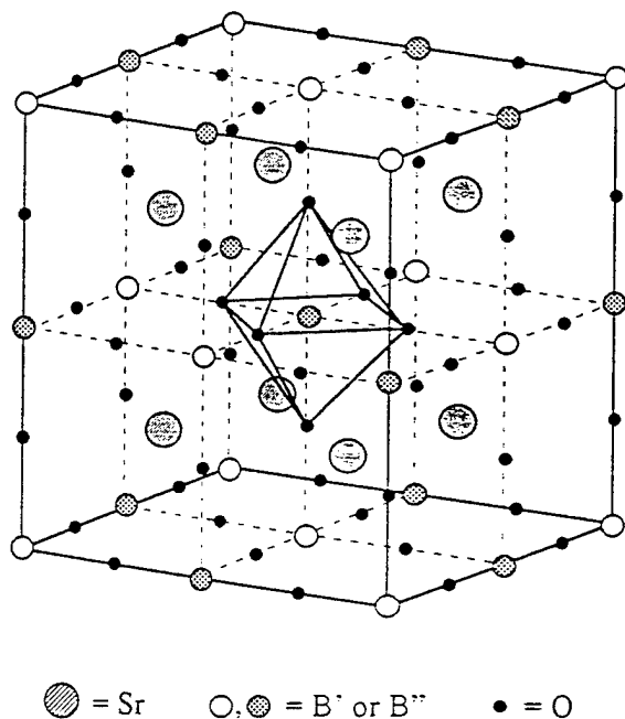
Fig. 1 The unit cell of SAN and SAT with Fm\bar{3}m symmetry.
