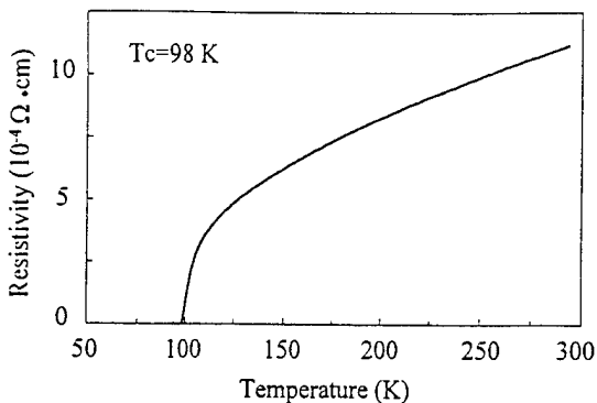
FIG. 4. Resistivity vs temperature for the \text{Tl}_2\text{Ba}_2\text{CaCu}_2\text{O}_8 film on SAT/MgO.
