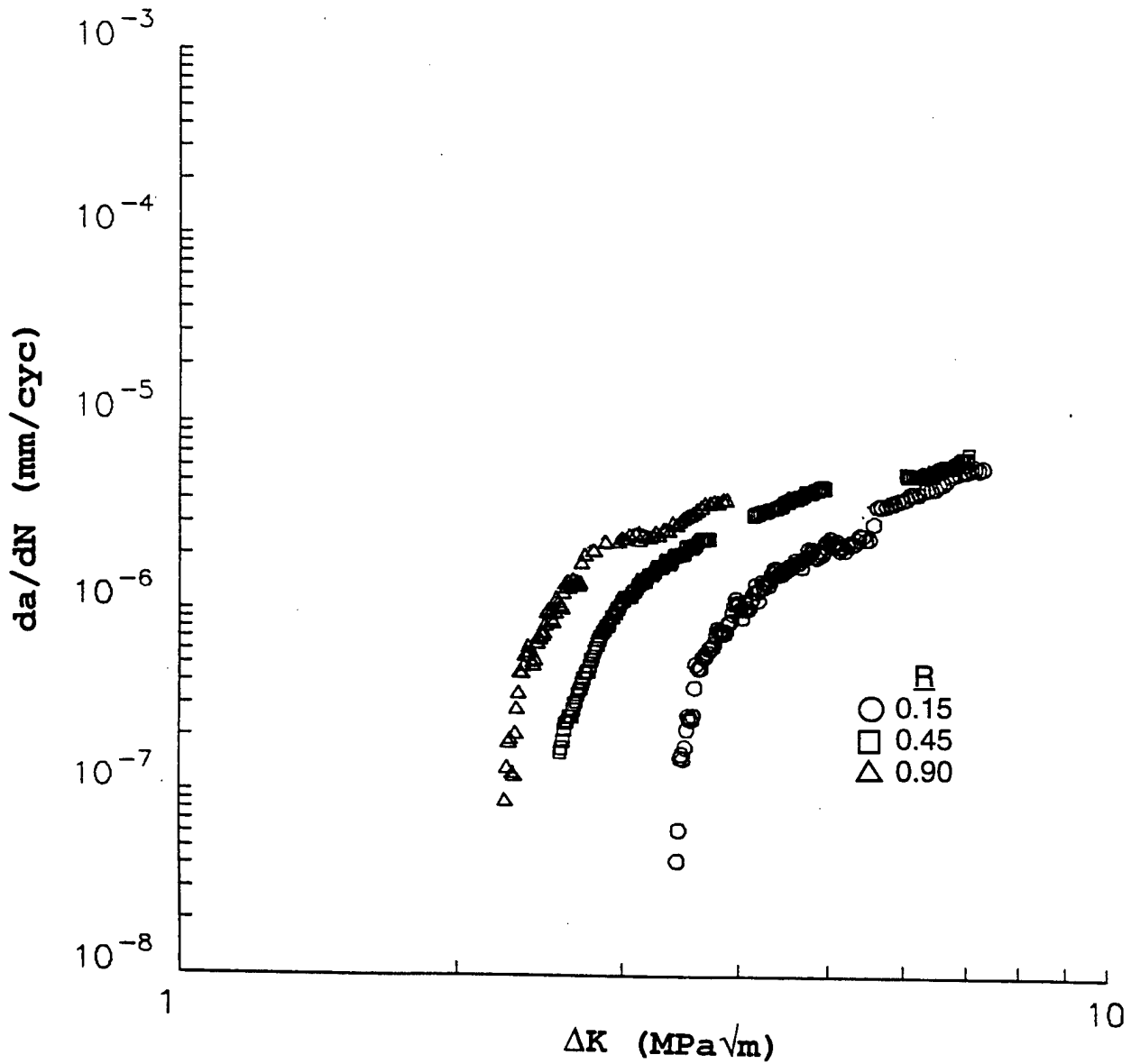
Figure A-3 VARIATION OF FATIGUE CRACK GROWTH RATE, da/dN , WITH STRESS INTENSITY RANGE, \Delta K , AT LOAD RATIO R=0.15, 0.45, \text{ AND } 0.9
