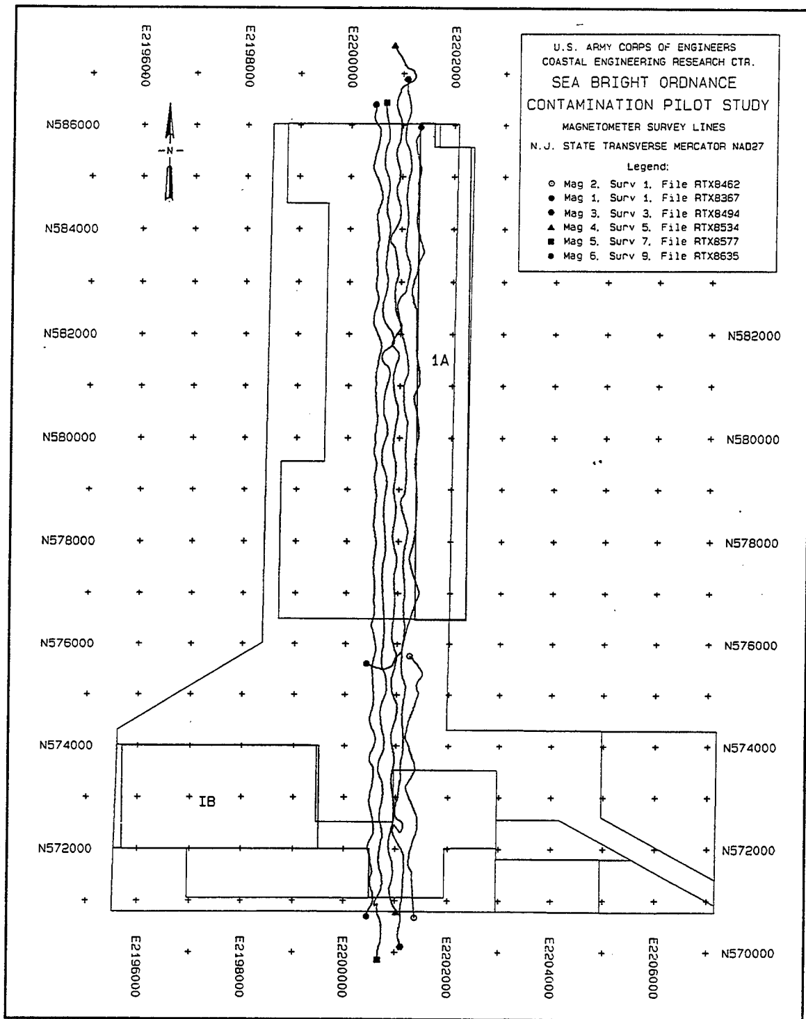
Figure 7. Long magnetometer survey lines. Overall Sea Bright borrow area shown for reference
