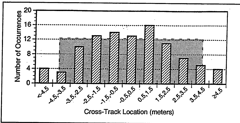
Figure 29. Cross-track locations, 100 analyzed samples. Shaded area indicates computed detection range of array used in the field. (Plot provided by AETC)
