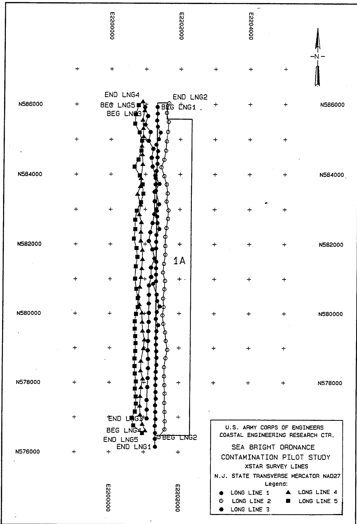
Figure 5. X-star subbottom profiler survey lines. Borrow area 1A shown for reference
