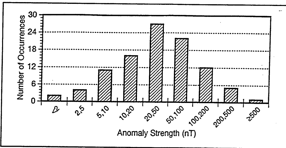
Figure 28. Anomaly strength (peak signal magnitude) of 100 samples selected from the north-south magnetometer lines. (Plot provided by AETC)
