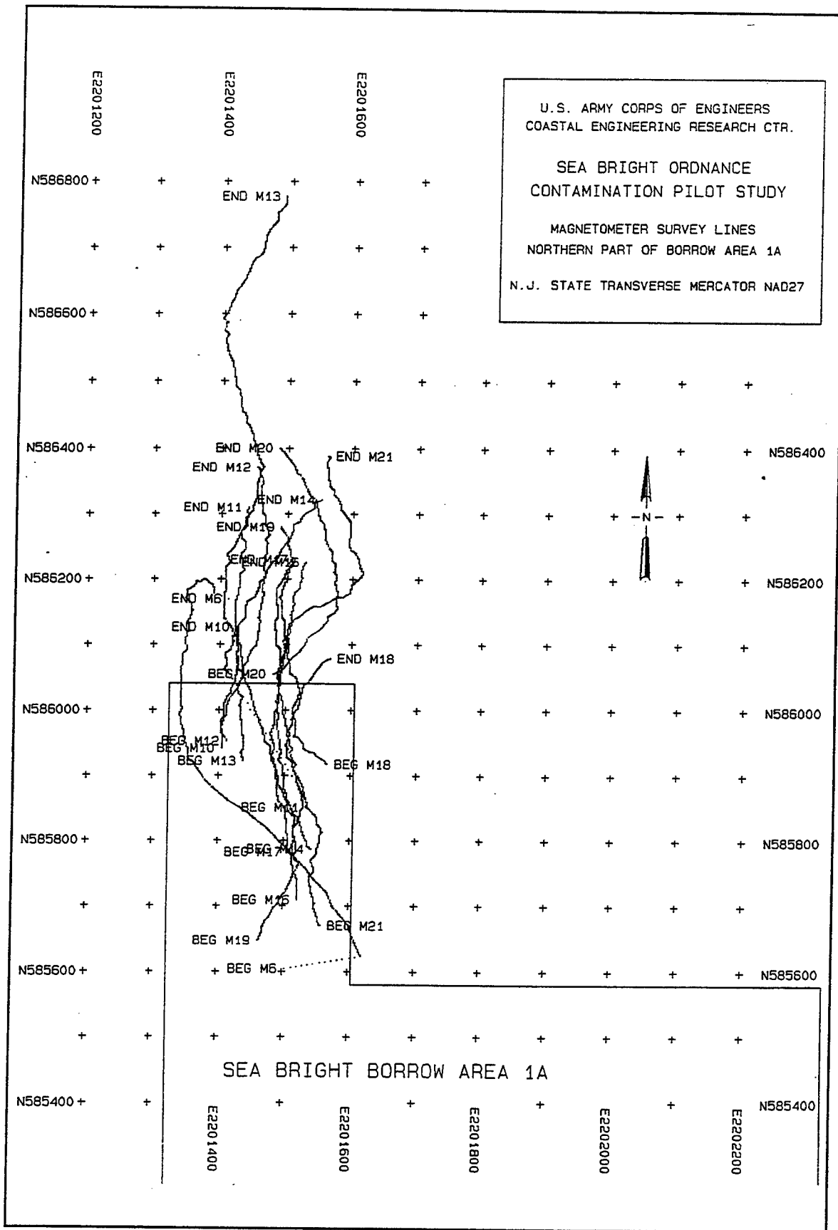
Figure 6. Magnetometer survey lines, northern portion of borrow area 1A
