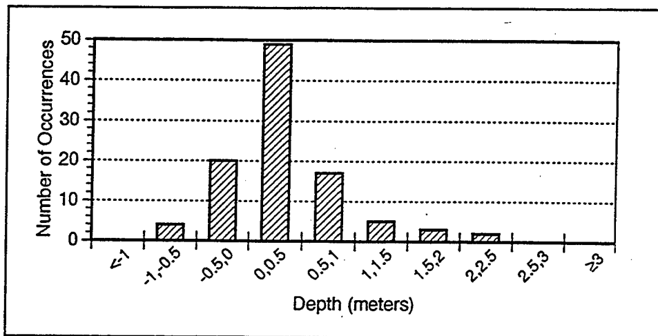
Figure 30. Computed depth from seafloor to center of objects. Negative values correspond to dipole fits where the center of object is above the bottom. Most objects are lying on the seafloor. (Plot provided by AETC)
