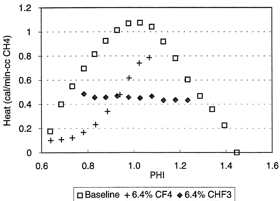
Figure 3. Reduction in Heat Absorbed by the Burner.
