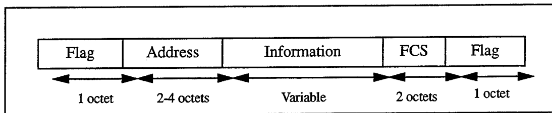
Figure 5.3 Frame Format
