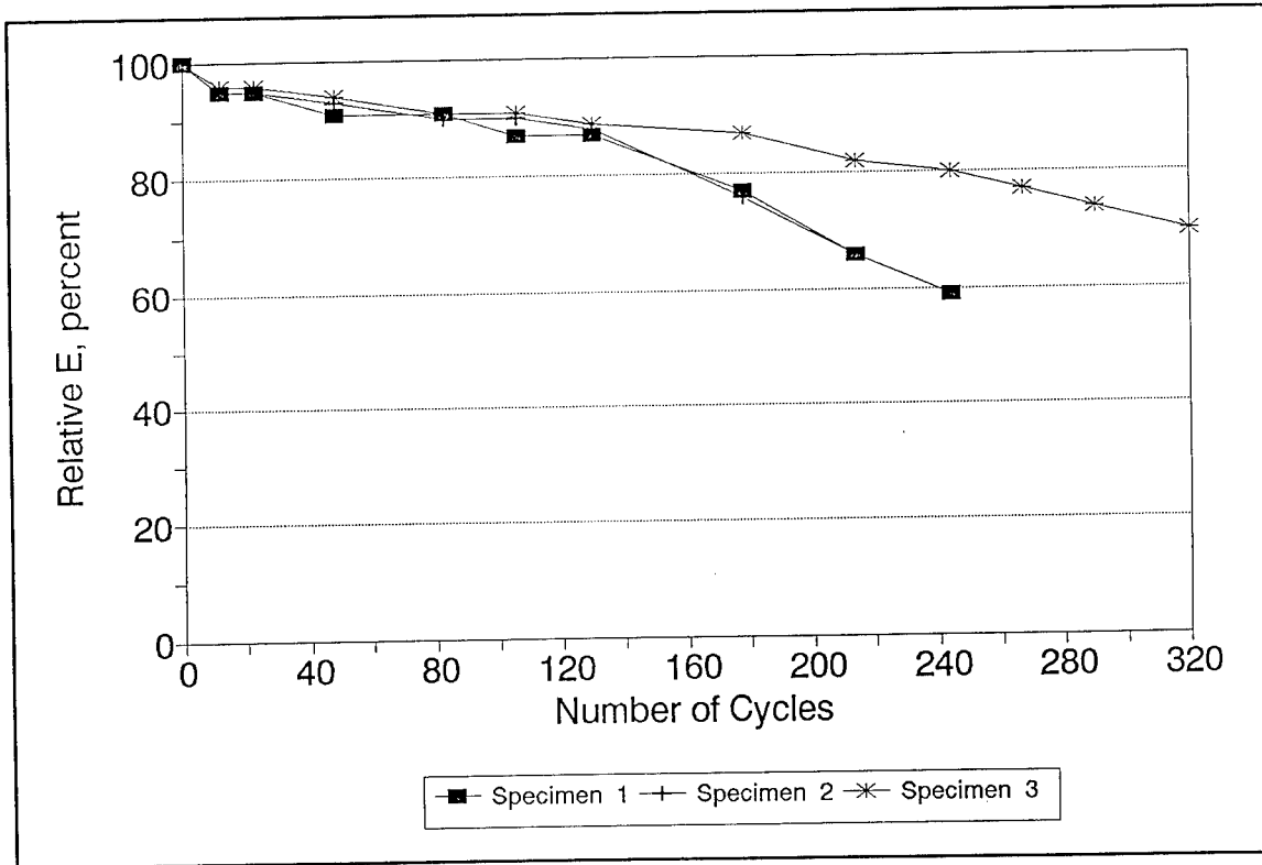
Figure 11. Results of freezing-and-thawing test on material P-8
