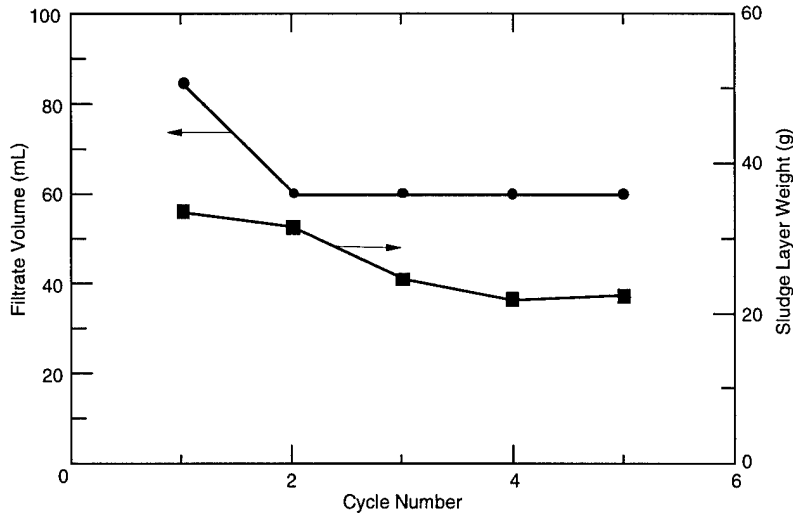
Figure 13. Effect of repeated use of cloth 2019 at 100 mm of Hg vacuum and a 5.0-minute filtration time in alum sludge containing 1.0% solids.
