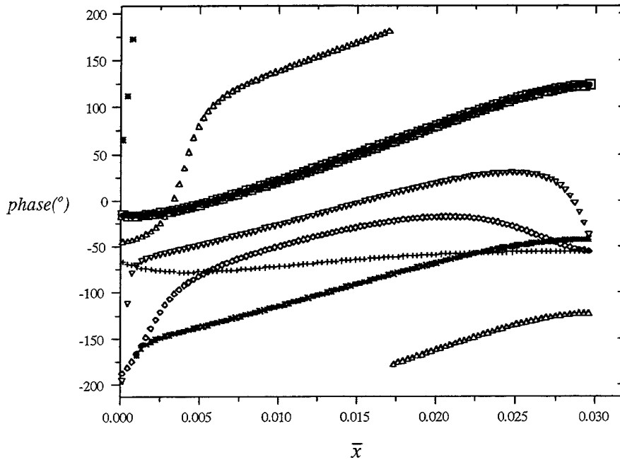
Figure 5.5. Relative phase (in degrees) for the eigenfunctions \hat{n}_e ( \square ), \hat{U}_e ( \bullet ), \hat{T}_e (+), \hat{U}_i ( \nabla ), \hat{E} ( \diamond ), d\hat{T}_e/d\bar{x} ( \Delta ), \hat{T}_e (*). Note that the electron density and velocity perturbations are approximately in phase.
