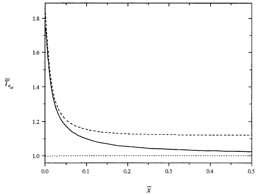
Figure 3.2. Profiles of the non-dimensional electron temperature for \bar{J} = 400 (dashed), 40 (solid), and 0.4 (dotted).
