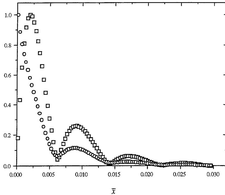
Figure 5.12. Normalized Amplitudes for the eigenfunctions \hat{U}_i ( \square ), \hat{E} ( \circ ). The maximum values of the amplitudes are 3.06 \times 10^{-4} and 2.44 \times 10^{-3} , respectively.
