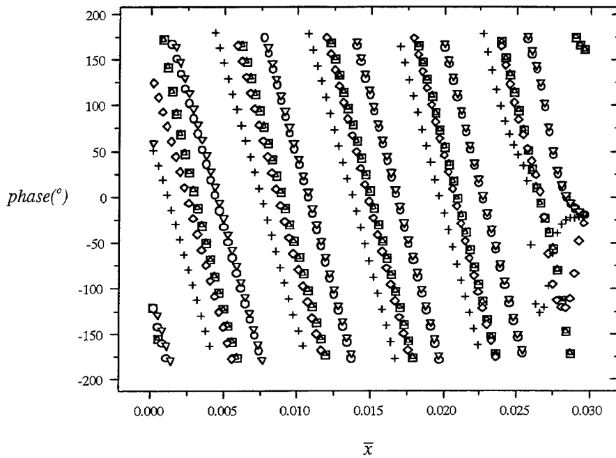
Figure 5.17. Relative phase (in degrees) for the eigenfunctions \hat{n}_e ( \square ), \hat{U}_e ( \circ ), \hat{T}_e ( + ), \hat{U}_i ( \nabla ), \hat{E} ( \diamond ), d\hat{T}_e/dx ( \Delta ), \hat{T}_e ( * ), ion mode. Note that the electron density and velocity perturbations are approximately in phase.
