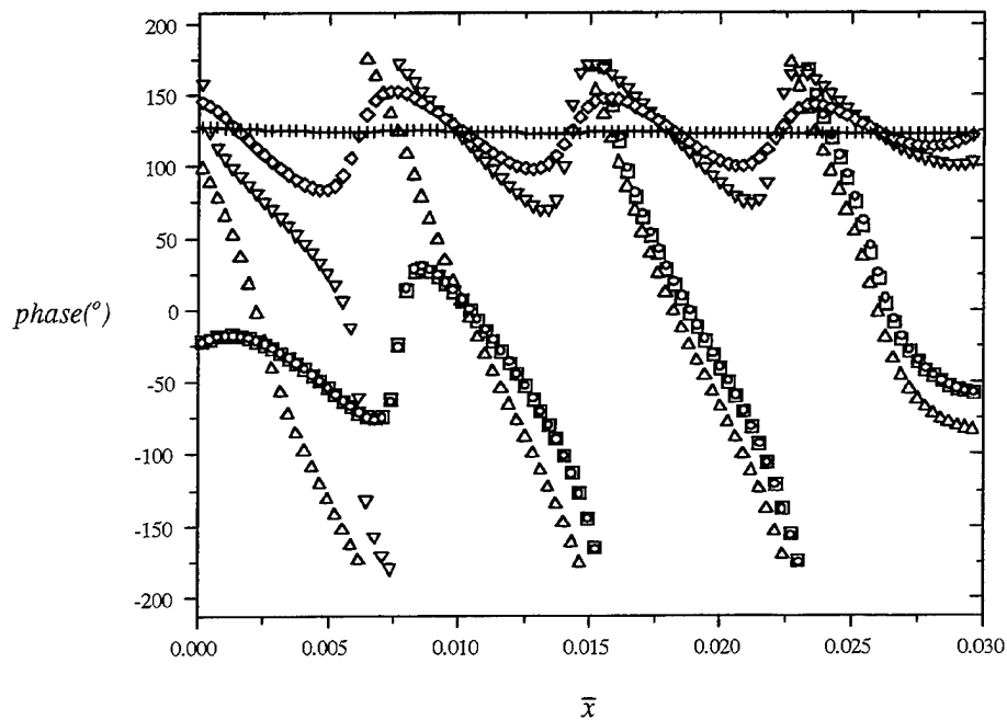
Figure 5.13. Relative phase (in degrees) for the eigenfunctions \hat{n}_e ( \square ), \hat{U}_e ( \circ ), \hat{T}_e ( \triangle ), \hat{U}_i ( \nabla ), \hat{E} ( \diamond ), d\hat{T}_e/d\bar{x} ( \Delta ). Note that the electron density and velocity perturbations are approximately in phase, and that phase of \hat{T}_e is not plotted because it has the same phase as the ion velocity perturbation.
