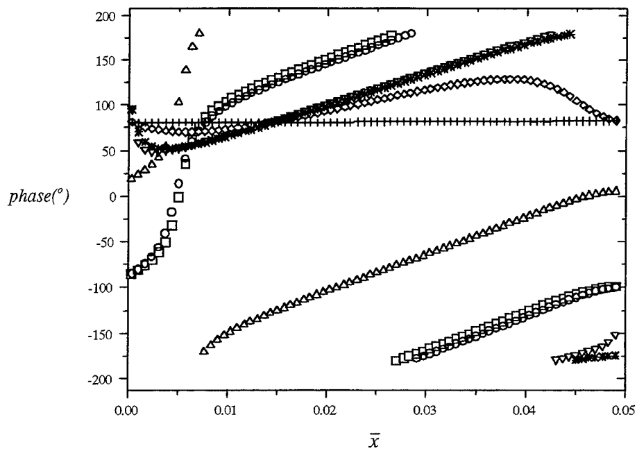
Figure 5.9. Relative phase (in degrees) for the eigenfunctions \hat{n}_e ( \square ), \hat{U}_e ( \circ ), \hat{T}_e ( + ), \hat{U}_i ( \nabla ), \hat{E} ( \diamond ), \hat{d}\Gamma_e/dx ( \Delta ), \hat{\Gamma}_e ( * ). Note that the electron density and velocity perturbations are approximately in phase.
