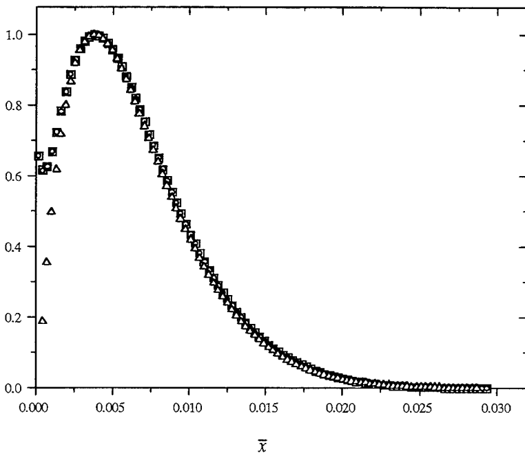
Figure 5.15. Normalized Amplitudes for the eigenfunctions \hat{n}_e ( \square ), d\hat{T}_e/d\bar{x} ( \circ ), \hat{T}_e ( \Delta ), ion mode. The maximum values of the amplitudes are 1.09 \times 10^5 , 0.21 , and 6.11 \times 10^4 , respectively.
