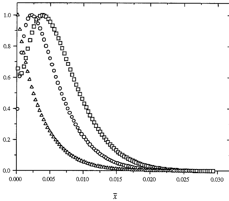
Figure 5.14. Normalized Amplitudes for the eigenfunctions \hat{n}_e ( \square ), \hat{U}_e ( \circ ), \hat{T}_e ( \Delta ), ion mode. The maximum values of the amplitudes are 1.09 \times 10^5 , 0.471 , and 1.72 \times 10^3 , respectively.
