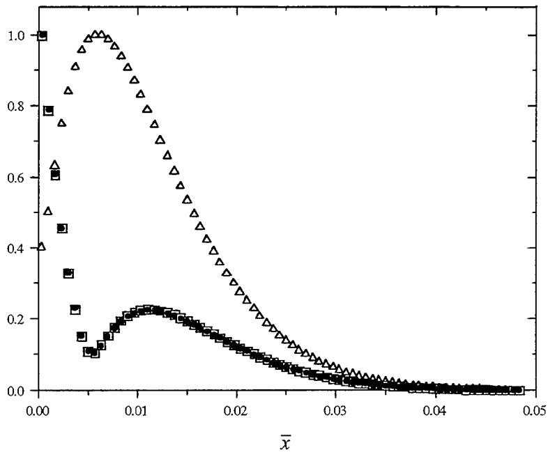
Figure 5.7. Normalized Amplitudes for the eigenfunctions \hat{n}_e(\square) , d\hat{\Gamma}_e/d\bar{x}(\bullet) , \hat{\Gamma}_e(\Delta) . The maximum values of the amplitudes are 1.09 \times 10^{-5} , 0.21 , and 6.11 \times 10^{-4} , respectively.
