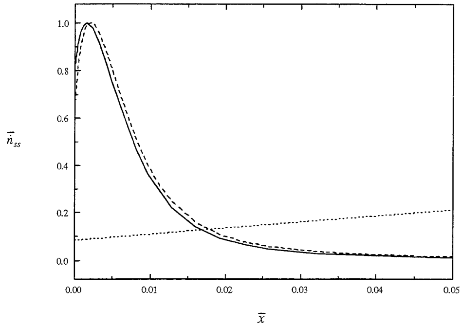
Figure 3.5. Near-anode view of Figure 3.4.
