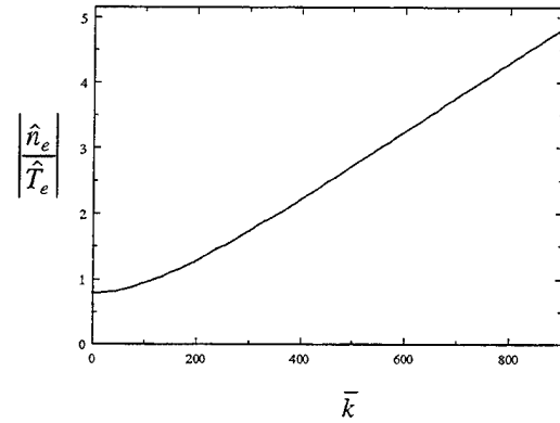
Figure 4.12. Relative amplitude between the electron number density and temperature for the thermal mode.
