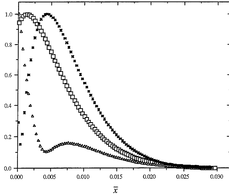
Figure 5.4. Normalized Amplitudes for the eigenfunctions \hat{n}_e ( \square ), d\hat{T}_e/d\bar{x} ( \Delta ), \hat{T}_e (*). The maximum values of the amplitudes are 1.88 \times 10^7 , 1.33 \times 10^4 , and 8.91 \times 10^4 , respectively. Note the discontinuity in the flux amplitude at the anode wall.
