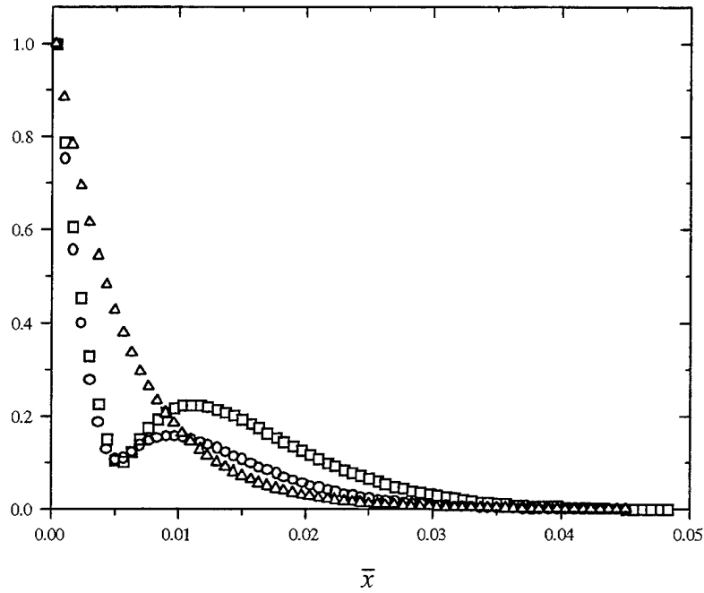
Figure 5.6. Normalized Amplitudes for the eigenfunctions \hat{n}_e(\square) , \hat{U}_e(\circ) , \hat{T}_e(\Delta) . The maximum values of the amplitudes are 1.09 \times 10^{-5} , 0.471 , and 1.72 \times 10^{-3} , respectively.
