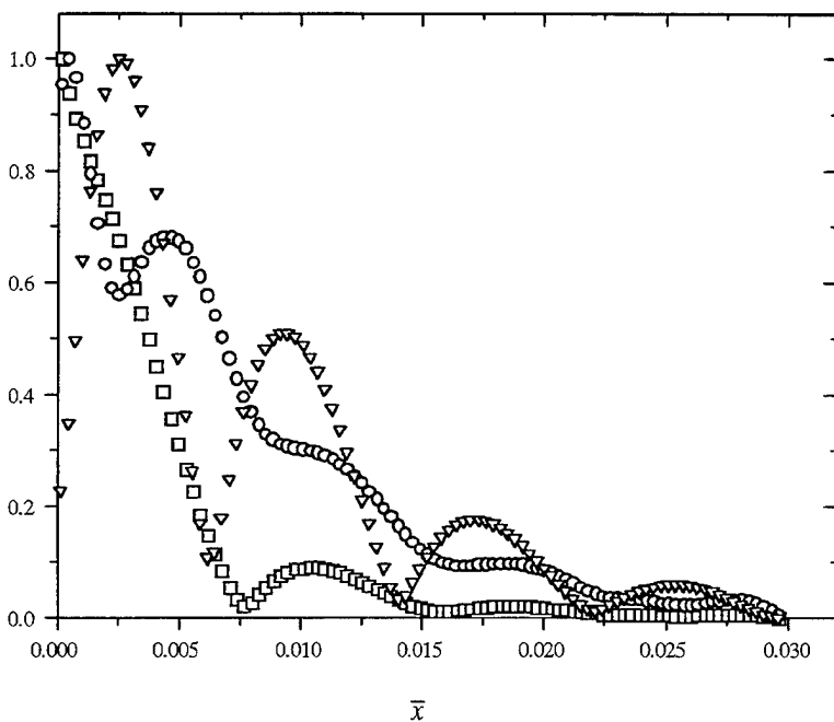
Figure 5.11. Normalized Amplitudes for the eigenfunctions \hat{n}_e ( \square ), d\hat{\Gamma}_e/dx ( \circ ), \hat{\Gamma}_e ( \nabla ). The maximum values of the amplitudes are 2.16 \times 10^{-7} , 1.57 \times 10^{-2} , and 2.54 \times 10^{-5} , respectively.
