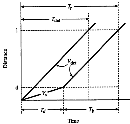
Figure 5. Schematic of a space-time plot of shock initiation of acceptor charges, l cm long.
