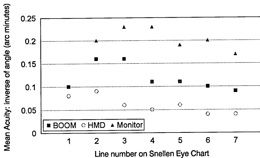
Figure 8. Virtual acuity for three display devices.
