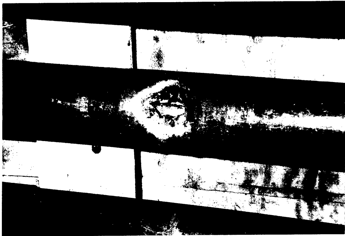
Fig. 6 - Pipe mockup rupture in 114mm (4.5 in.) diameter pipe
