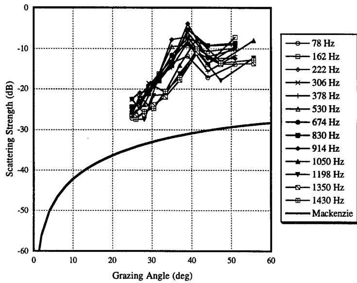
151 — Bottom scattering strengths for CST-8 Run B18 beams 7-9
