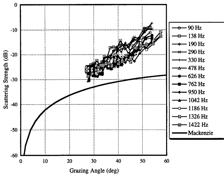
Fig. 51 — Bottom scattering strengths for CST-4 Run 7 beams 7-9
