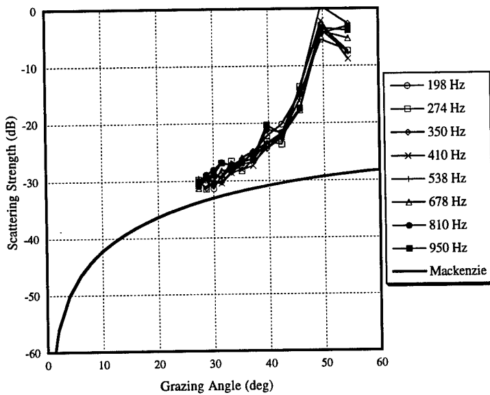
Fig. 29 — Bottom scattering strengths for CST-2 Run 43 Mod 1 beams 7-9
