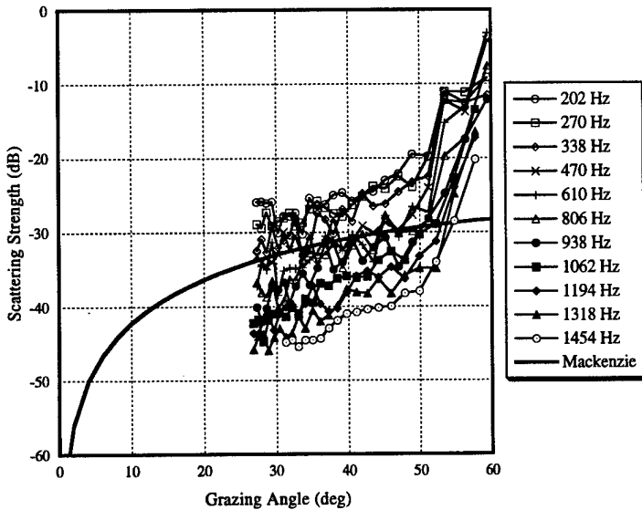
Fig. 35 — Bottom scattering strengths for CST-3 Run 2B beams 7-9
