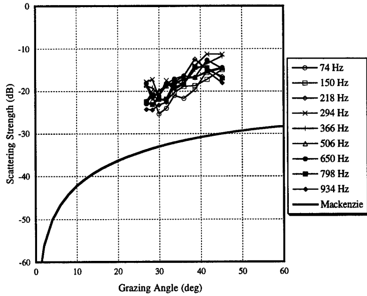
Fig. 88 — Bottom scattering strengths for CST-5 Run 46 beam 13
