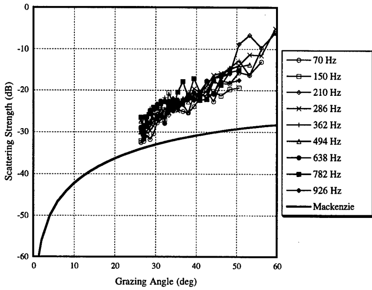
Fig. 72 — Bottom scattering strengths for CST-4 Run 59 beam 13
