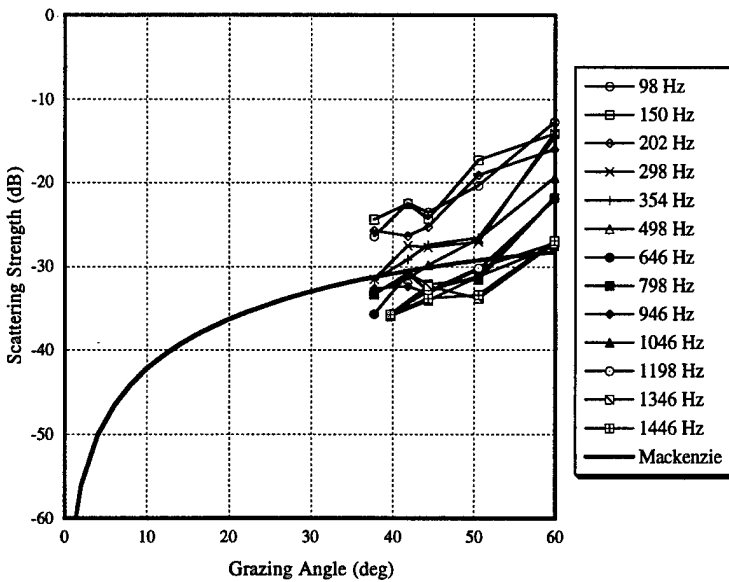
Fig. 83 — Bottom scattering strengths for CST-5 Run T1-3 beams 7-9
