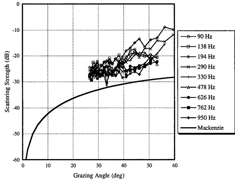
Fig. 52 — Bottom scattering strengths for CST-4 Run 7 beam 13
