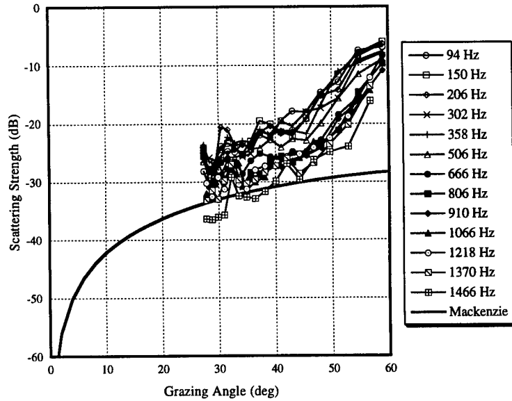
Fig. 79 — Bottom scattering strengths for CST-5 Run 26 beams 7-9
