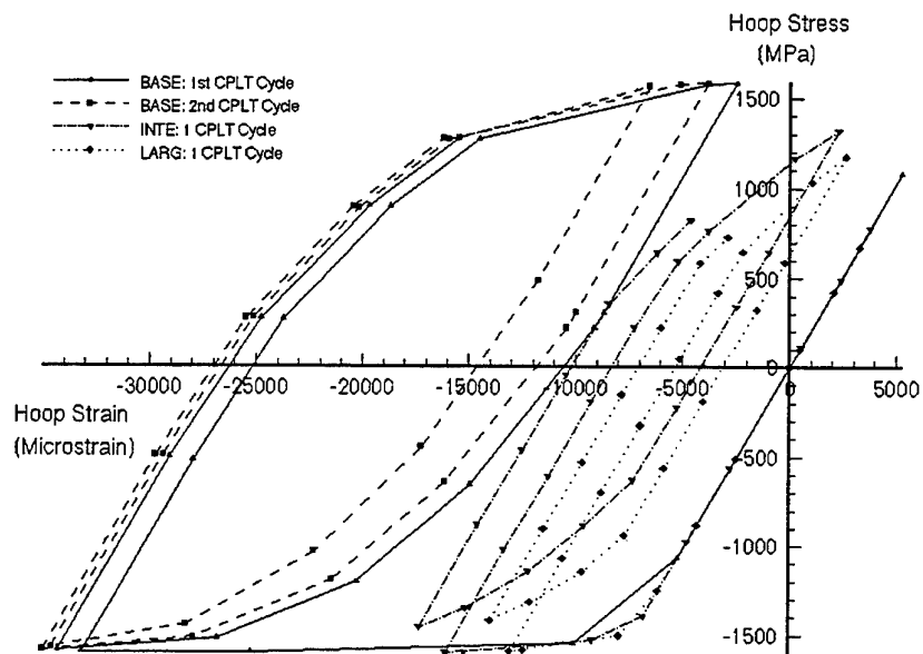
Figure 39: Comparison between Wing Test 3 results and FE results for Large Analysis: Residual after 1 CPLT cycle.
