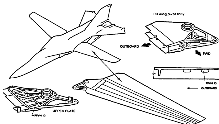
Figure 1: Location of FFWH#13 in the F-111 Aircraft.
