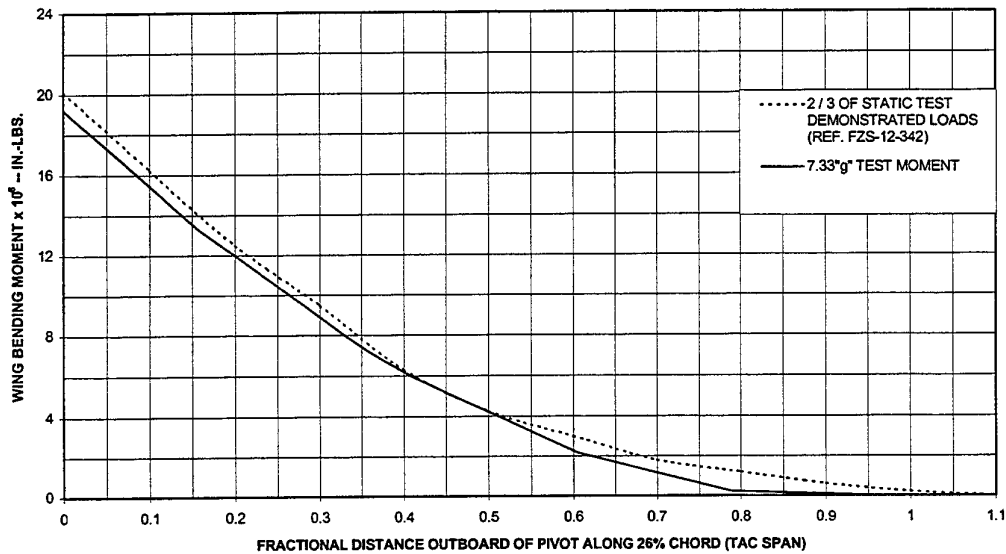
Figure 21: CPLT Wing Root Bending Moment: 1 st +7.33g Load Case.
