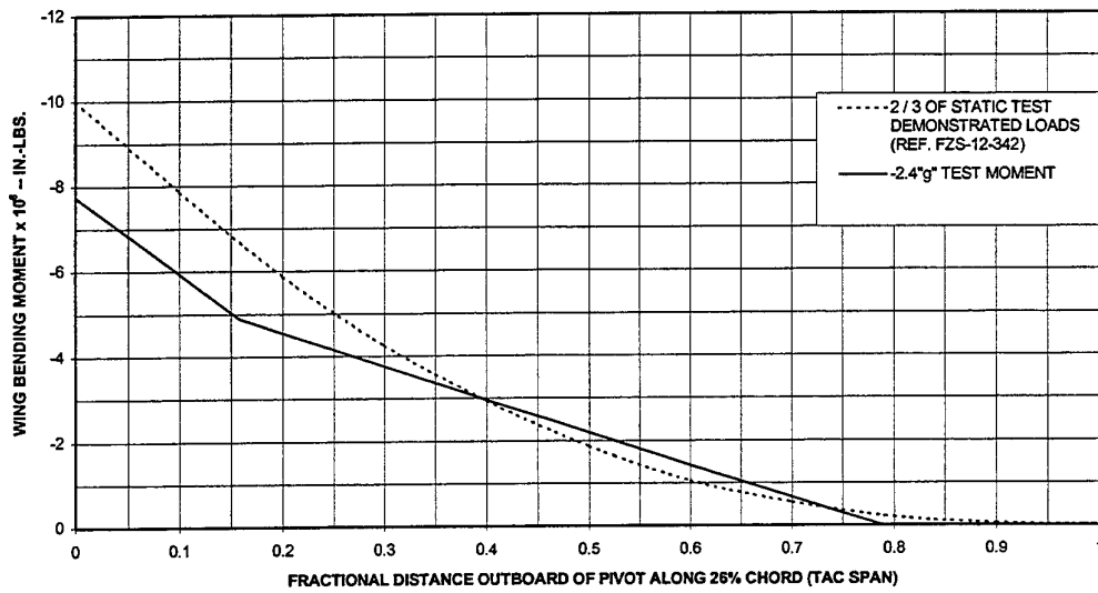
Figure 20: CPLT Wing Root Bending Moment: -2.4g Load Case.
