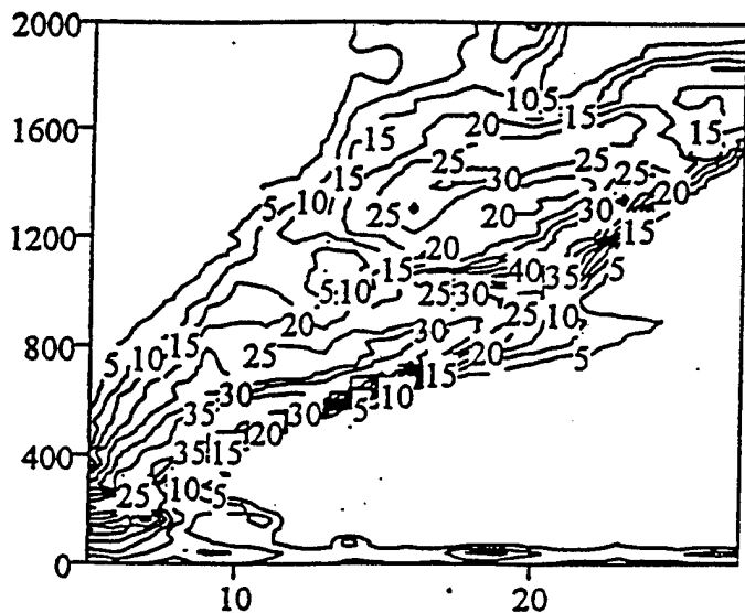
(b) A wide sweep backscatter sounder ionogram is plotted as db contours of clutter-to-noise ratio in virtual range (mi) - frequency (MHz) space.
