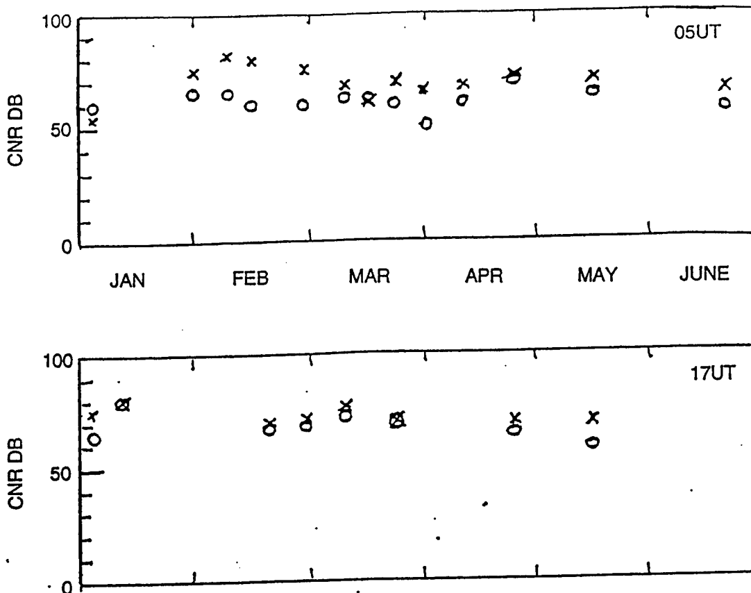
Figure 7. Selected CNR values are plotted over the seasons for 05 UT and 17 UT. The ROTHR levels are given as O points and were limited to examples where radar frequency selection was appropriate for the range. The corresponding RADARC value is marked as an X
