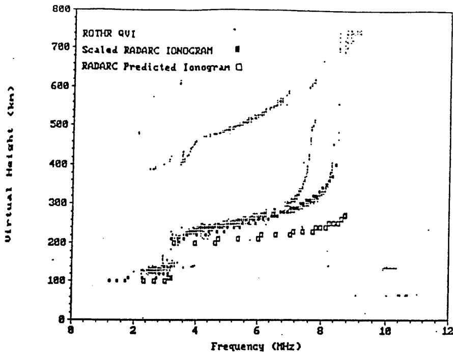
(a) The quasi-vertical sounding is shown for: ROTHR as dots; RADARC's median predicted ionogram as open box points; and the RADARC prediction after critical frequency and height correction as solid boxes.
