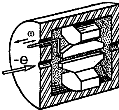
Fig 3.2a Resonant coupler with transverse electric field in the interaction region .
