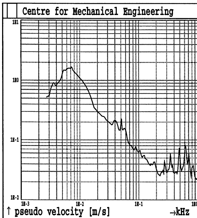
Fig.1B100. Shot 1 MAXIMAX Sensor A20
