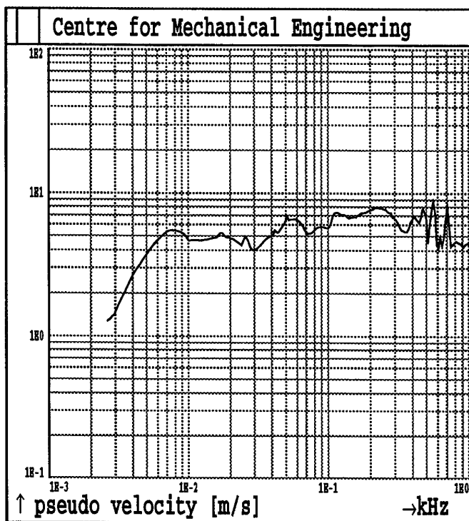
Fig.2B83. Shot 2 MAXIMAX Sensor A3
