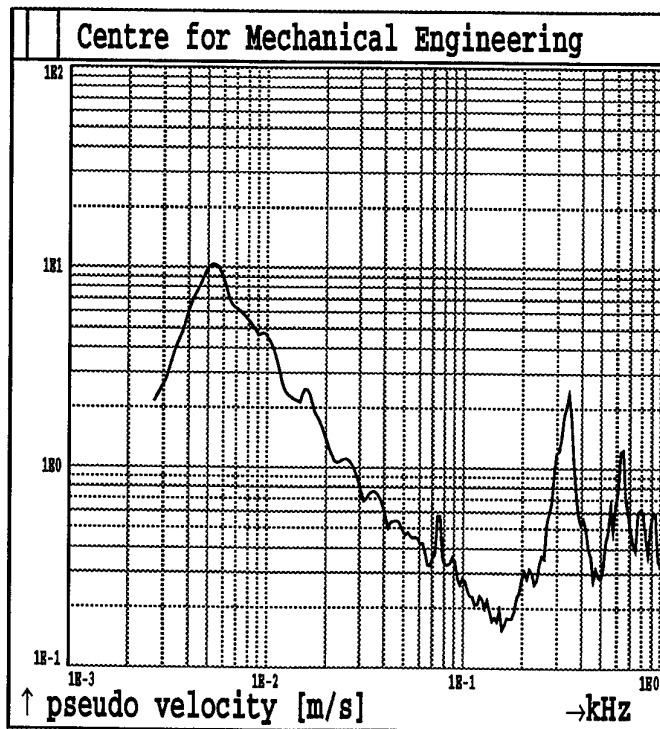
Fig.2B102. Shot 2 MAXIMAX Sensor A22
