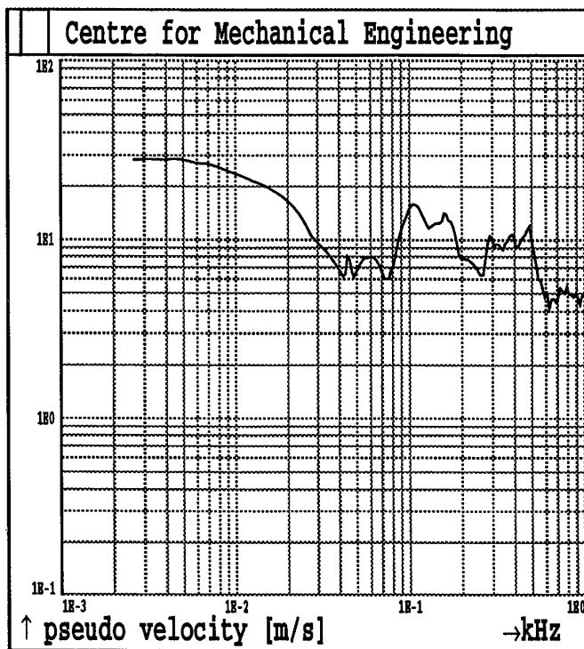
Fig.2B87. Shot 2 MAXIMAX Sensor A7
