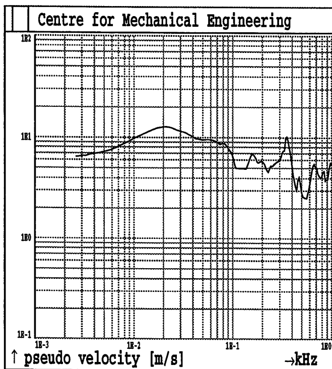
Fig.2B91. Shot 2 MAXIMAX Sensor A11
