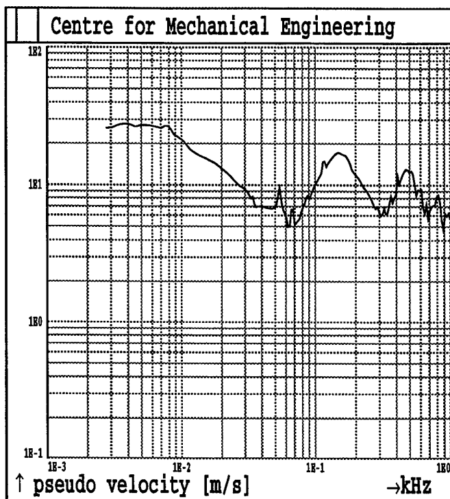
Fig.3B87. Shot 3 MAXIMAX Sensor A7
