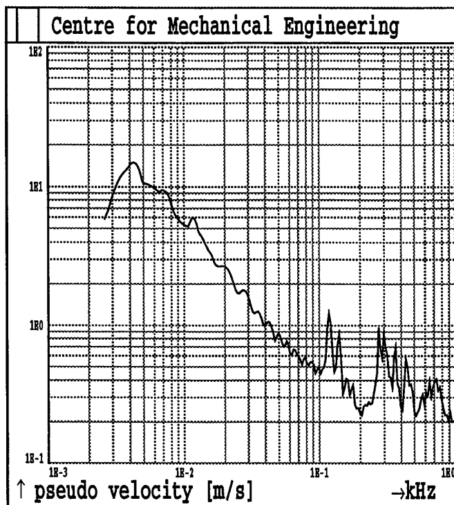
Fig.3B103. Shot 3 MAXIMAX Sensor A24
