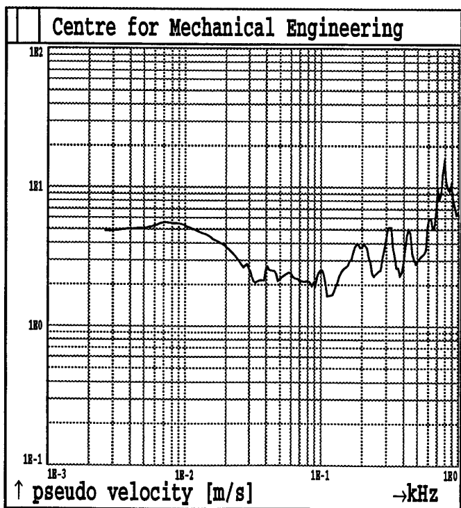
Fig.2B86. Shot 2 MAXIMAX Sensor A6
