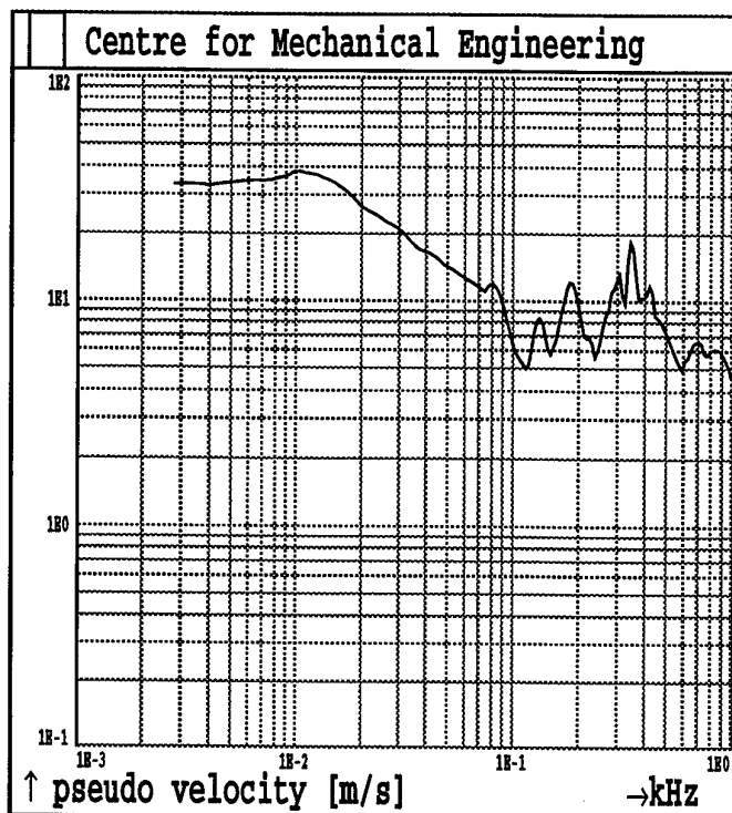
Fig.3B81. Shot 3 MAXIMAX Sensor A1
