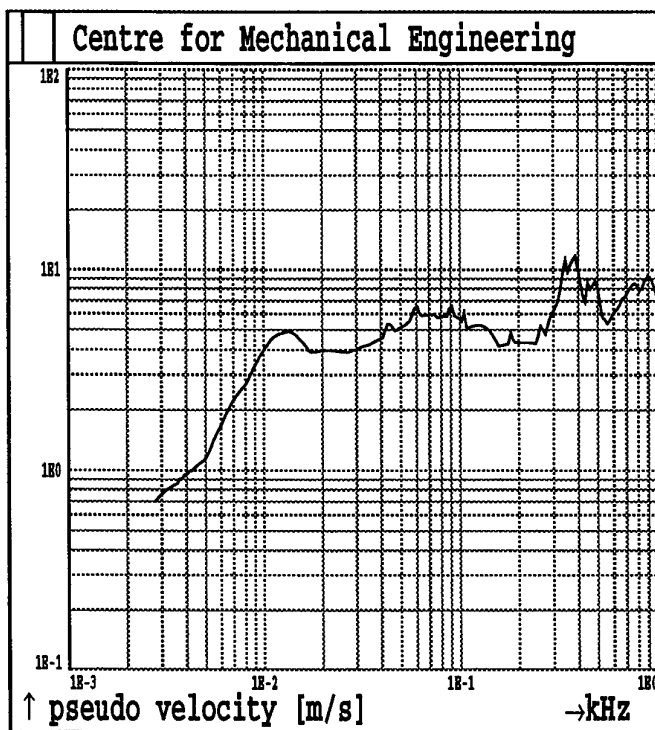
Fig.1B93. Shot 1 MAXIMAX Sensor A13
