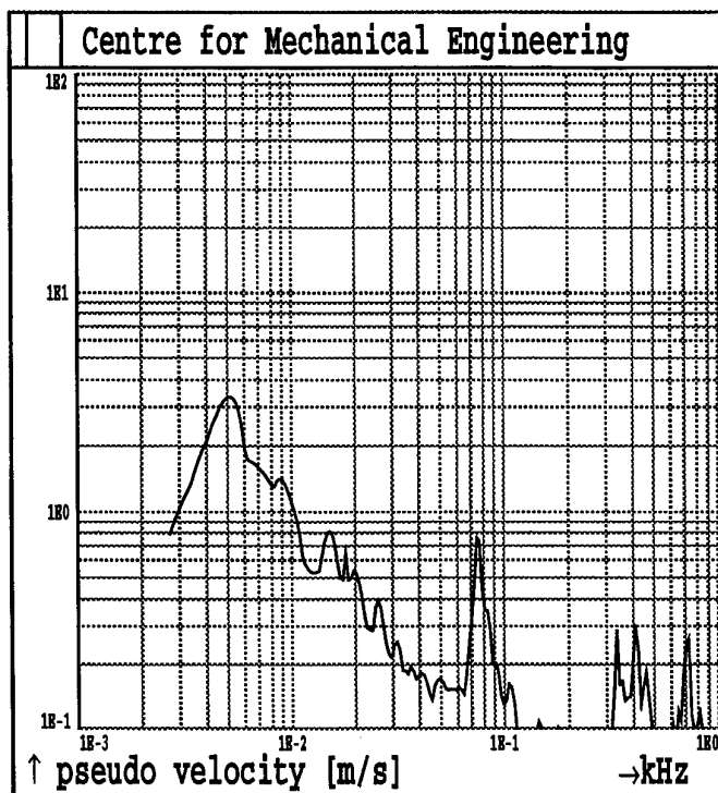
Fig.2B99. Shot 2 MAXIMAX Sensor A19
