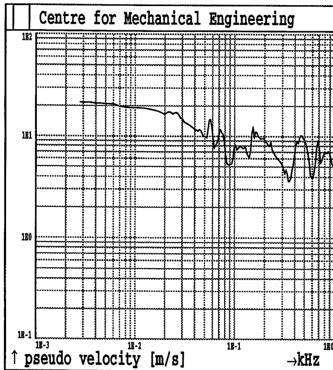
Fig.1B87. Shot 1 MAXIMAX Sensor A7
