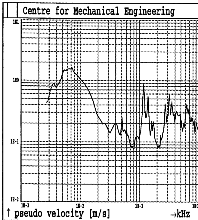
Fig.1B103. Shot 1 MAXIMAX Sensor A23
