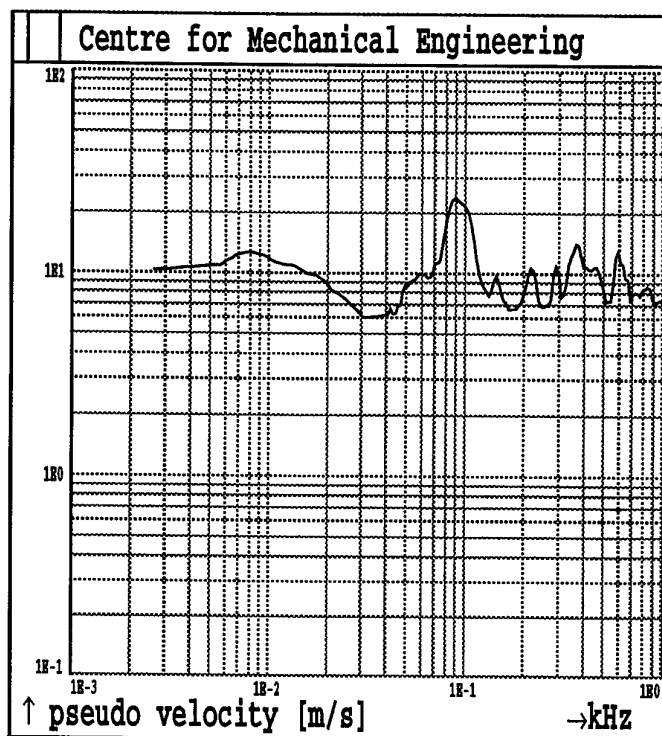
Fig.2B89. Shot 2 MAXIMAX Sensor A9
