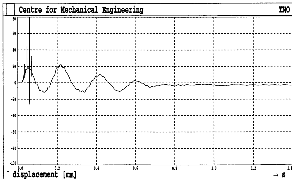
Fig.2B2. Shot 2 Sensor R2
