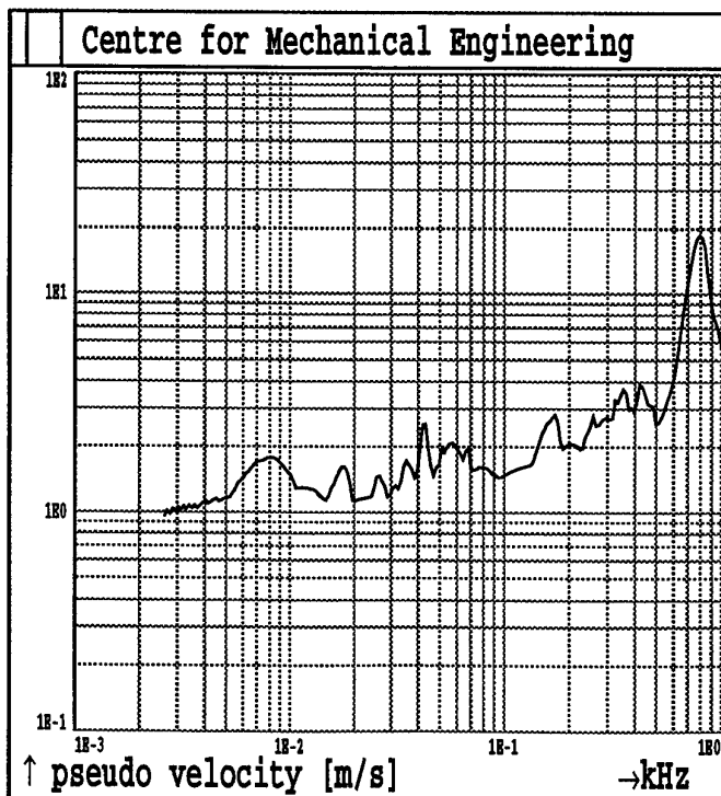
Fig.2B94. Shot 2 MAXIMAX Sensor A14
