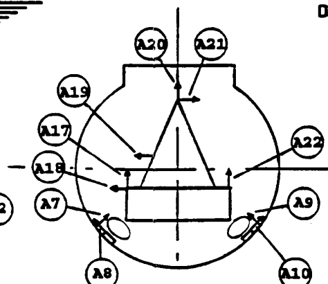
SECTION A-A Accelerometers
