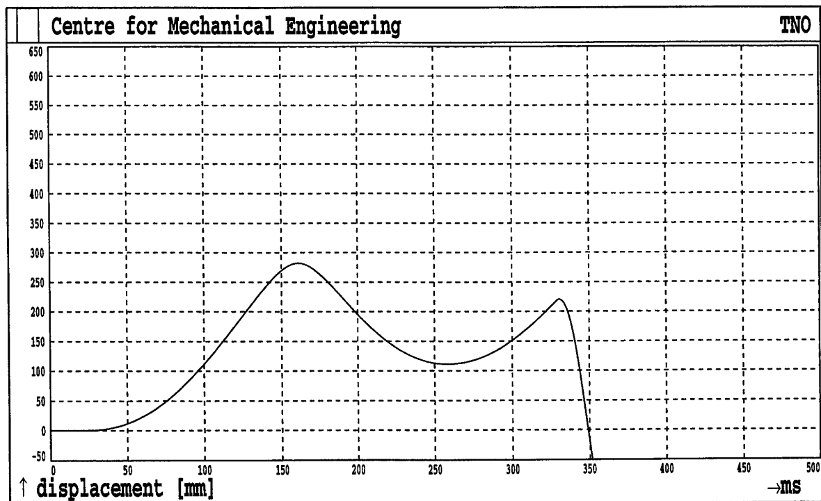
Fig.3B80. Shot 3 Sensor A24
