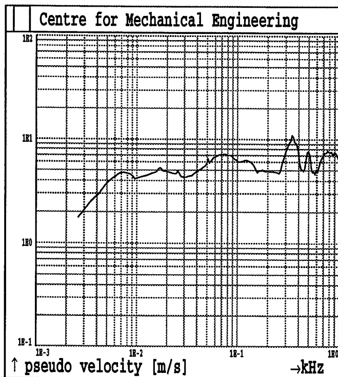
Fig.2B93. Shot 2 MAXIMAX Sensor A13
