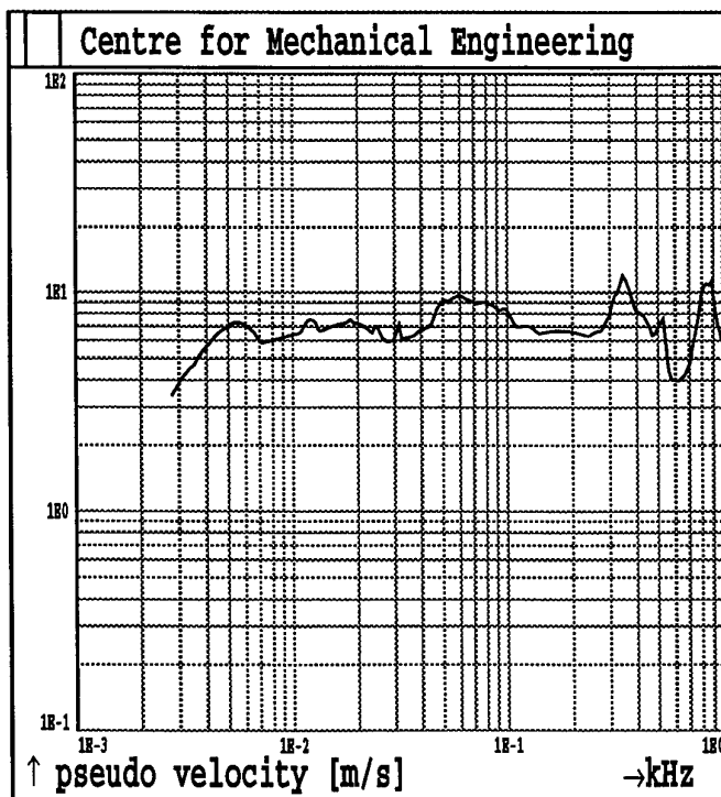
Fig.3B92. Shot 3 MAXIMAX Sensor A13
