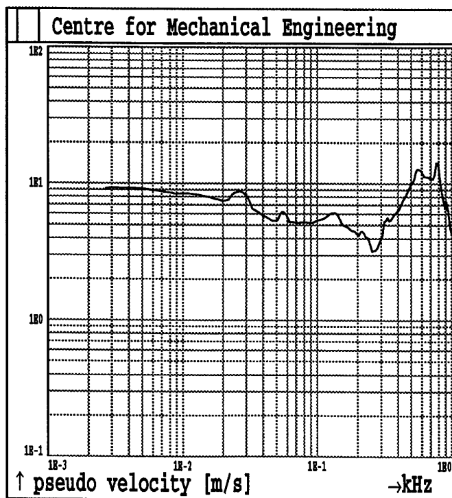
Fig.2B92. Shot 2 MAXIMAX Sensor A12
