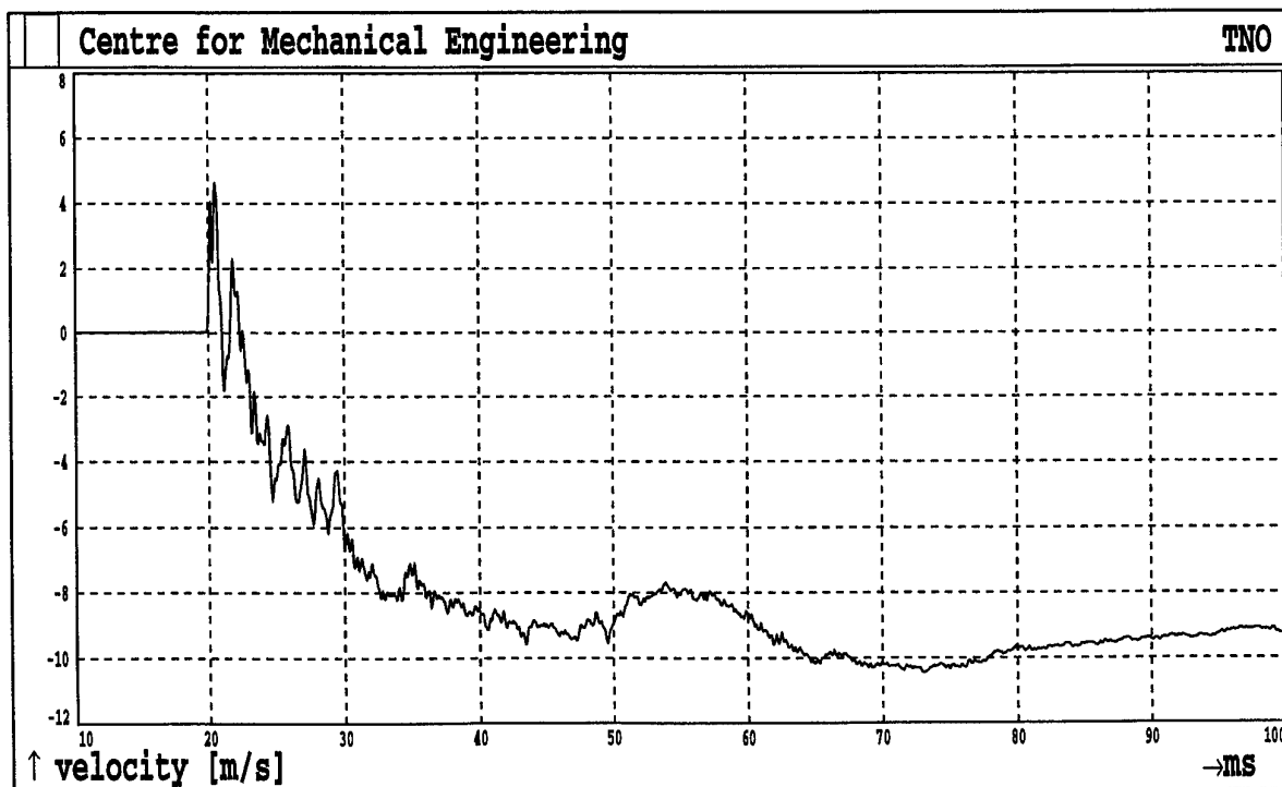
Fig.2B44. Shot 2 Sensor A12
