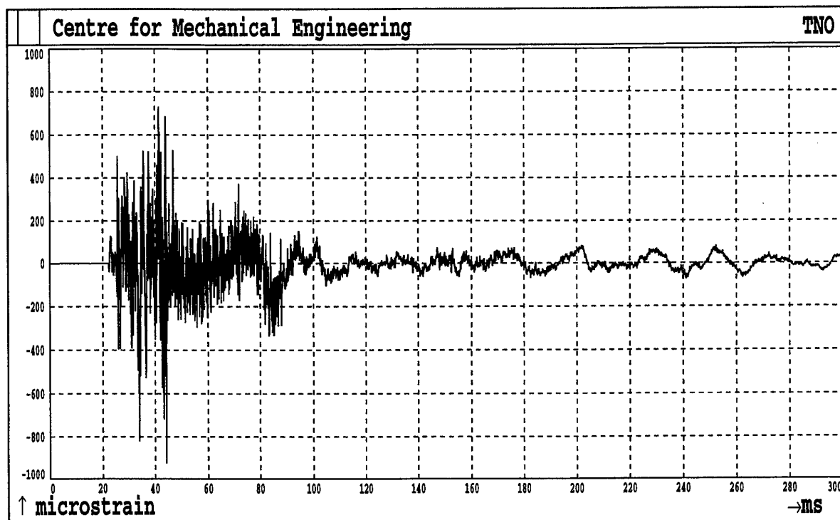
Fig.1A23. Shot 1 Sensor S24
