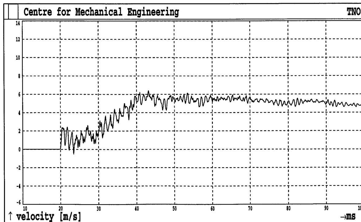
Fig.2B38. Shot 2 Sensor A6
