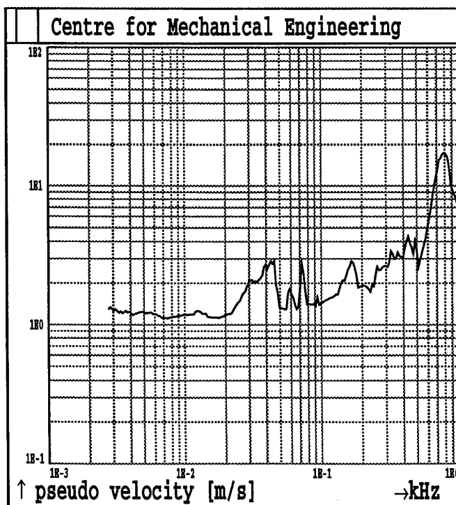
Fig.1B94. Shot 1 MAXIMAX Sensor A14
