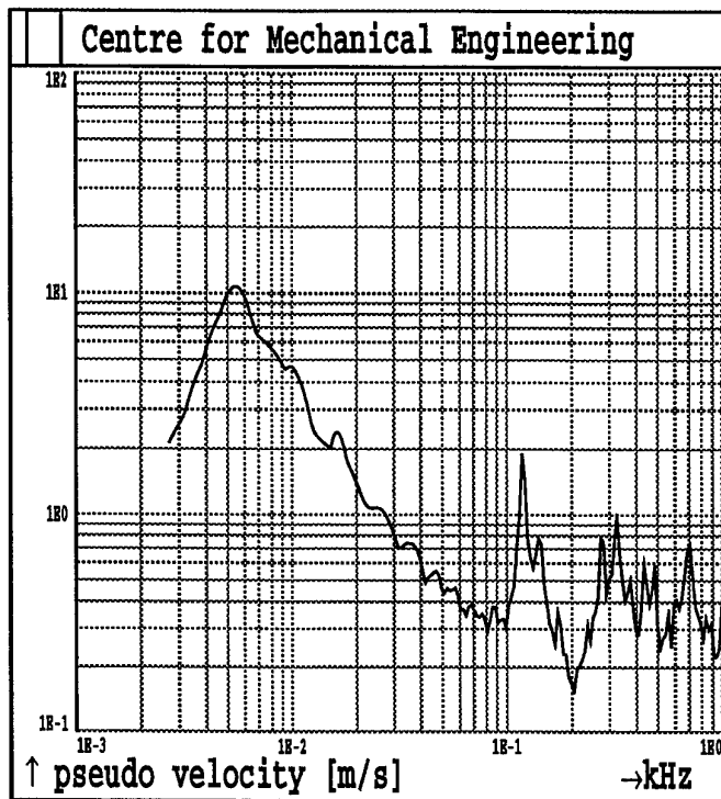
Fig.2B103. Shot 2 MAXIMAX Sensor A23
