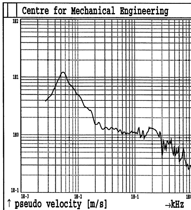
Fig.2B104. Shot 2 MAXIMAX Sensor A24
