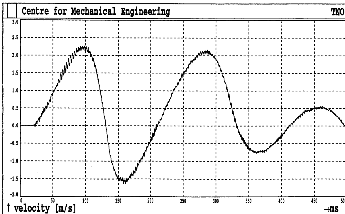
Fig.2B54. Shot 2 Sensor A22
