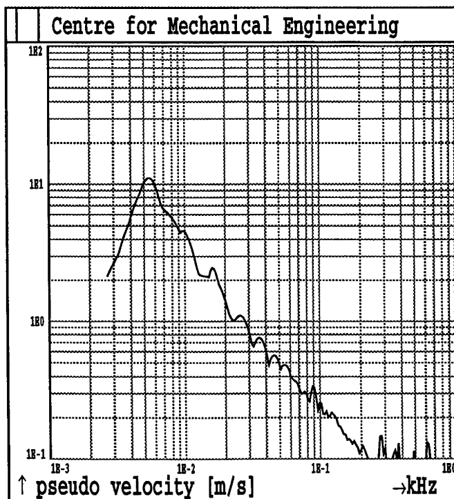
Fig.2B100. Shot 2 MAXIMAX Sensor A20
