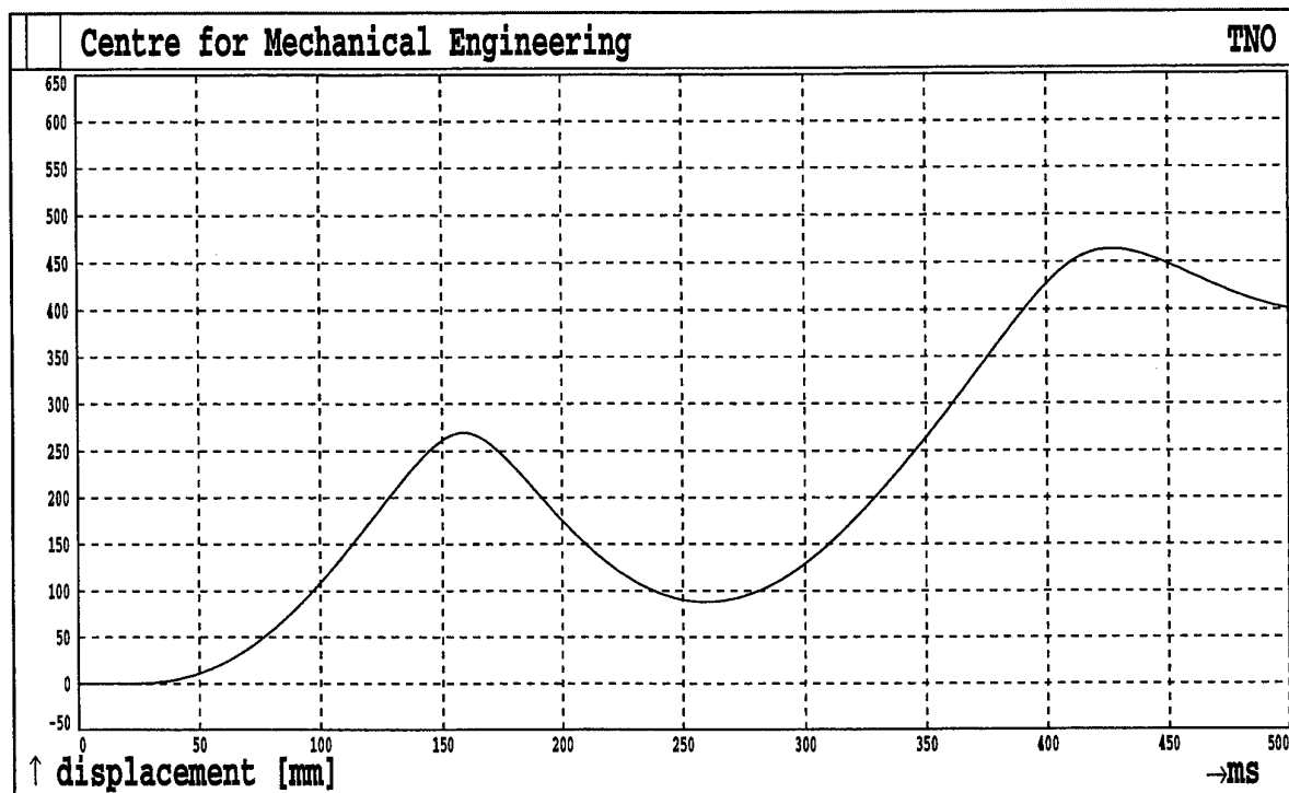
Fig.3B79. Shot 3 Sensor A23
