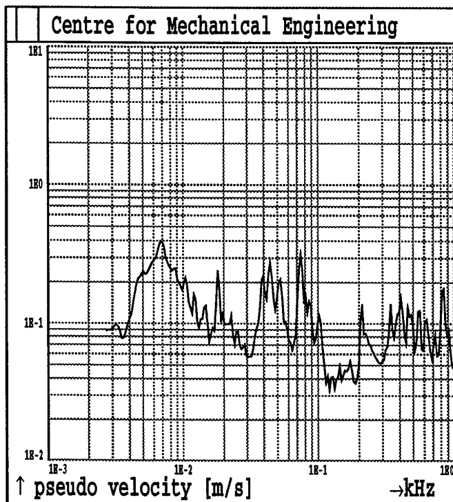
Fig.1B101. Shot 1 MAXIMAX Sensor A21
