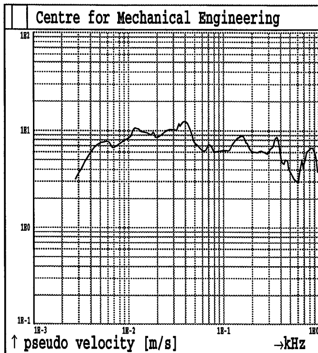
Fig.3B95. Shot 3 MAXIMAX Sensor A16
