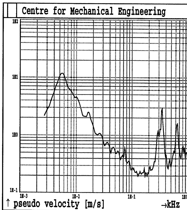
Fig.2B97. Shot 2 MAXIMAX Sensor A17
