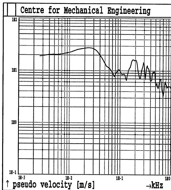
Fig.2B81. Shot 2 MAXIMAX Sensor A1
