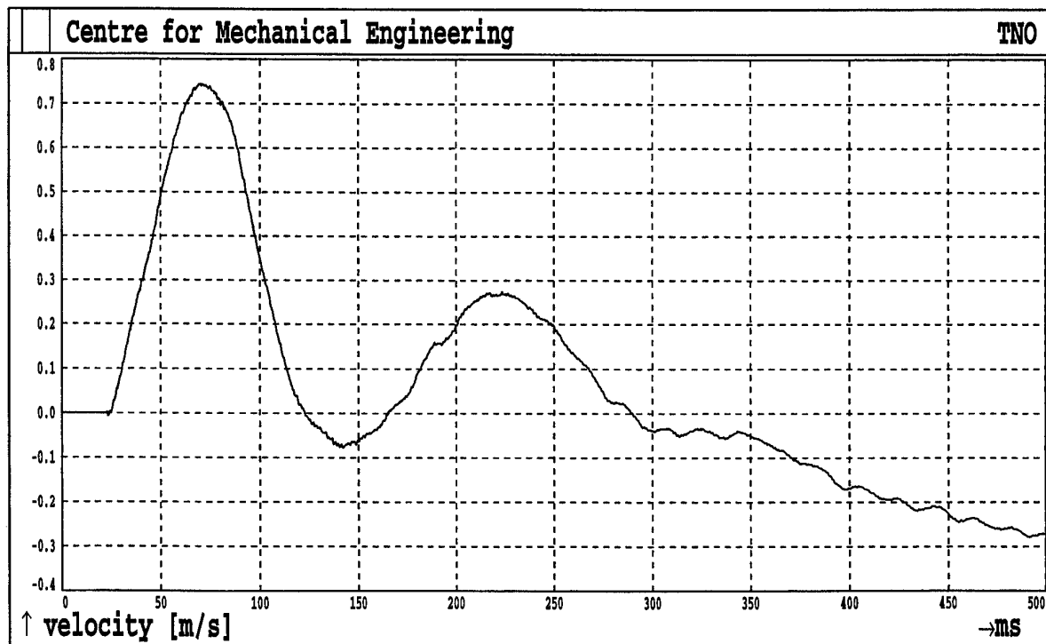
Fig.1B52. Shot 1 Sensor A20
