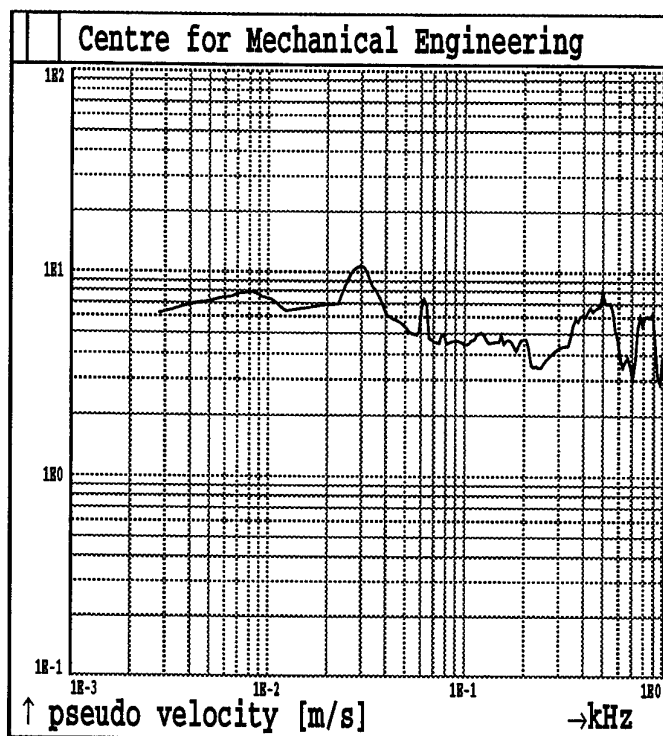
Fig.1B95. Shot 1 MAXIMAX Sensor A15
