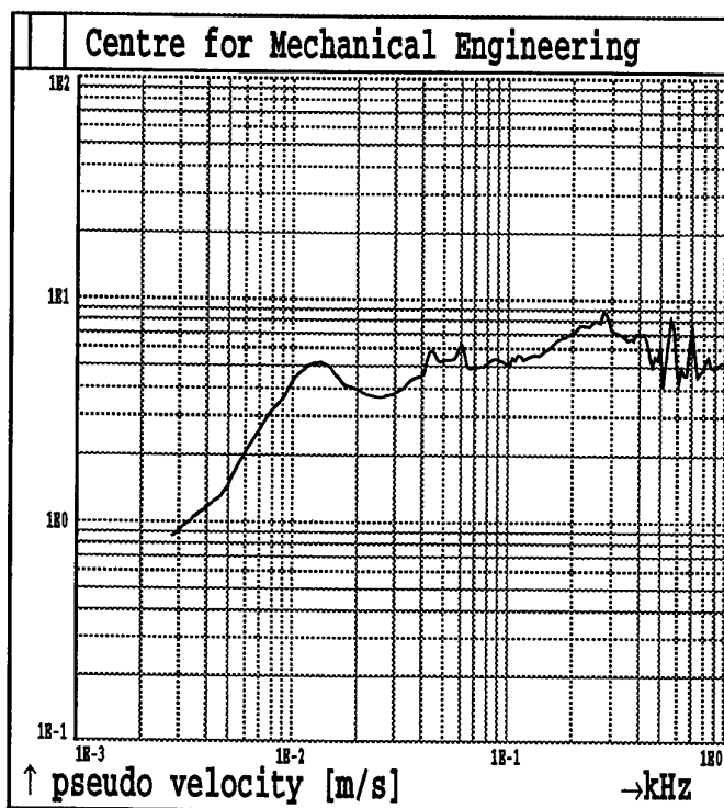
Fig.1B83. Shot 1 MAXIMAX Sensor A3
